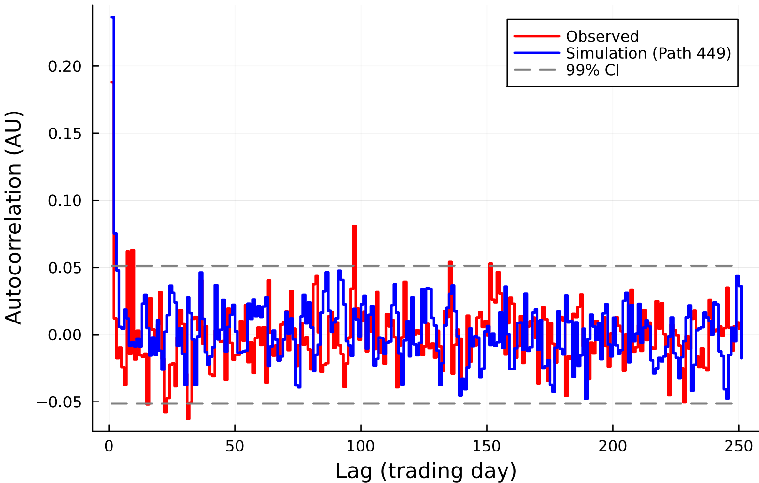
ACF of SPY Growth Rate (Non-Jump, Path 449)
