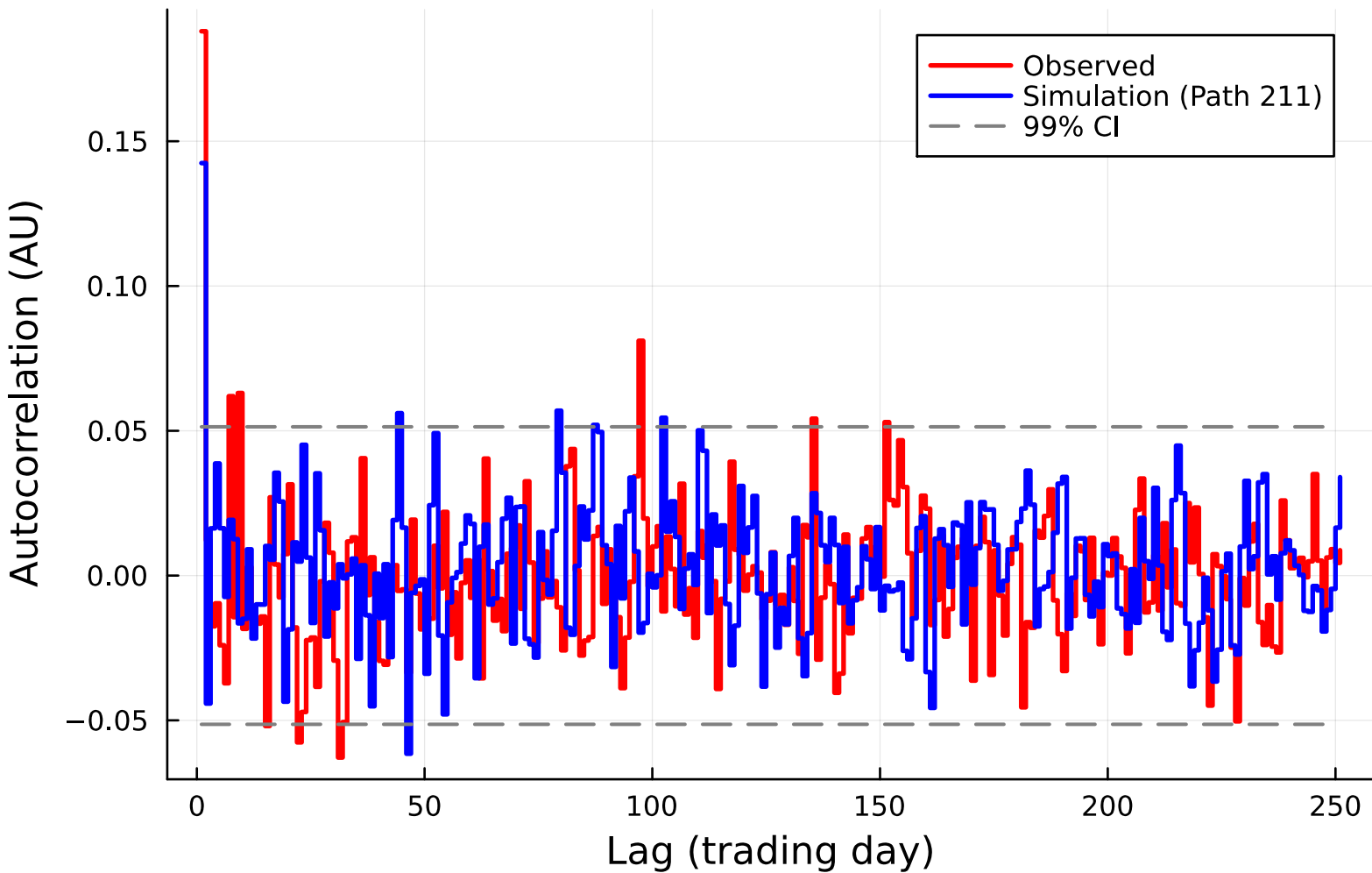
ACF of SPY Growth Rate (Jump, Path 211)
