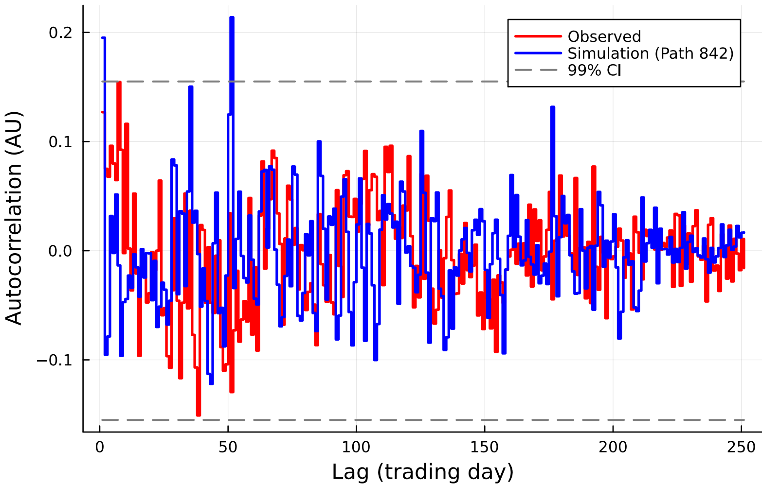
ACF of SPY |Growth Rate| (Jump, Path 842)
