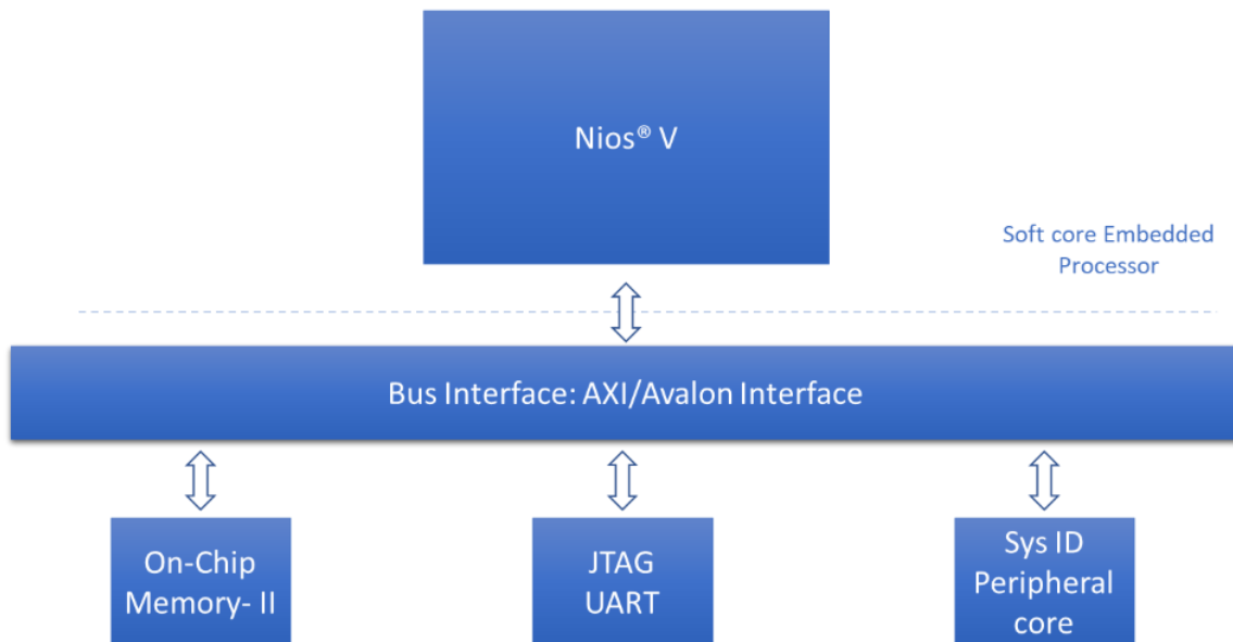
Figure 1-1. Block Diagram
