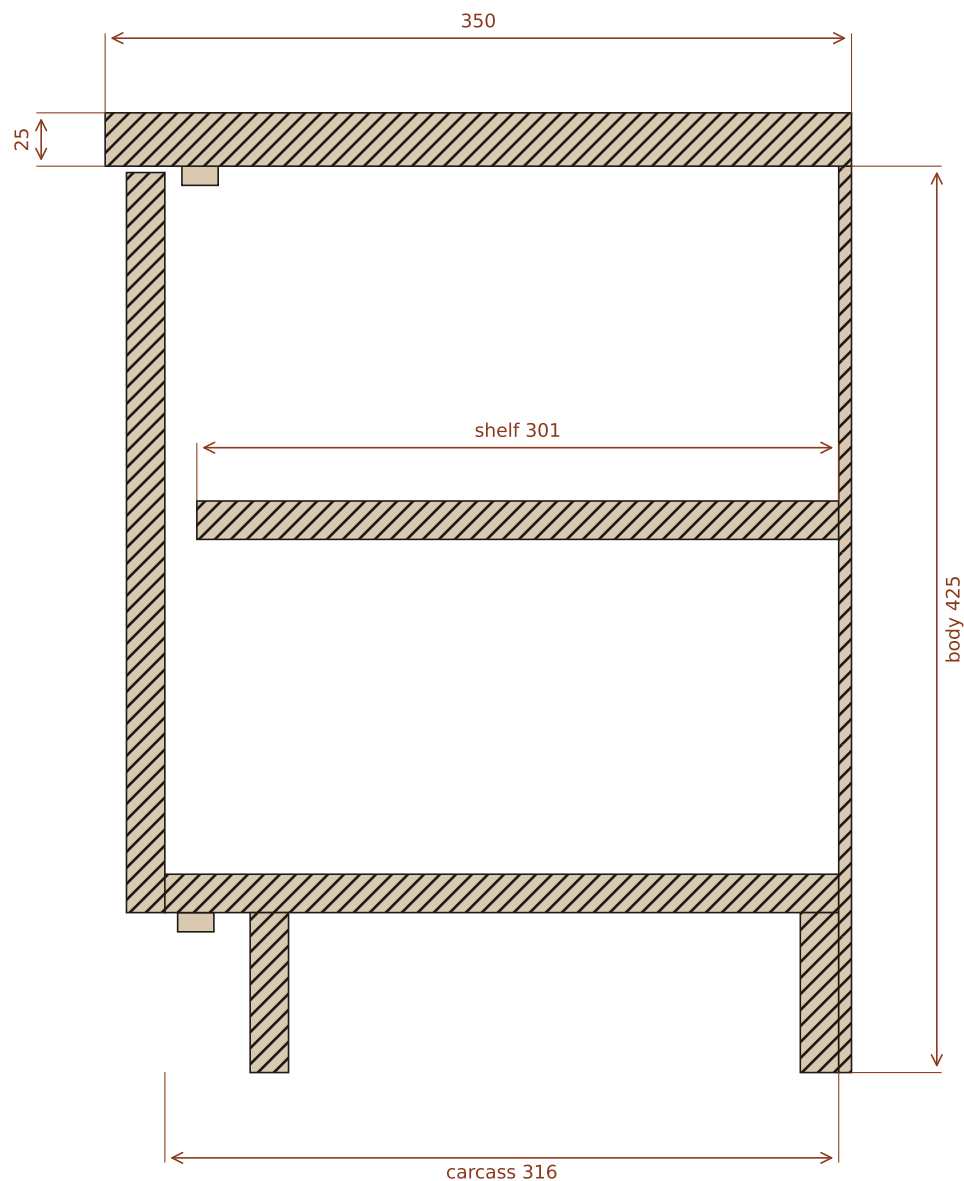
SECTION A-A at X = 224.5 mm (looking from right)
