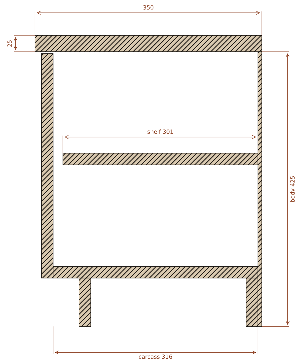
SECTION A-A at X = 229.5 mm (looking from right)
