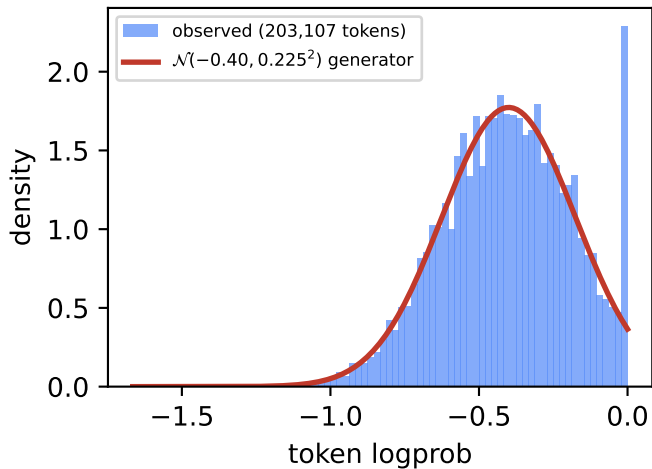
Logprobs match the synthetic generator
