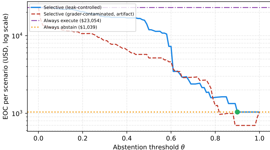
Always-abstain is the baseline a policy must beat
