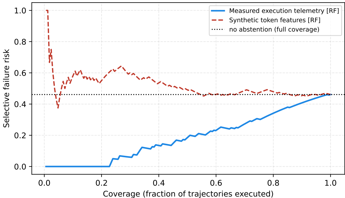
Out-of-fold risk--coverage profile
