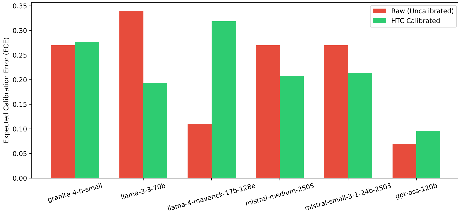
Expected Calibration Error Before & After HTC Calibration
