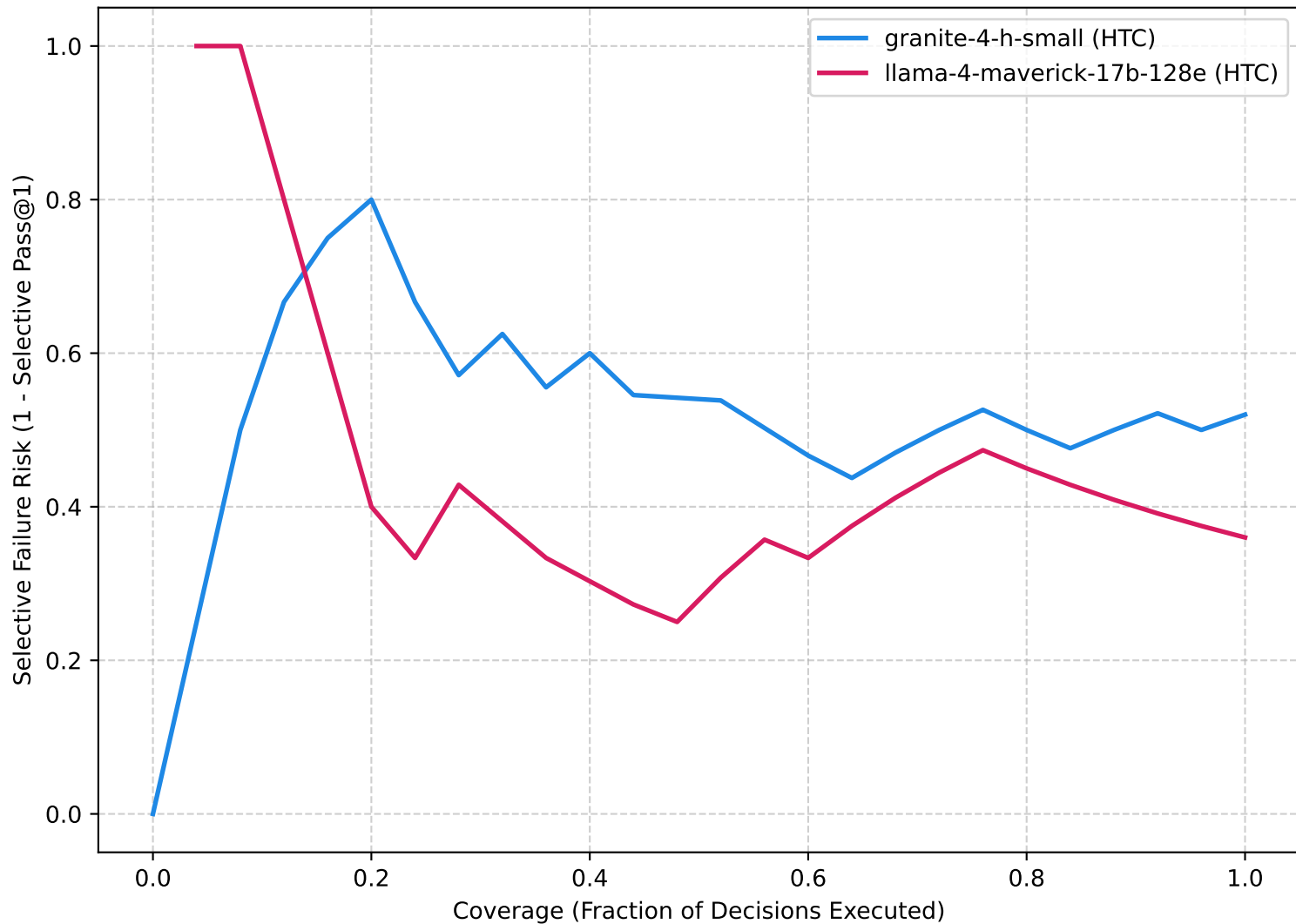
Risk-Coverage Profile (Selective Abstention)
