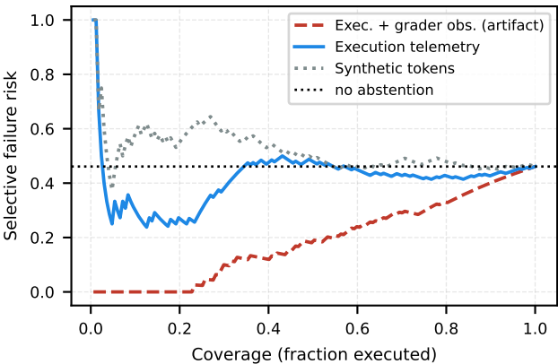
Out-of-fold risk--coverage
