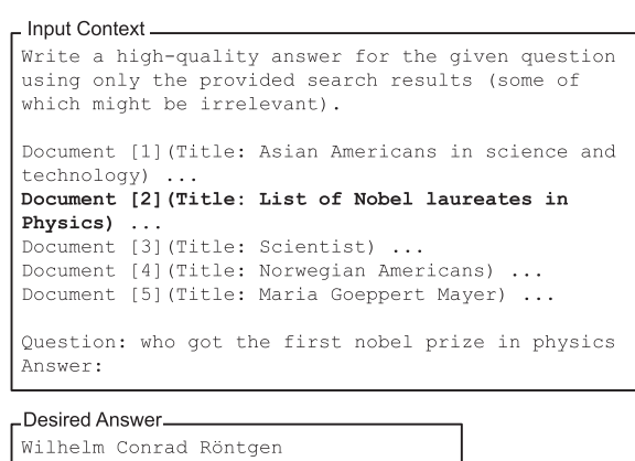
Figure 4: Modulating the input context length of the multi-document question answering example presented in Figure 2. Adding documents that do not contain the answer increases the length of the input context, but does not affect the desired output.
