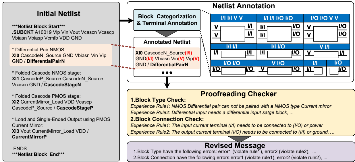
Fig. 4: Human experience-based proofreading.
