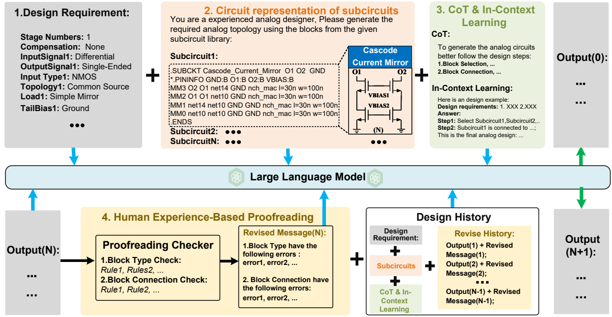
Fig. 2: Overview of AnalogXpert framework.
