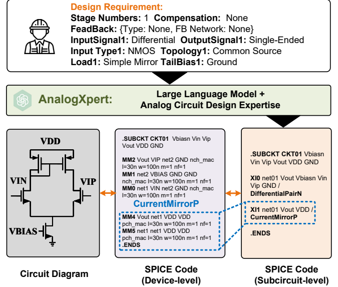
Fig. 1: AnalogXpert formulation of the topology synthesis task.
