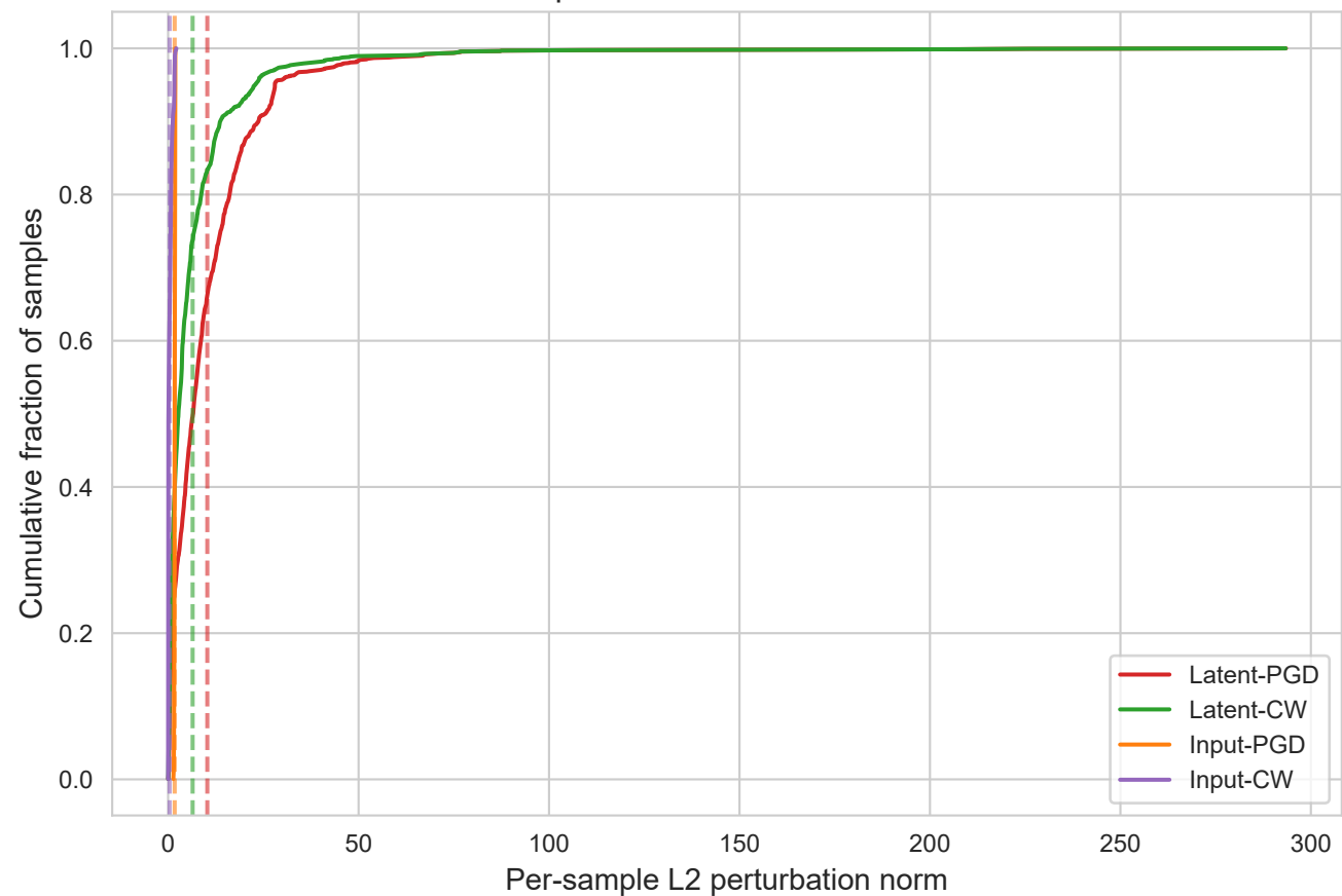
Empirical CDF of L2 Distortion
