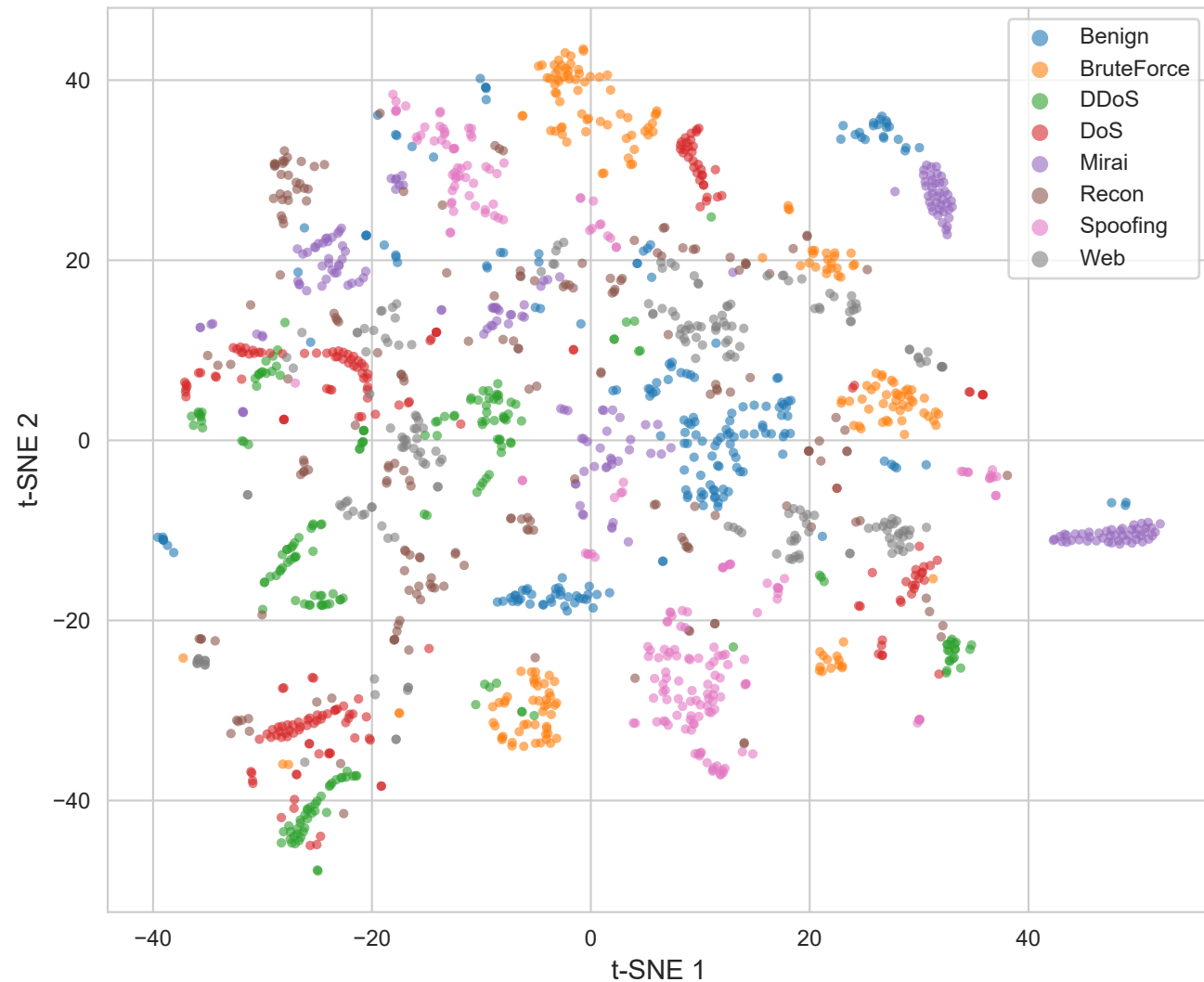
VAE Latent Space by Attack Category
