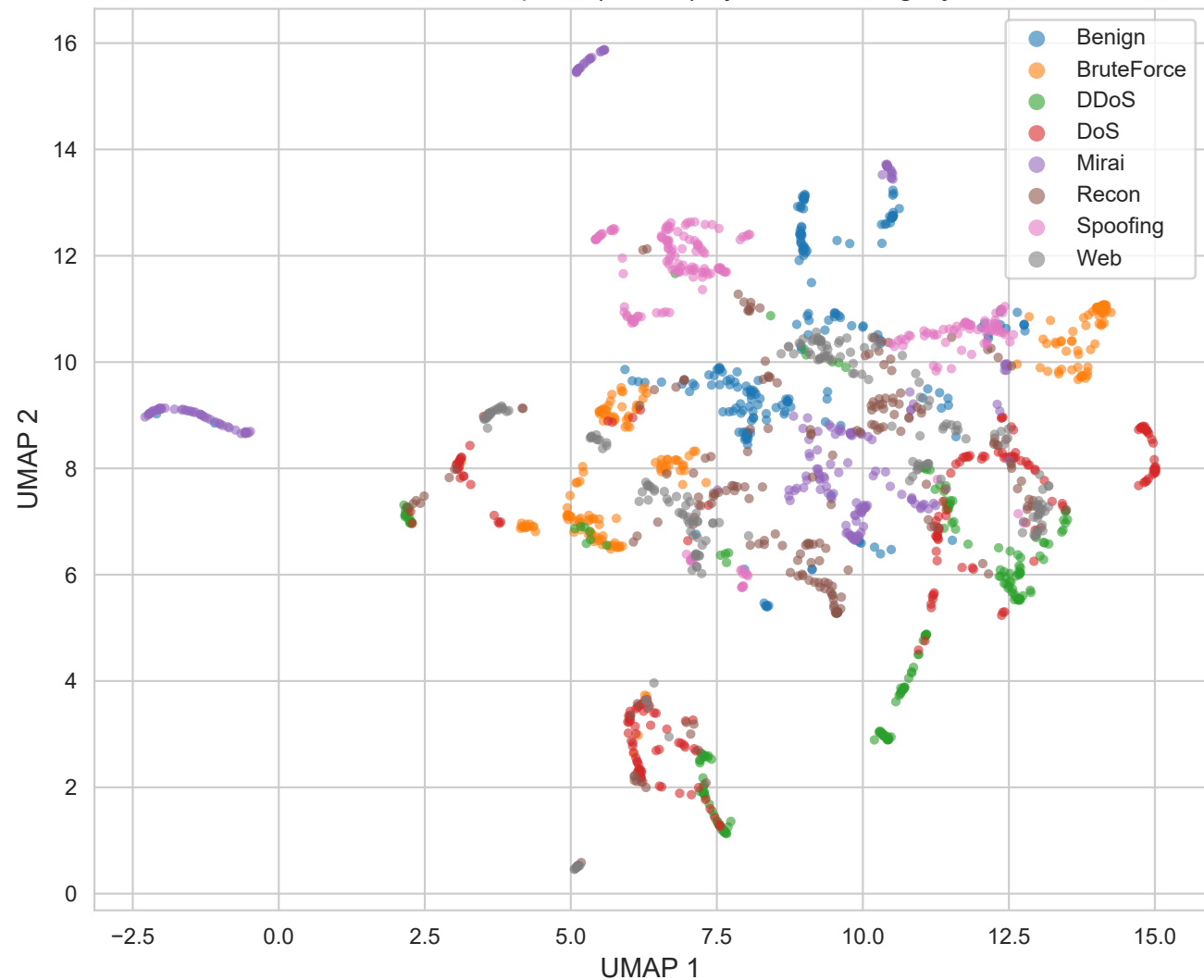
VAE Latent Space (UMAP) by Attack Category
