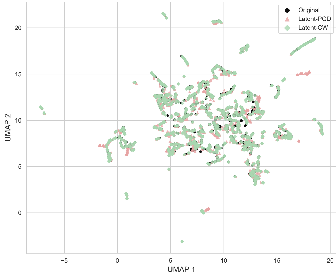
Latent Space (UMAP): Original vs Perturbed
