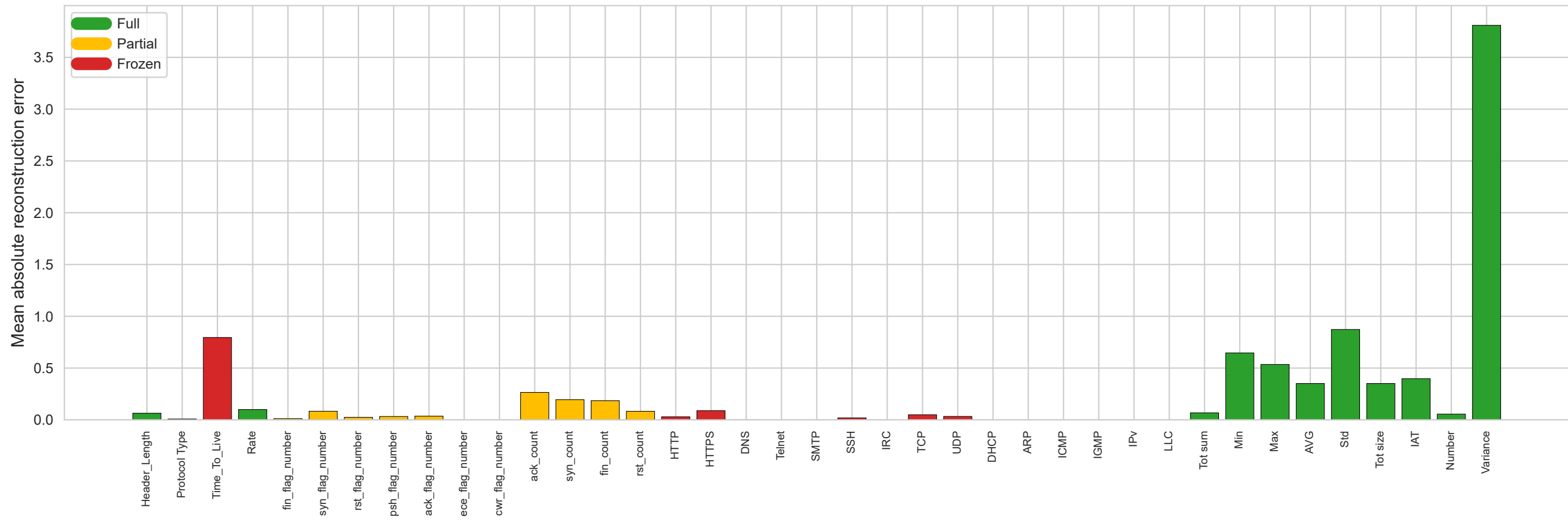
Per-Feature VAE Reconstruction MAE (color = mask type)
