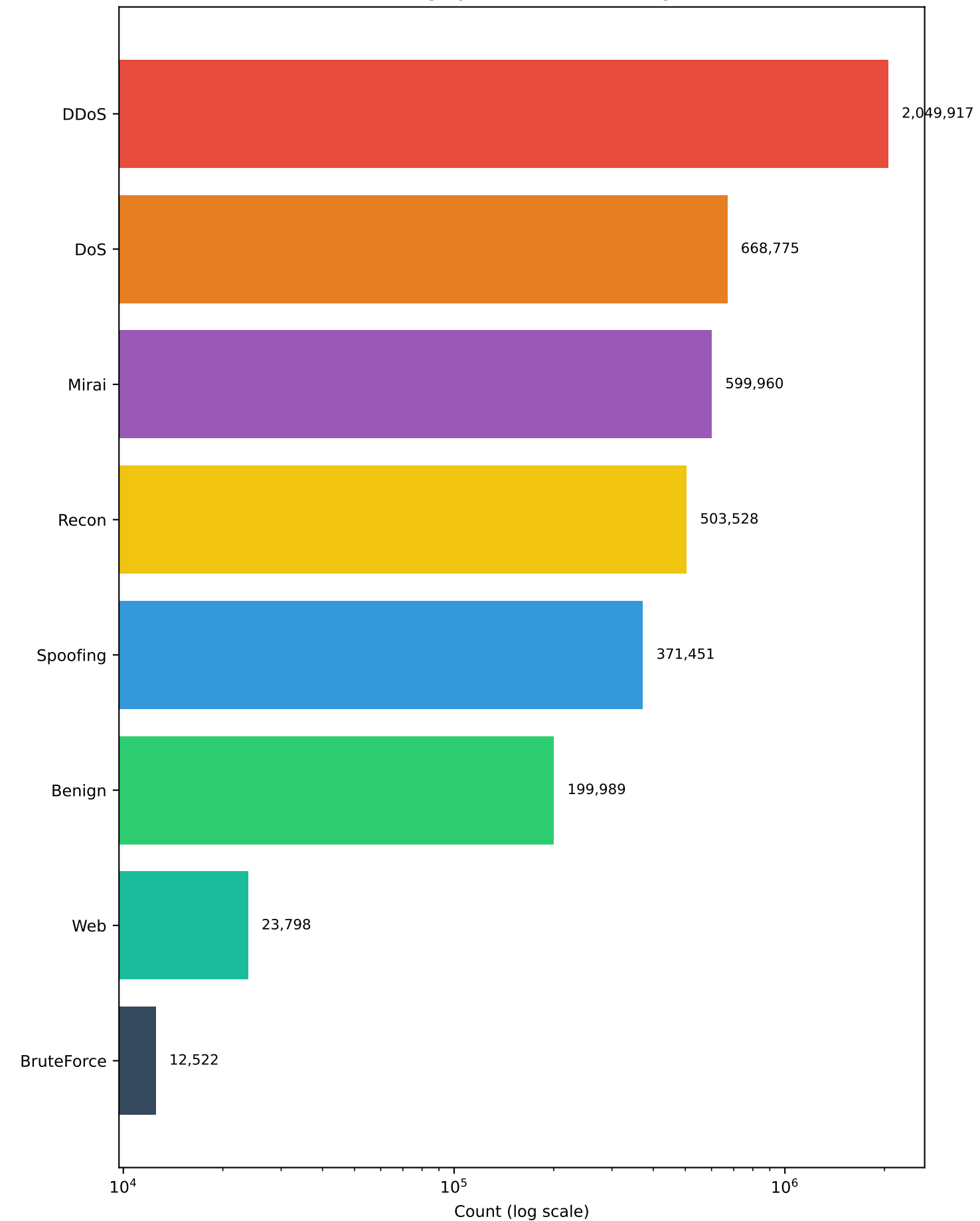
B) Per-Category Distribution (8 categories)
