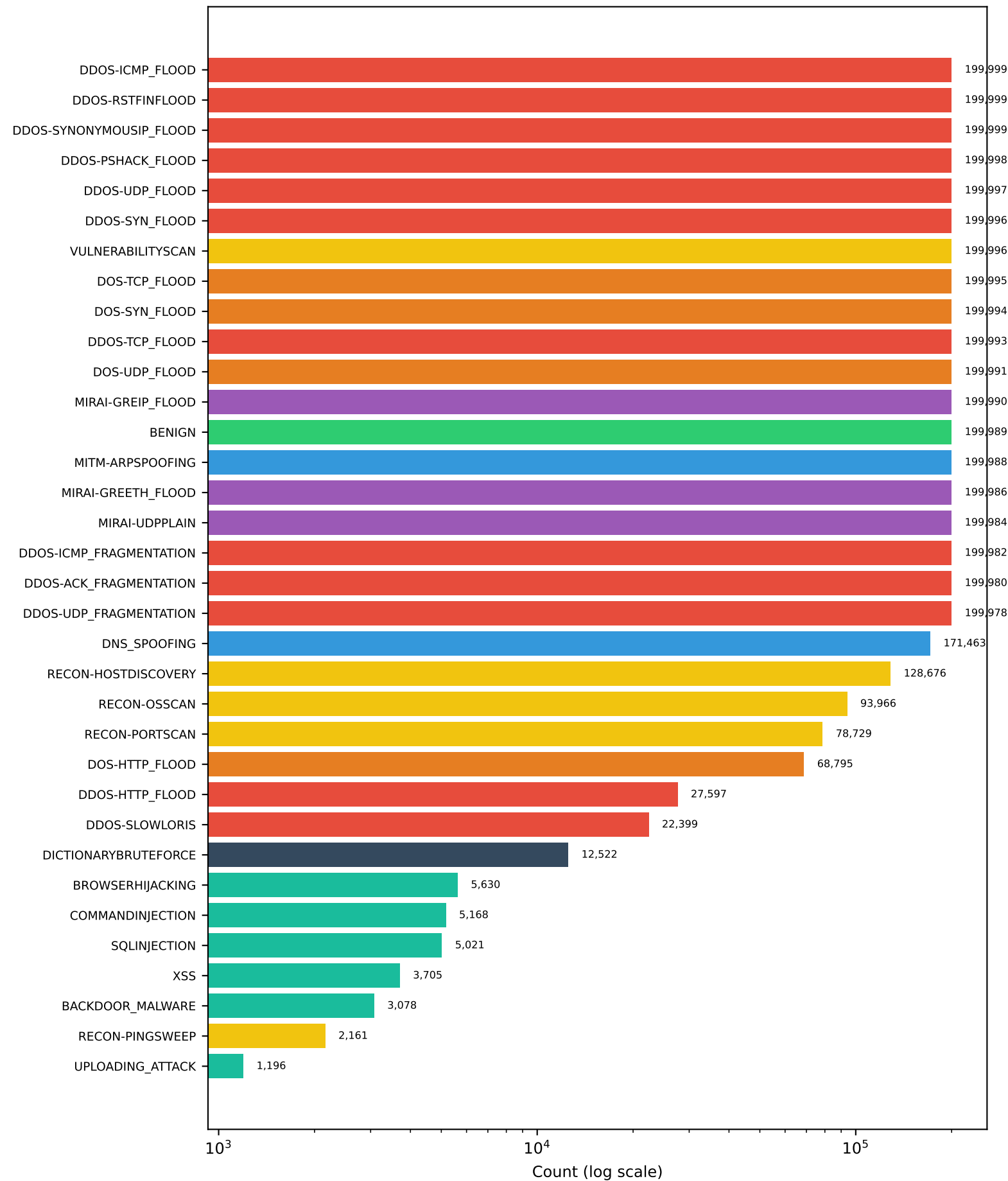
A) Per-Class Distribution (34 classes)
