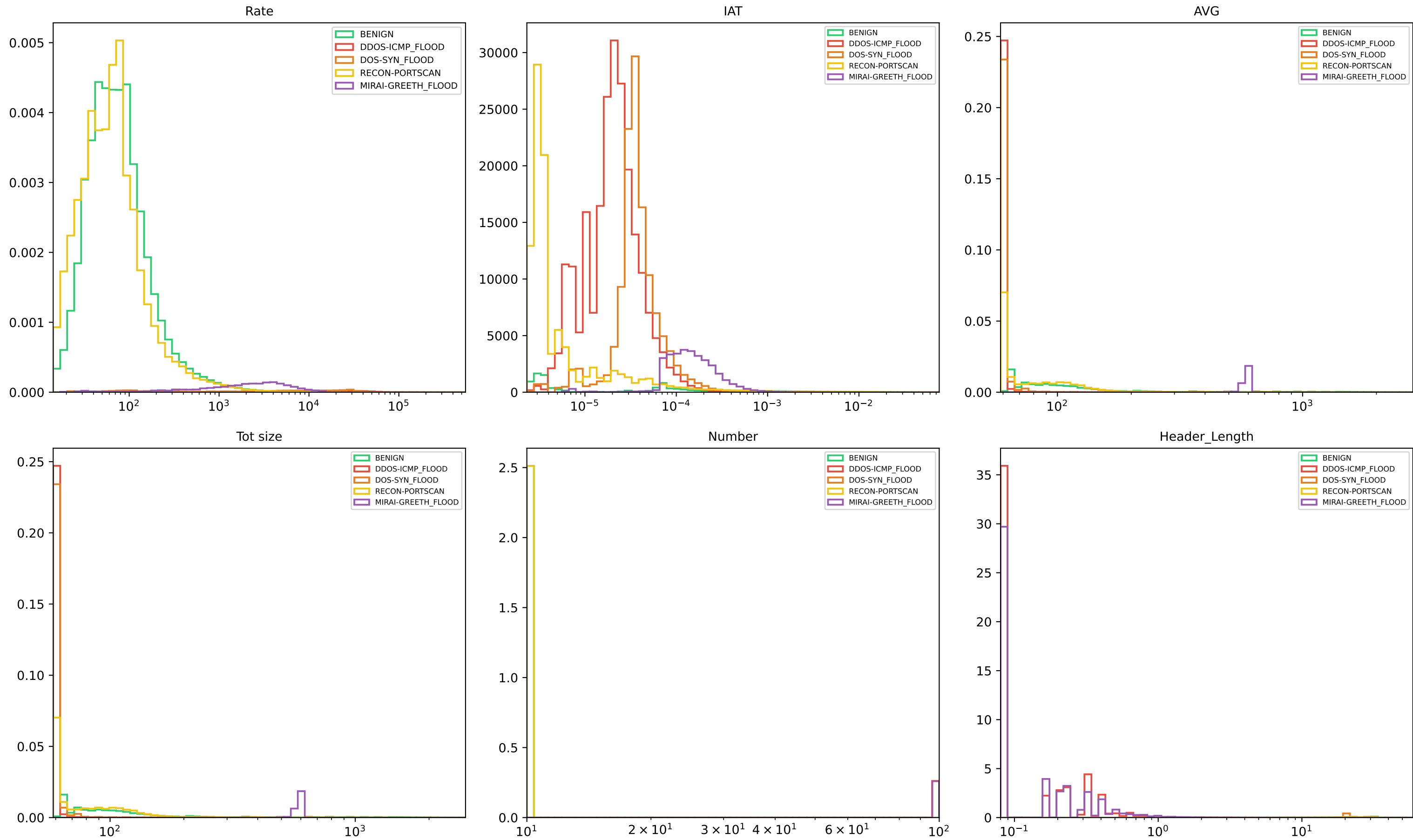
Feature Distributions (Log-binned Histograms): Benign vs Key Attack Types
