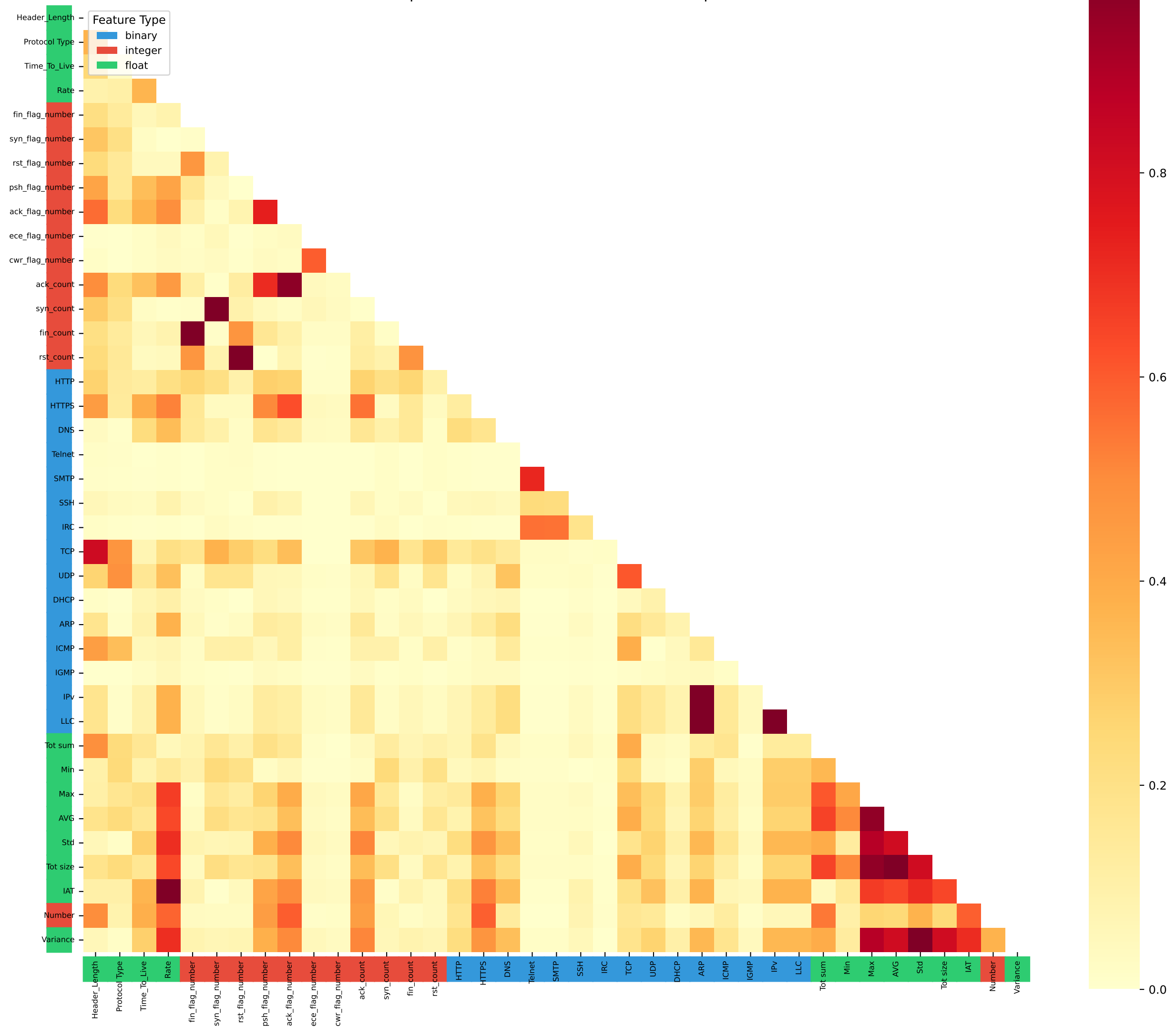
Spearman Absolute Correlation Heatmap
