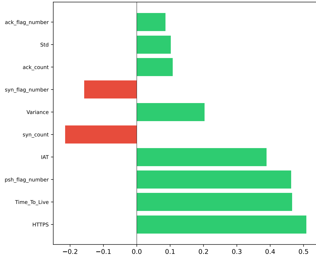
PC1 Top 10 Loadings (29.01% var)
