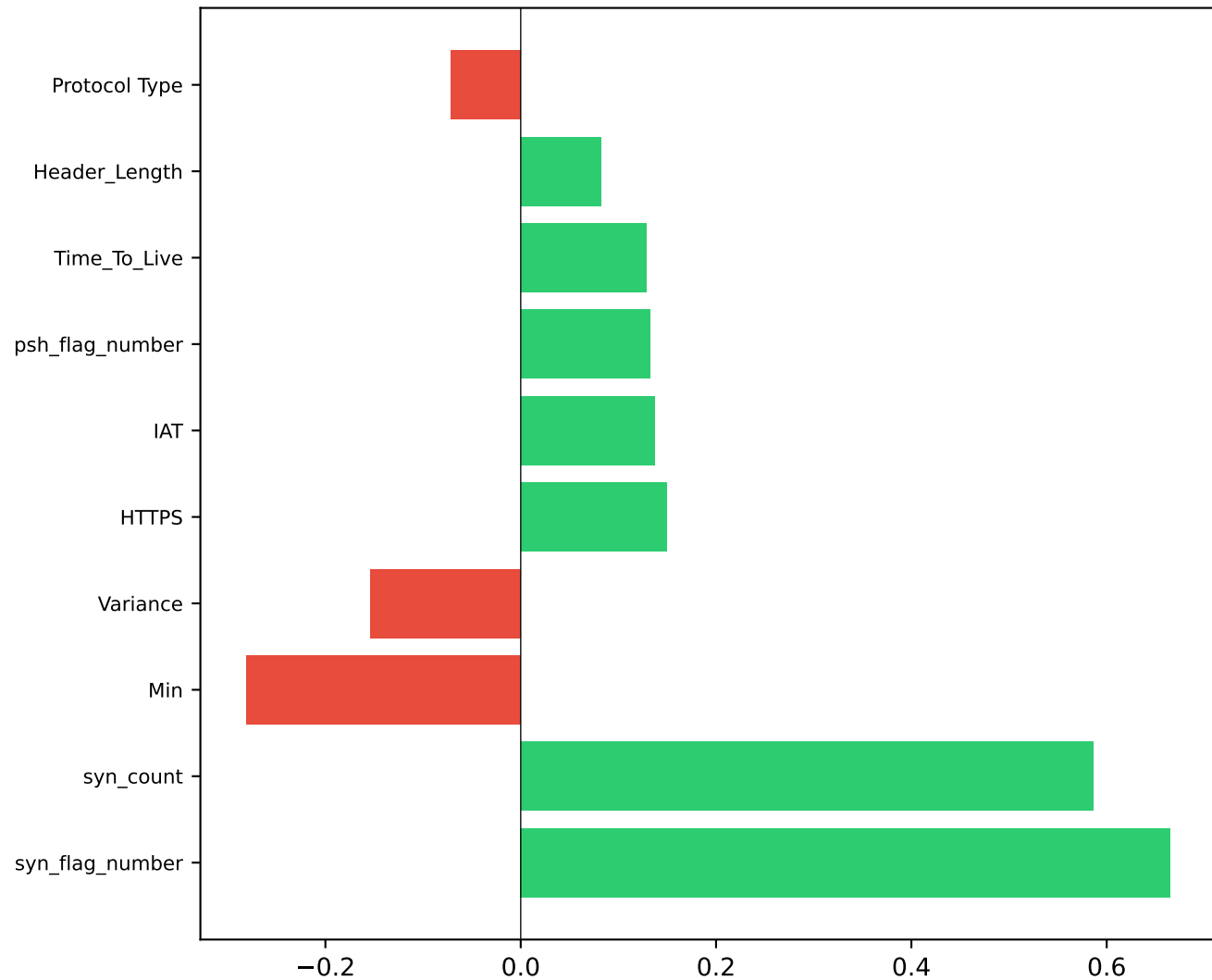
PC2 Top 10 Loadings (21.17% var)
