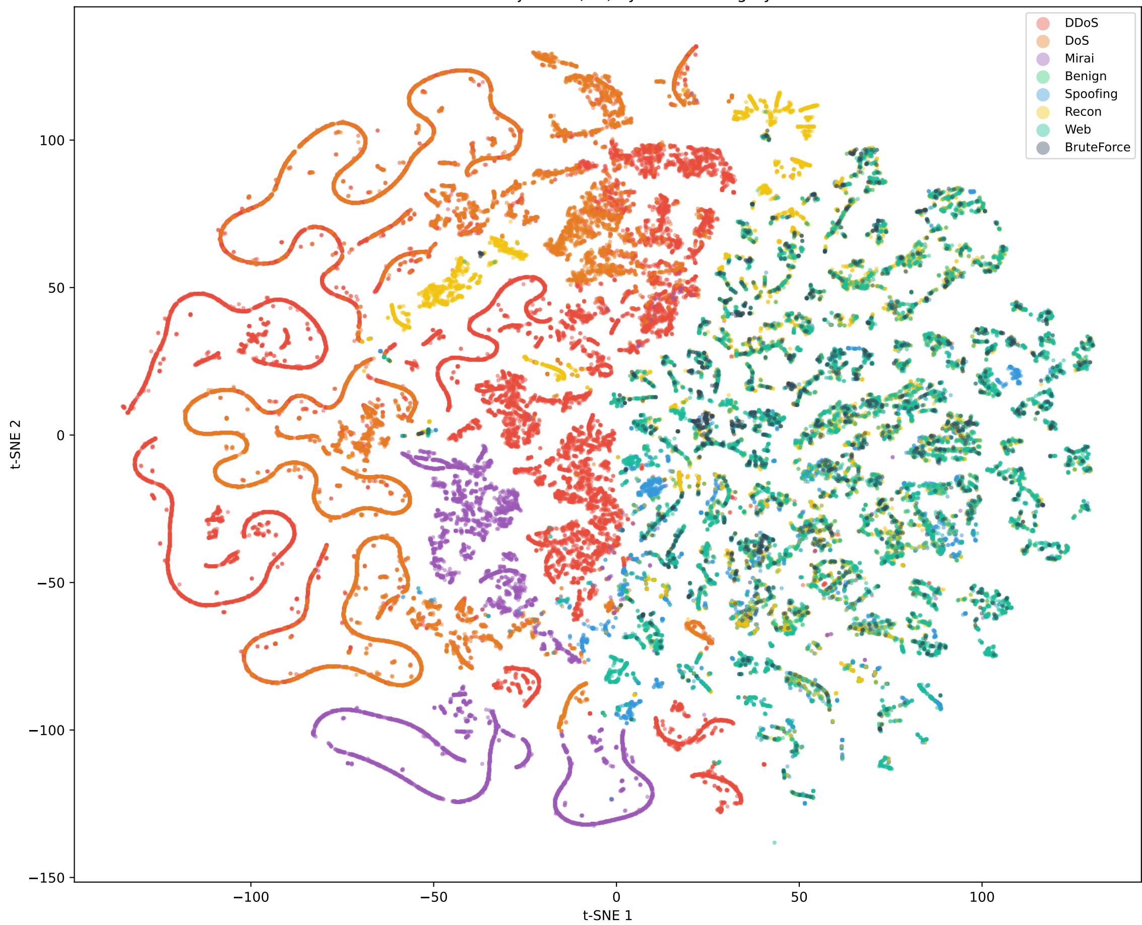
t-SNE Projection (2D) by Attack Category
