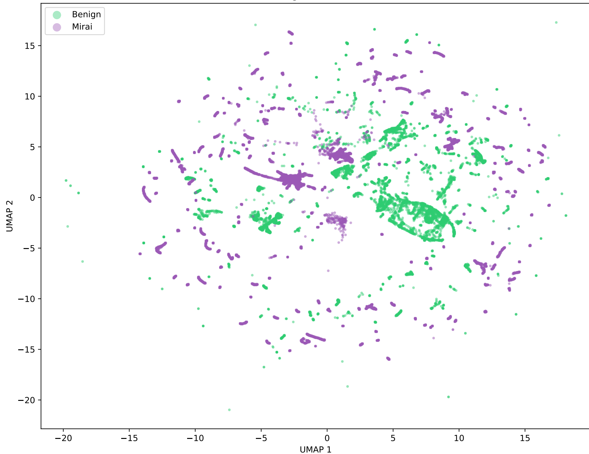
UMAP: Benignvs Mirai (zoomed)
