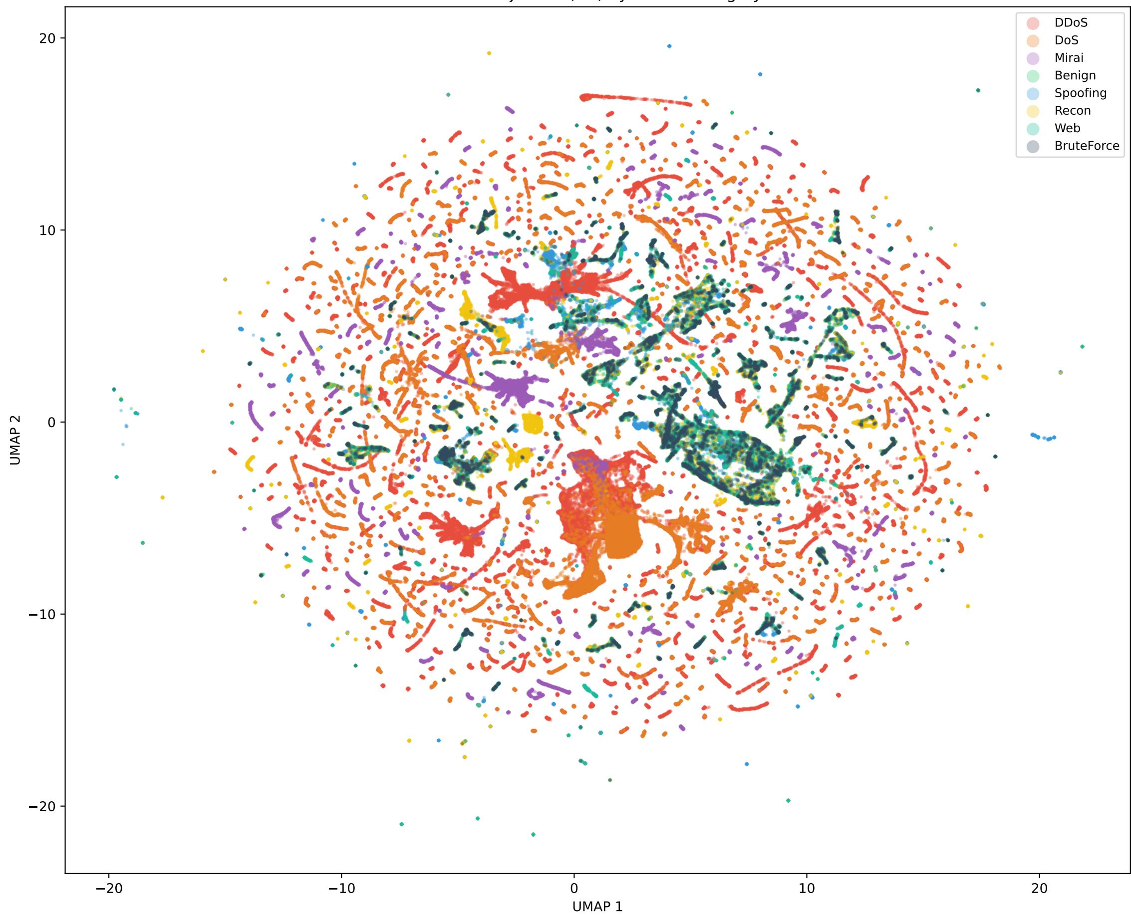
UMAP Projection (2D) by Attack Category
