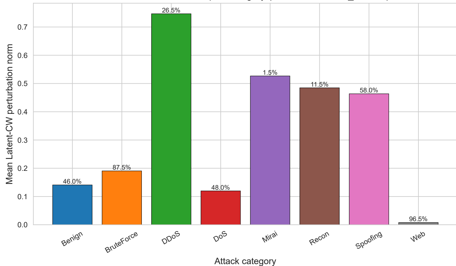
Latent Perturbation Size per Category (annotation = ASR_Valid %)
