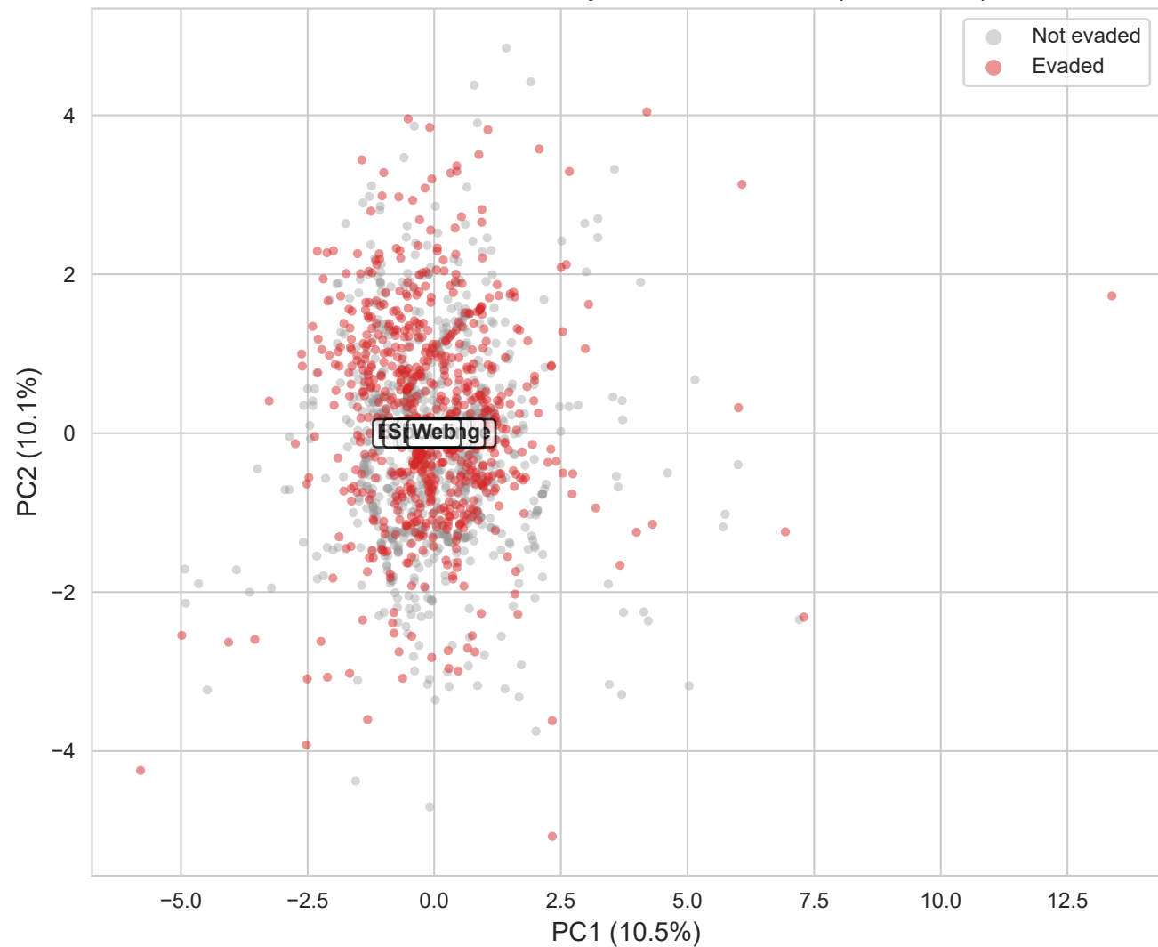
Class-Local Latent PCA by Evasion Success (Latent-CW)
