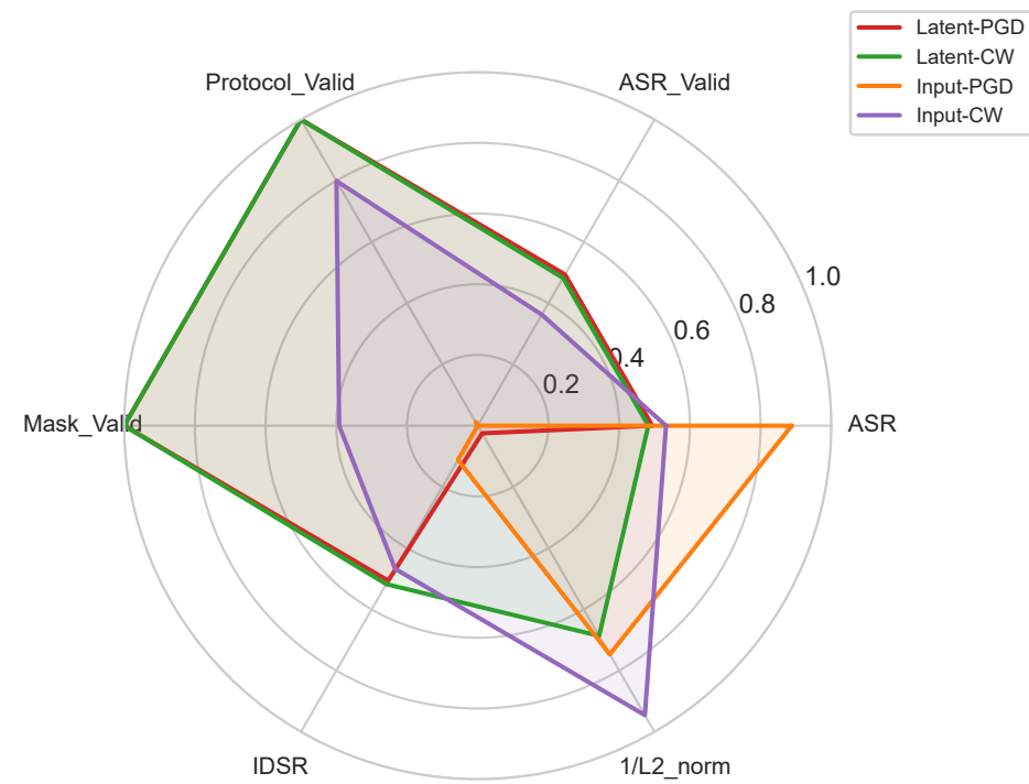
LSTM
