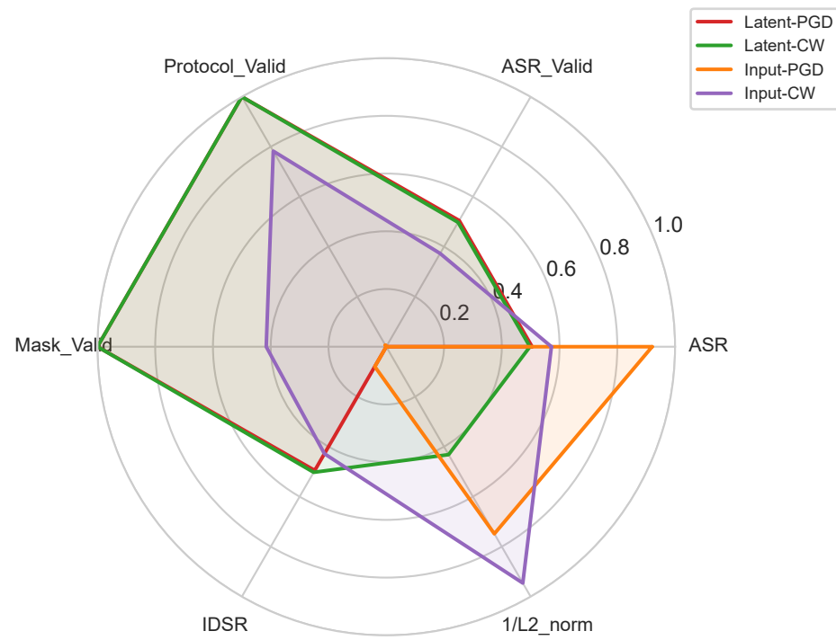
DualPath
