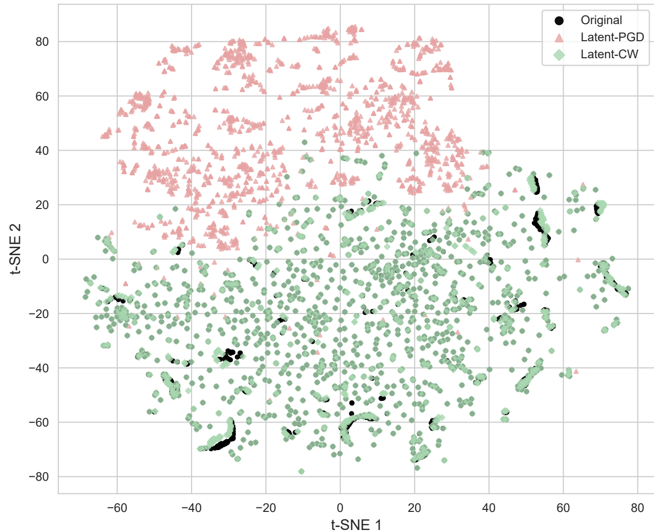
Class-Local Latent Codes: Original vs Perturbed
