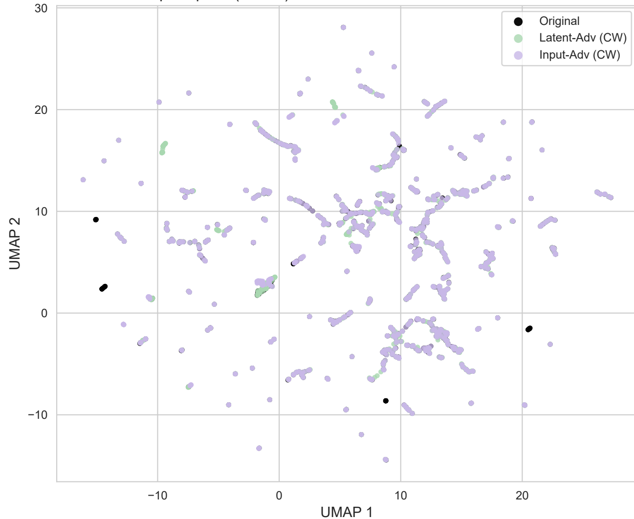
Input Space (UMAP): On-Manifold vs Off-Manifold Attacks
