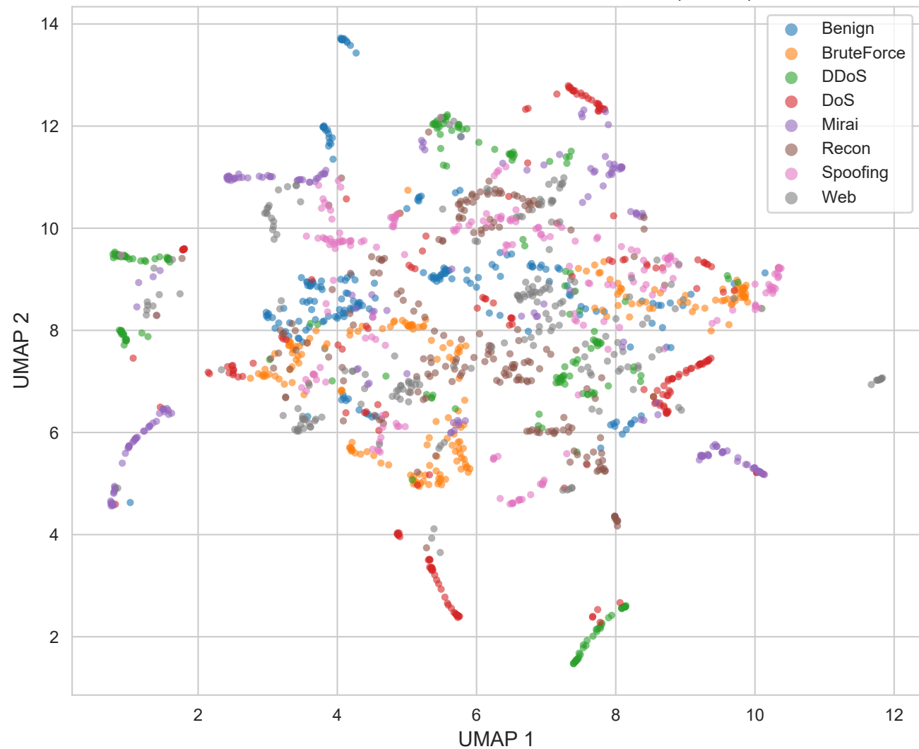
Class-Local Normalized VAE Latent Codes (UMAP)
