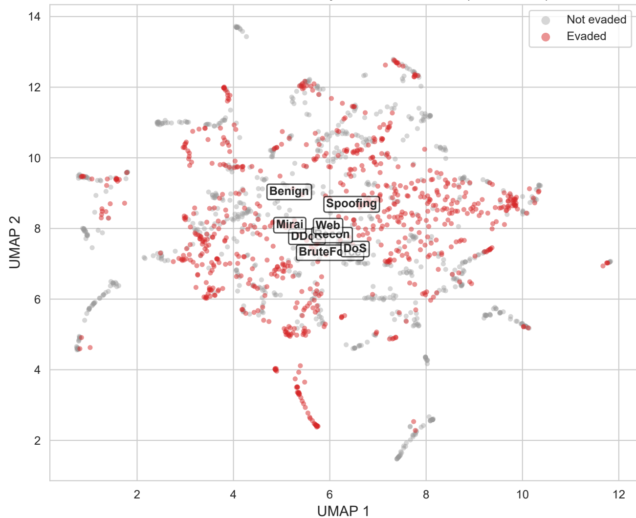
Class-Local Latent UMAP by Evasion Success (Latent-CW)
