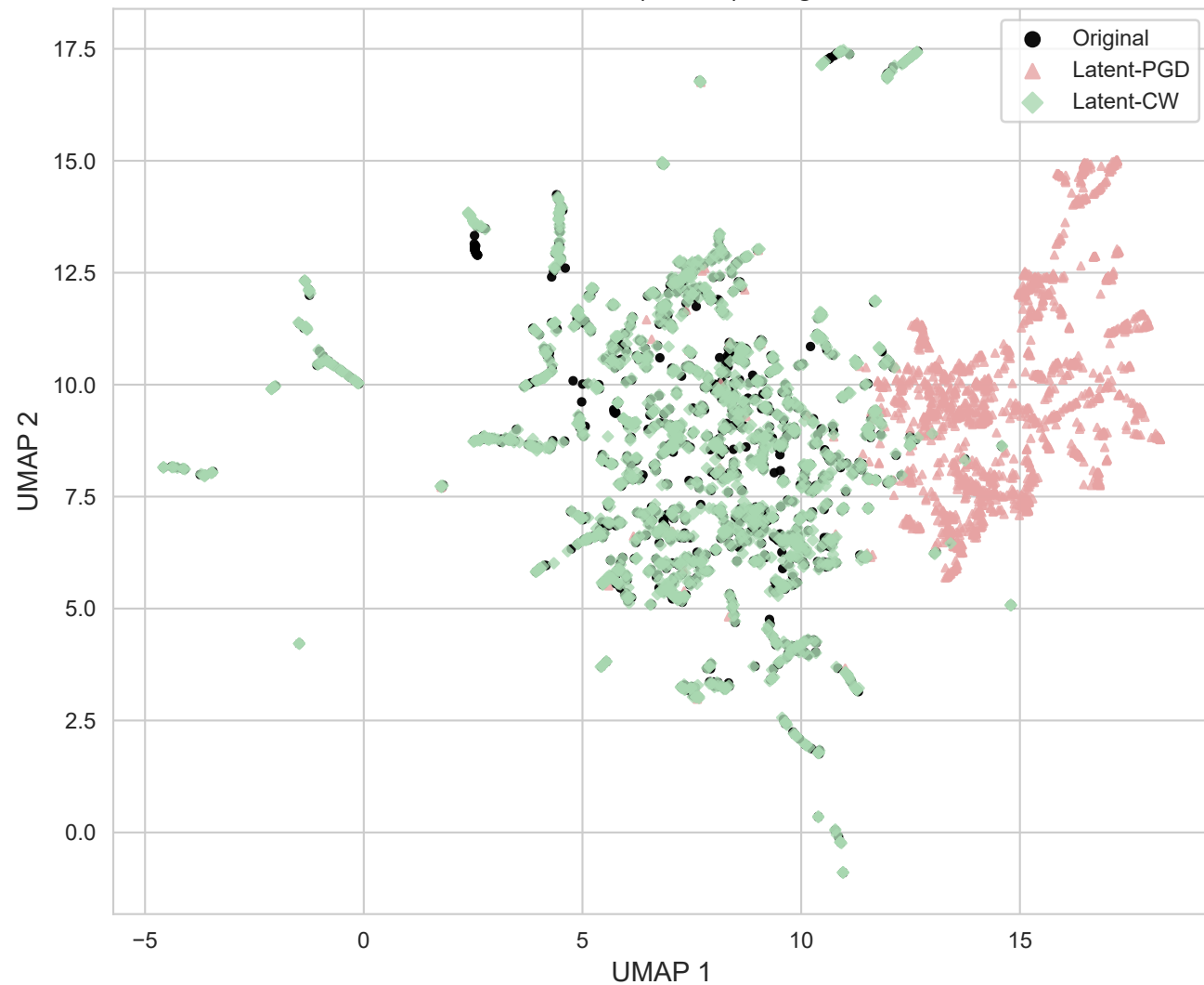
Class-Local Latent Codes (UMAP): Original vs Perturbed
