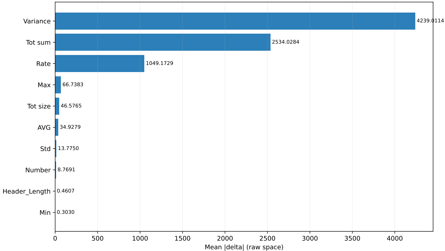
Top 10 Perturbed Features: CNN-LSTM CW eps=0 (8-class)
