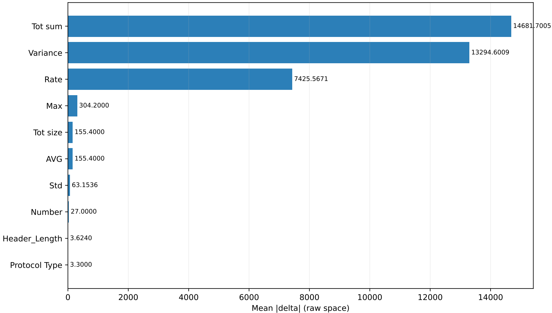
Top 10 Perturbed Features: CNN-LSTM FGSM eps=0.30 (8-class)
