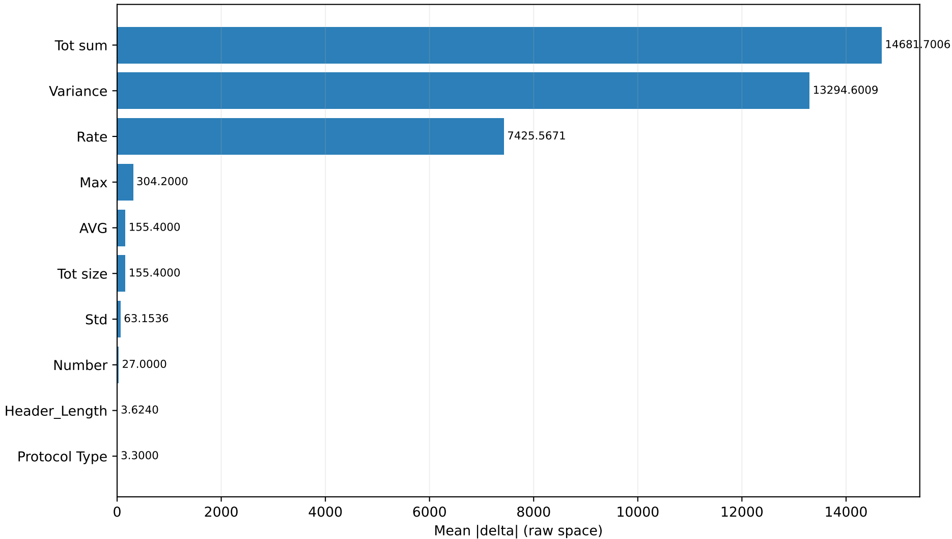
Top 10 Perturbed Features: LSTM FGSM eps=0.30 (8-class)
