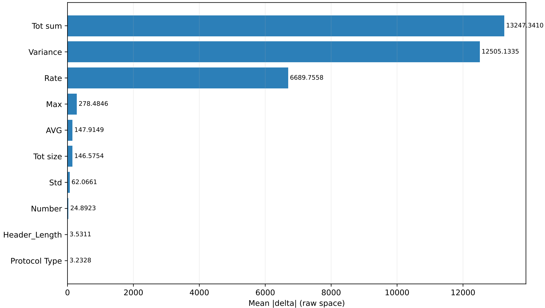
Top 10 Perturbed Features: LSTM PGD eps=0.30 (8-class)
