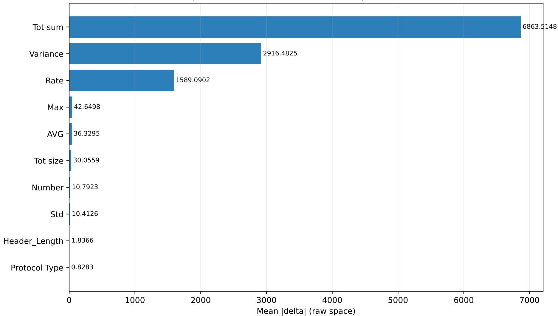
Top 10 Perturbed Features: MLP CW eps=0 (8-class)
