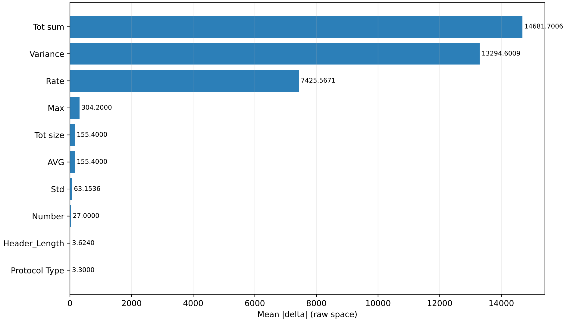
Top 10 Perturbed Features: MLP FGSM eps=0.30 (8-class)
