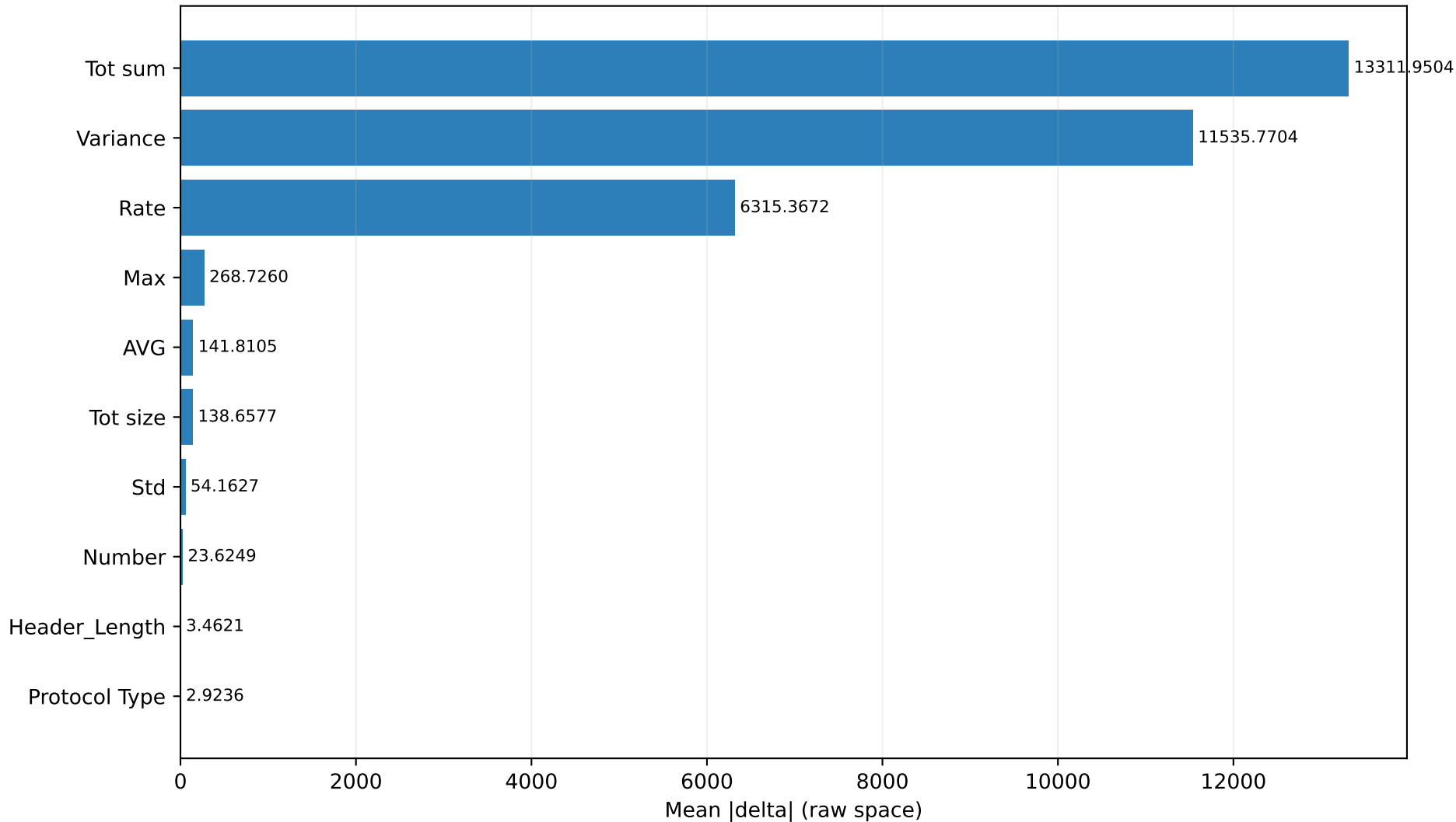
Top 10 Perturbed Features: MLP PGD eps=0.30 (8-class)
