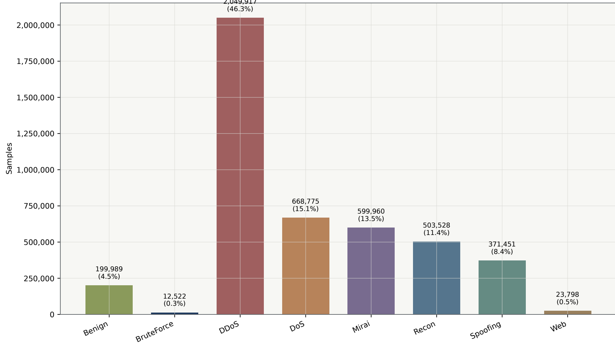
Raw/Staged CICIoT2023 Distribution by 8-Class Category
