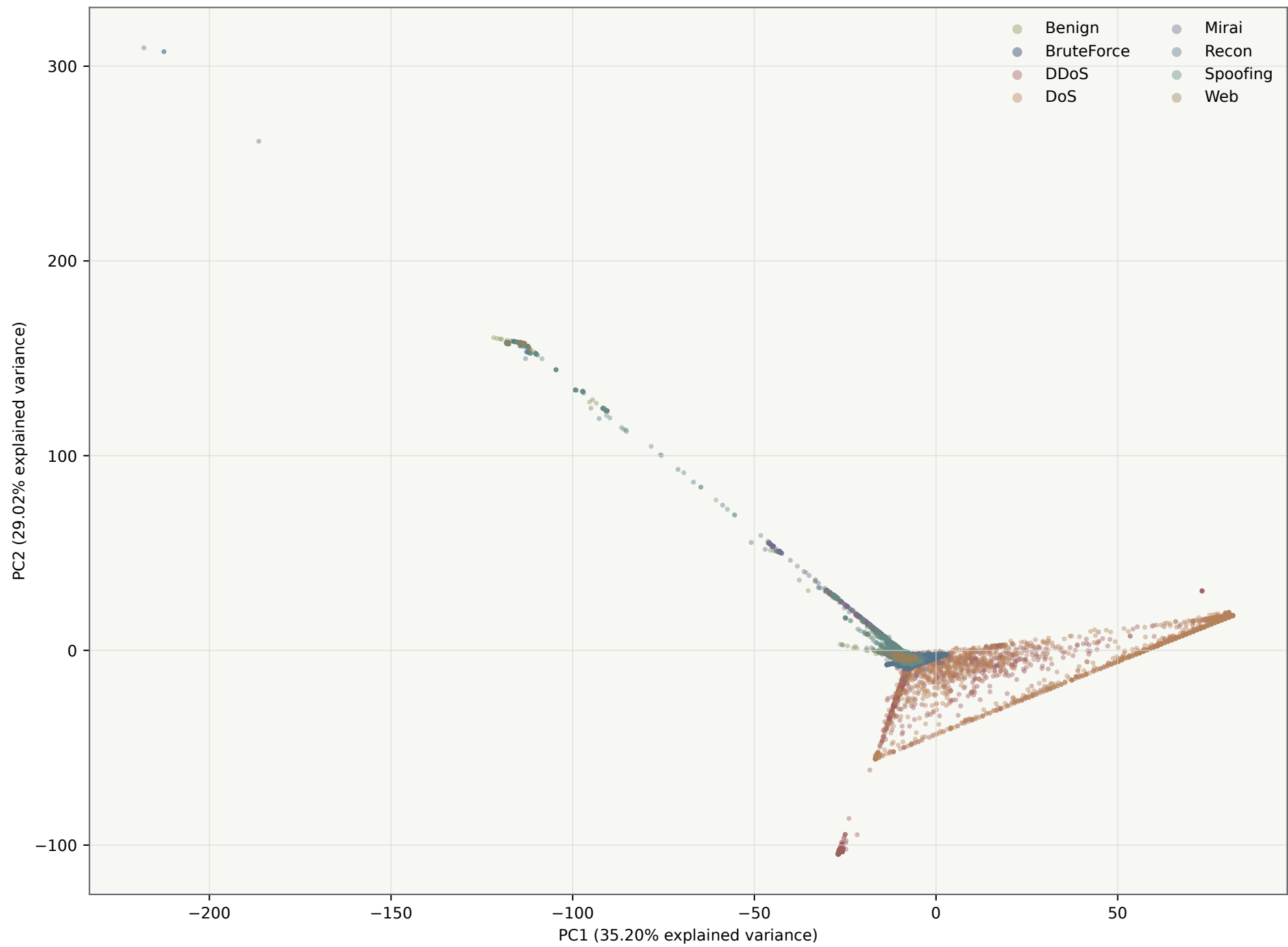
PCA of Scaled CICIoT2023 Features (PC1 + PC2 = 64.22%)
