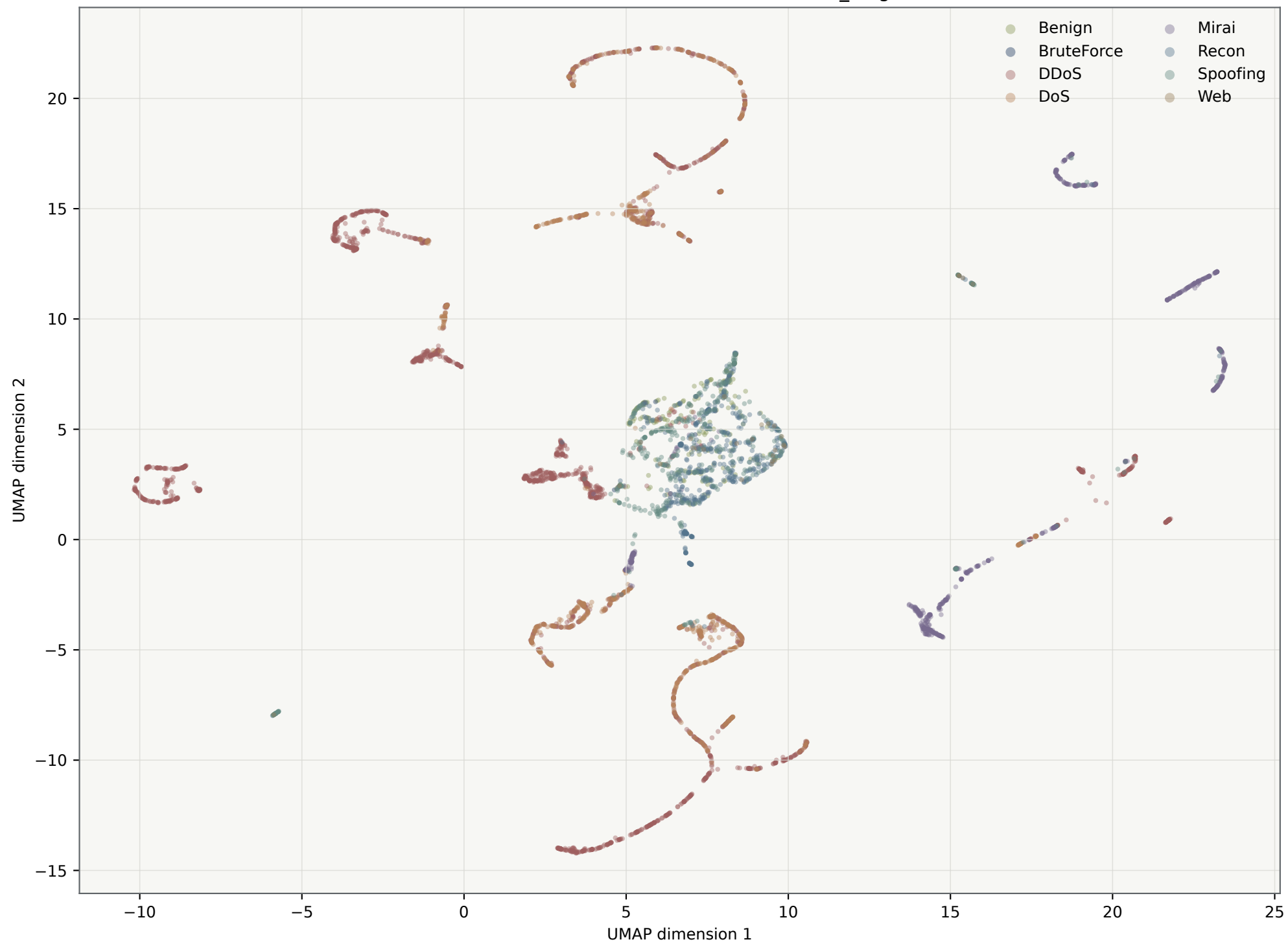
UMAP of Scaled CICIoT2023 Features (n=5,000, n_neighbors=30)
