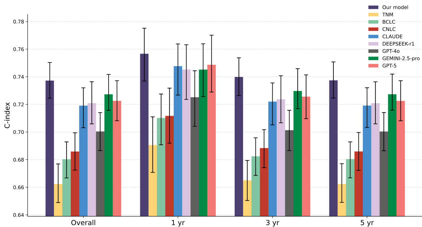
a. Overall and time-dependent C-index on the external test cohort
