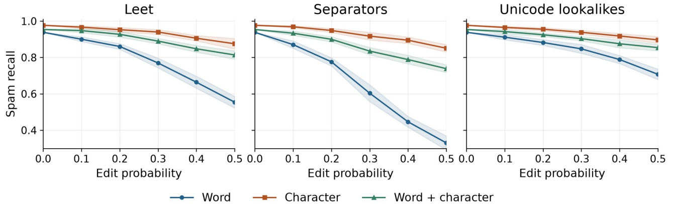
Figure 1. Default protocol, gentle cleanup and validation thresholds. Curves show mean spam recall; bands show one attack-seed standard deviation. All classifiers are LinearSVC. Different clean false-positive rates must be considered alongside recall.
