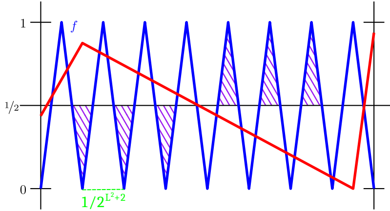
Figure 4.4: The target function f(x) = \Delta^{L^2+2}(x) is shown in blue, while the approximate function g(\mathbf{x}) is shown in red. We approximate the error between f and g by counting the number of half-triangles (shown with purple lines) that are created by intersecting the line x = \frac{1}{2} with f . Source: Telgarsky (2021) (slightly modified).
