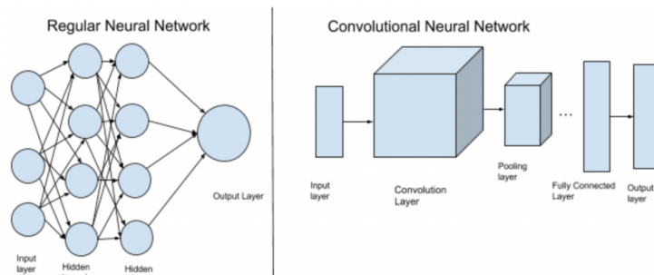
Figure 10.1: MLP vs CNN
