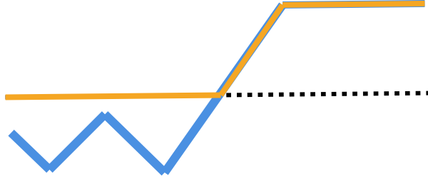
Figure 4.1: Illustration showing the effect of applying a ReLU function on a piecewise linear function. The dotted black line is the 0-axis. The piecewise linear function is shown in blue and the output of the ReLU function is shown in orange.
