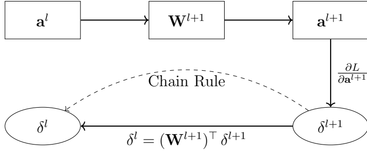
Figure 6.2: Illustration of the forward and backward pass.
