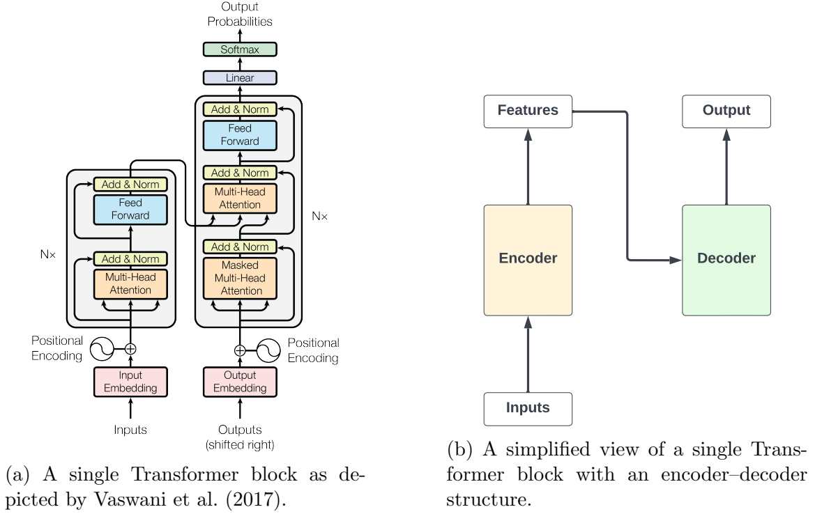
Figure 10.20: Overview of a single block of the Transformer architecture.
