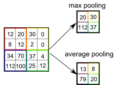
Figure 10.10: Max pooling over 2 \times 2 window.
