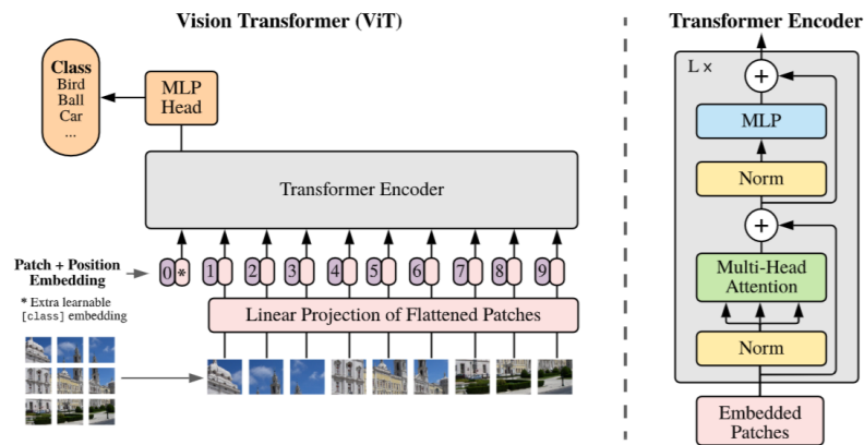
Figure 10.24: Illustration of a ViT Dosovitskiy et al. (2020).
