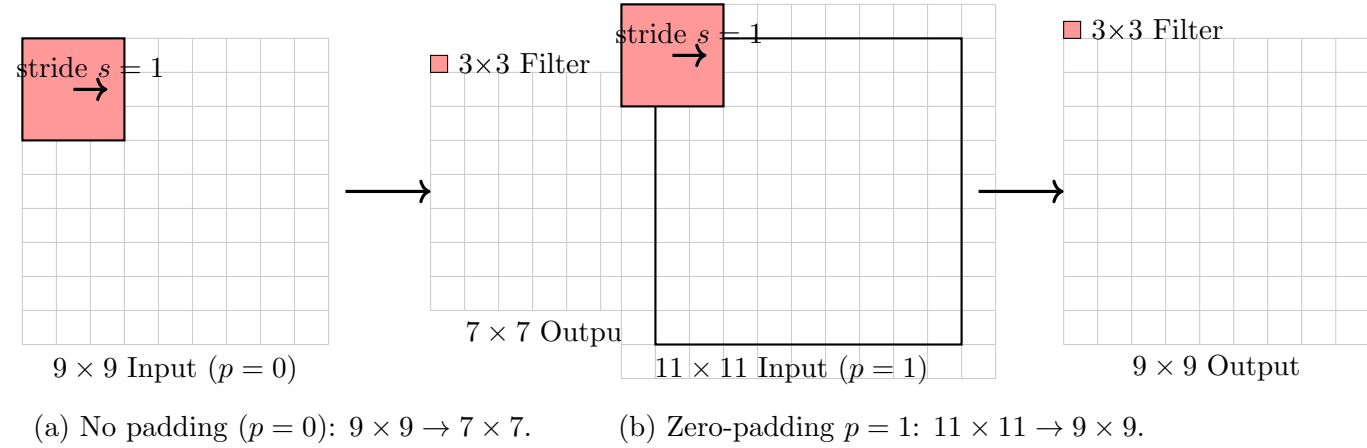
Figure 10.7: Effect of zero-padding on convolution output size.
