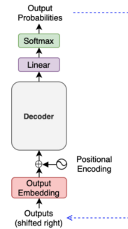
Figure 10.22: The decoder generates tokens sequentially. Source: kikaben.com.
