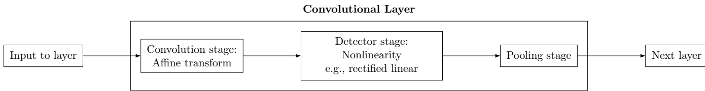
Figure 10.9: Convolutional layer stages: activation and pooling.
