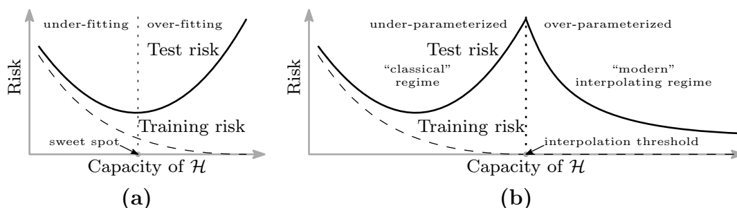
Figure 13.1: Curves for training risk (dashed line) and test risk (solid line). Figure from Belkin et al. (2019) (a) The classical U-shaped risk curve arising from the bias-variance trade-off. (b) The double descent risk curve , which incorporates the U-shaped risk curve (i.e., the “classical” regime) together with the observed behavior from using high capacity function classes (i.e., the “modern” interpolating regime), separated by the interpolation threshold. The predictors to the right of the interpolation threshold have zero training risk.
