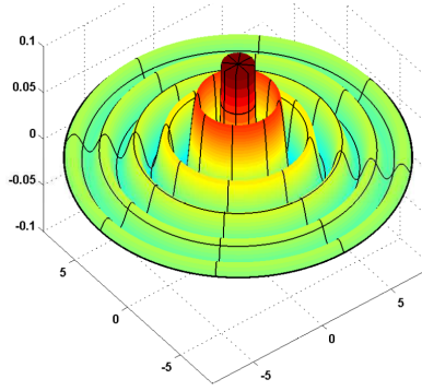
Figure 4.5: Illustration of the \phi(\mathbf{x}) function, which is a rescaled version of \text{sinc}(\|\mathbf{x}\|) = \frac{\sin(\|\mathbf{x}\|)}{\|\mathbf{x}\|} .
