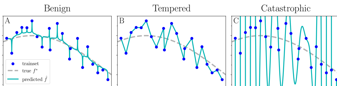
Figure 13.3: As n \rightarrow \infty , interpolating methods can exhibit three types of overfitting. (A) In benign overfitting , the predictor asymptotically approaches the ground-truth, Bayes-optimal function. Nadaraya-Watson kernel smoothing with a singular kernel, shown here, is asymptotically benign. (B) In tempered overfitting , the predictor approaches a constant test risk greater than the Bayes-optimal risk. Piecewise-linear interpolation is asymptotically tempered. (C) In catastrophic overfitting , the predictor generalizes arbitrarily poorly. Rank- n polynomial interpolation is asymptotically catastrophic.
