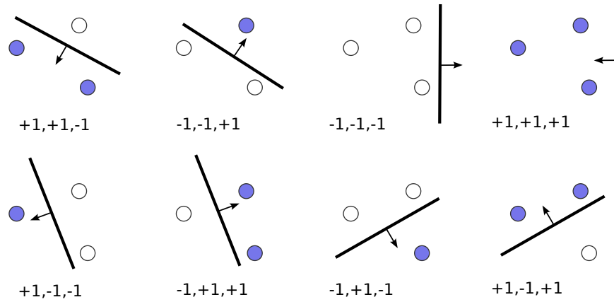
Figure 8.1: Illustration of the concept of growth function.
