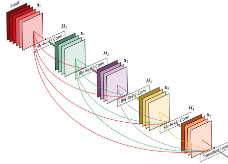
Figure 10.16: Dense block connectivity: each layer concatenates all preceding feature-maps.
