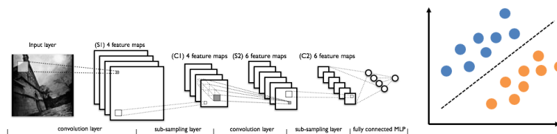
Figure 10.12: Fully-connected layers for classification.
