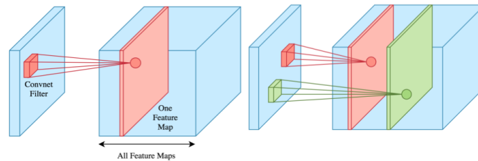
Figure 10.11: Multiple channels in convolutional layers.
