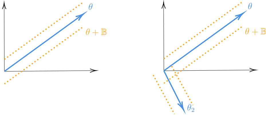
Figure 4.6: Left: Illustration of \text{supp}(\hat{\sigma} \star \hat{\phi}) as the space between the blue arrow and the dotted oranges lines; Right: by adding a second vector \theta_2 , we increase the support.
