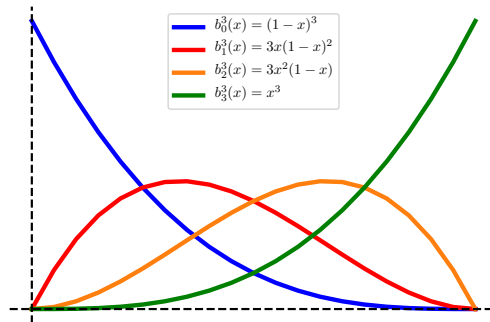
Figure 3.2: Example of Bernstein basis for degree m = 3 . Source: Wikipedia.
