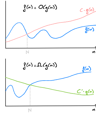
Figure 12.3: \mathcal{O} vs \Omega notation.
