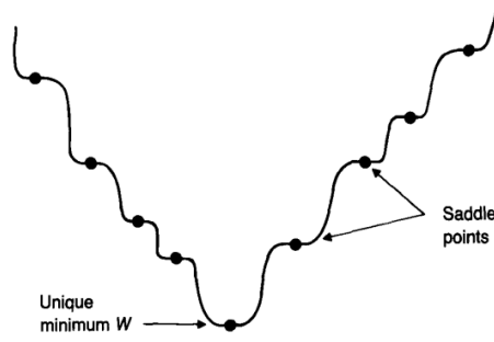
Figure 6.1: The landscape of the objective function (figure taken from Baldi and Hornik (1989)).
