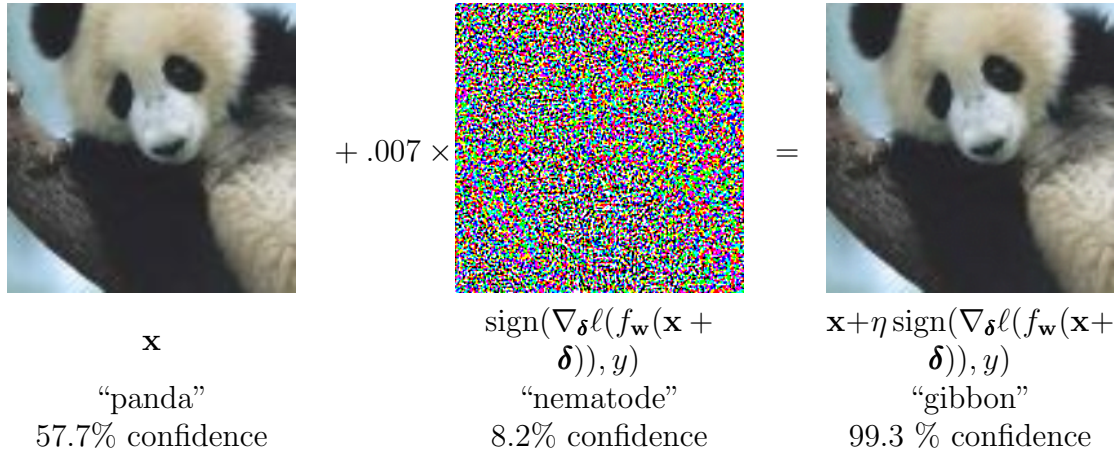
Figure 12.1: A demonstration of fast adversarial example generation applied to GoogLeNet on ImageNet. By adding an imperceptibly small perturbation \delta whose elements are equal to the sign of the elements of the gradient of the cost function with respect to the input, we can change GoogLeNet’s classification of the image. Here \eta = 0.007 corresponds to the magnitude of the smallest bit of an 8-bit image encoding after GoogLeNet’s conversion to real numbers.
