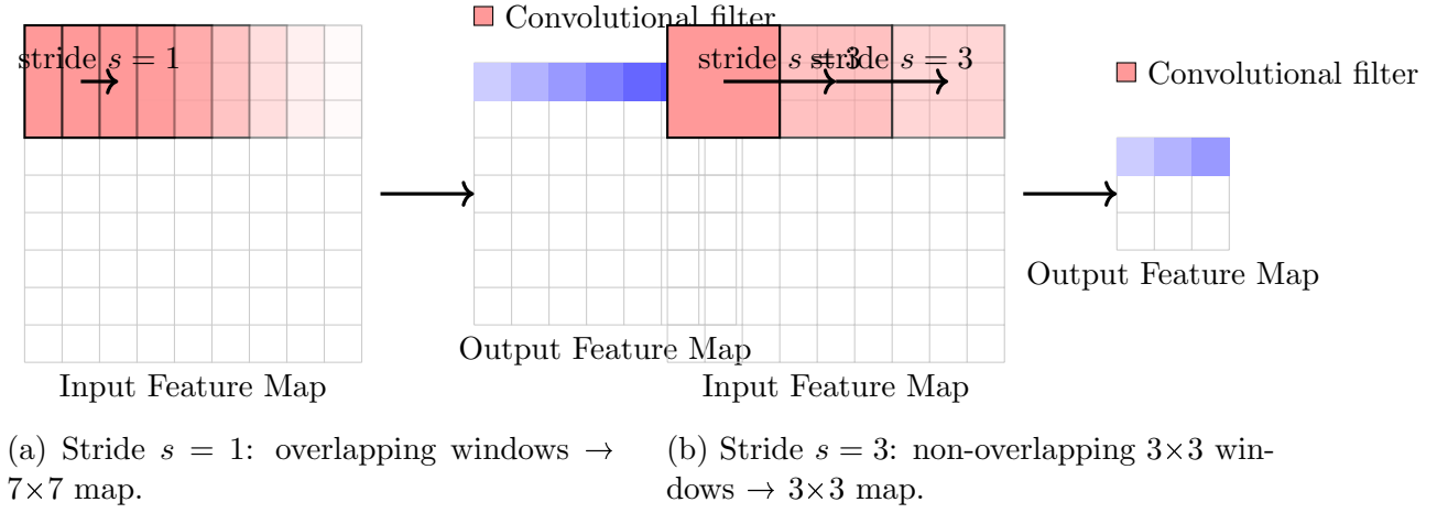
Figure 10.6: Comparison of convolution strides on a 9 \times 9 input: (a) stride 1 yields a 7 \times 7 feature map with overlapping receptive fields; (b) stride 3 yields a 3 \times 3 feature map.
