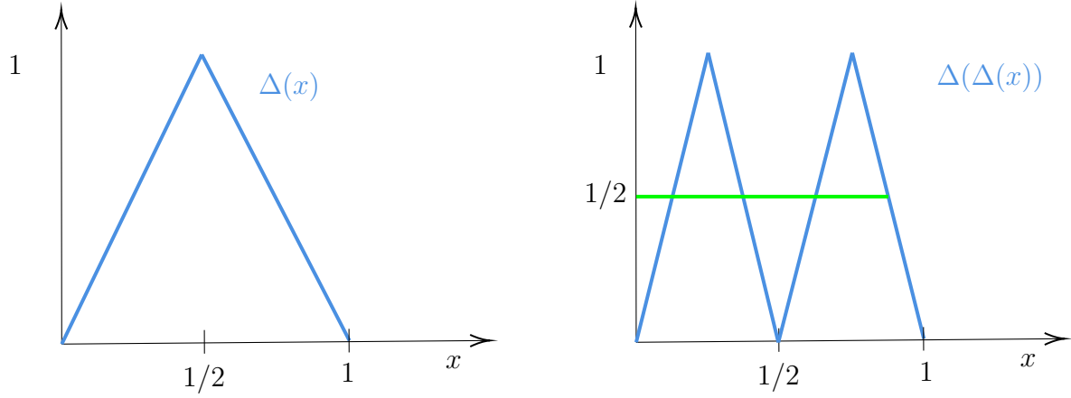
Figure 4.3: Illustration of the \Delta(x) function as well as \Delta(\Delta(x)) .
