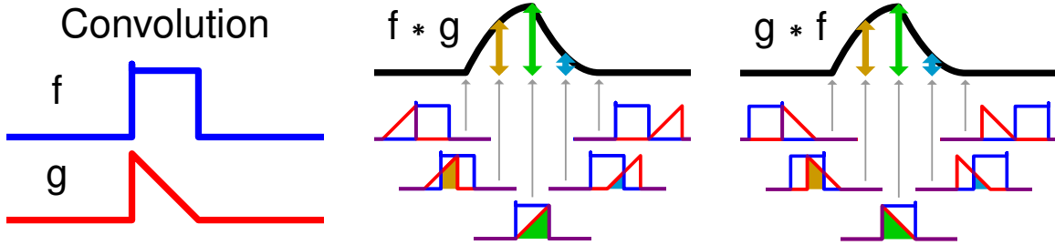
Figure 10.4: Visualization of continuous convolution (source: Wikipedia).
