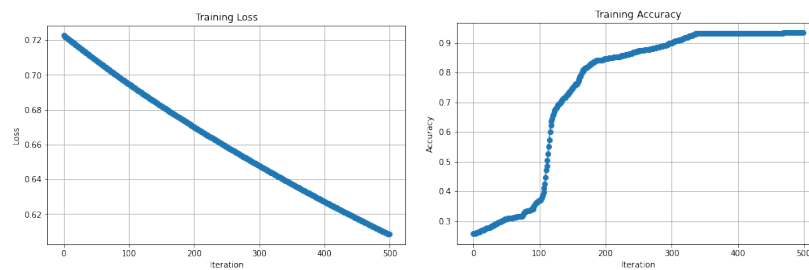
Figure 2.10: Loss and accuracy
