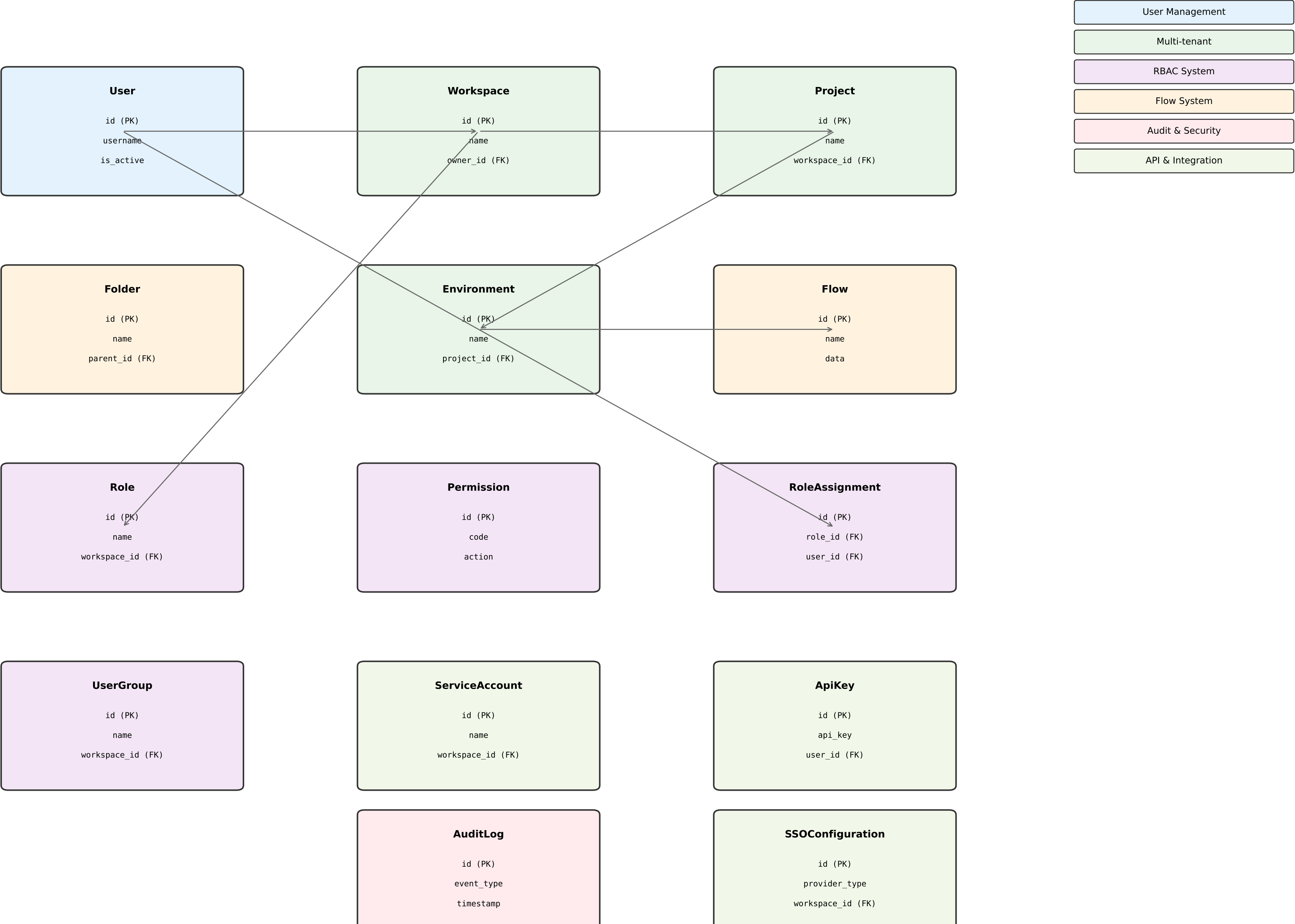
LangBuilder Database Entity-Relationship Diagram
