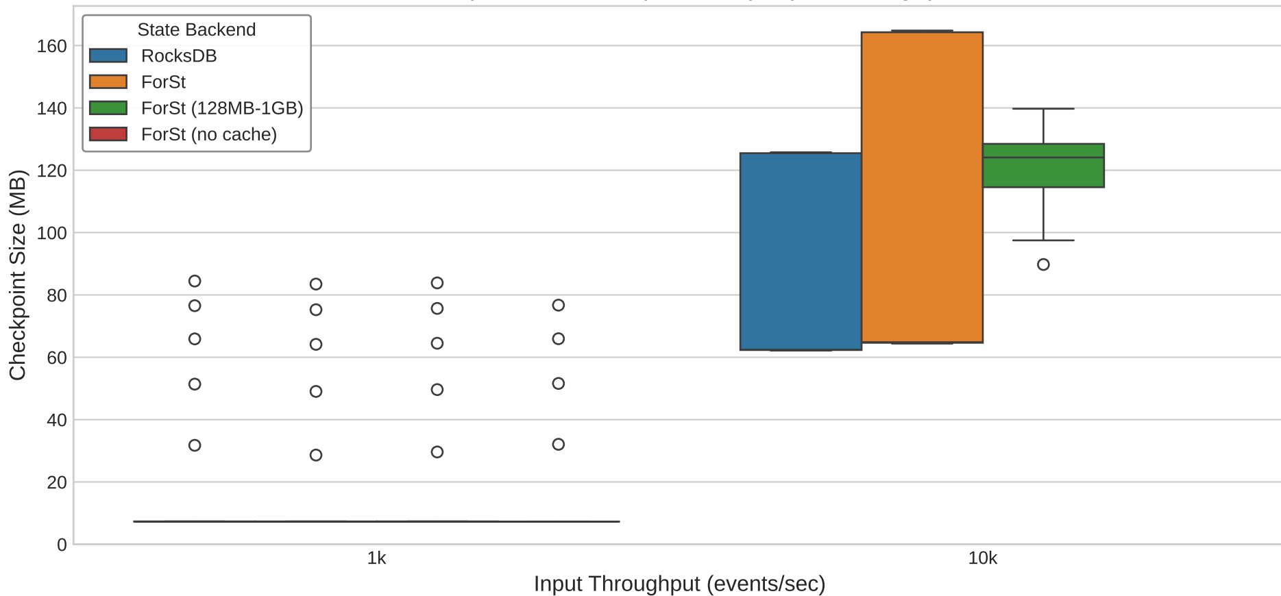
Checkpoint Size Comparison by Input Throughput
