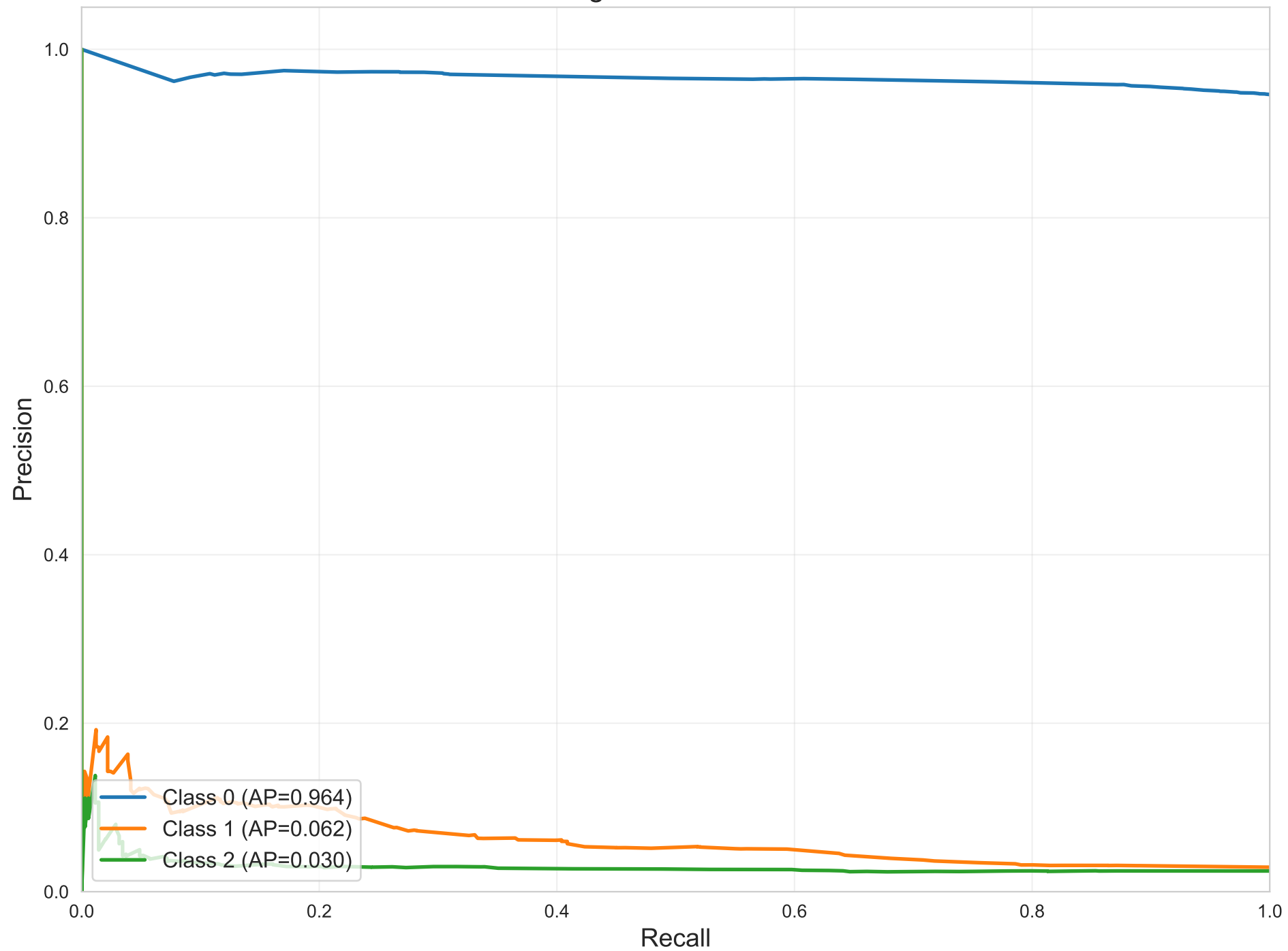
PR Curves per Class - Decision Tree Weighted AP = 0.915
