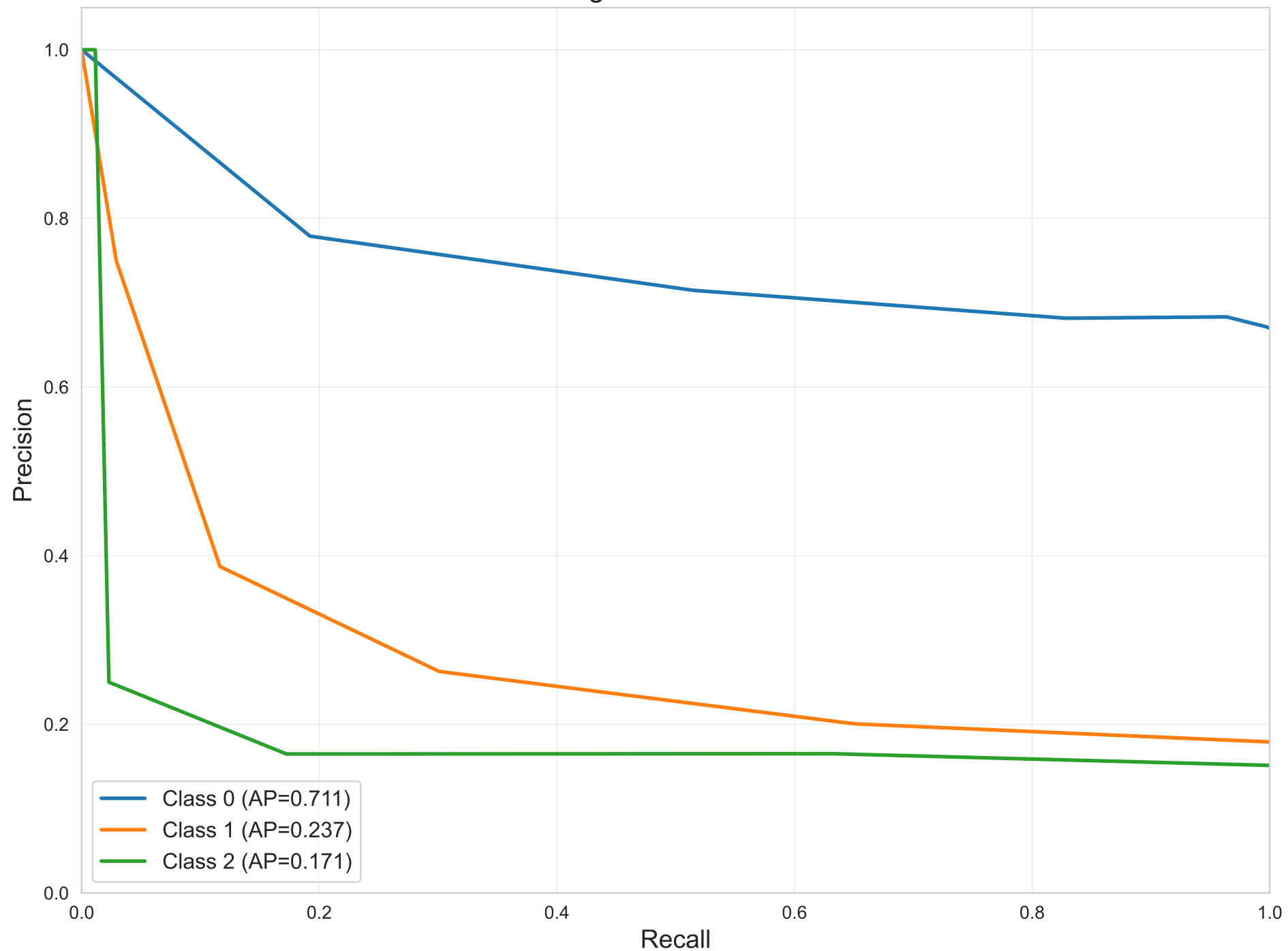
PR Curves per Class - K Nearest Neighbors Weighted AP = 0.544
