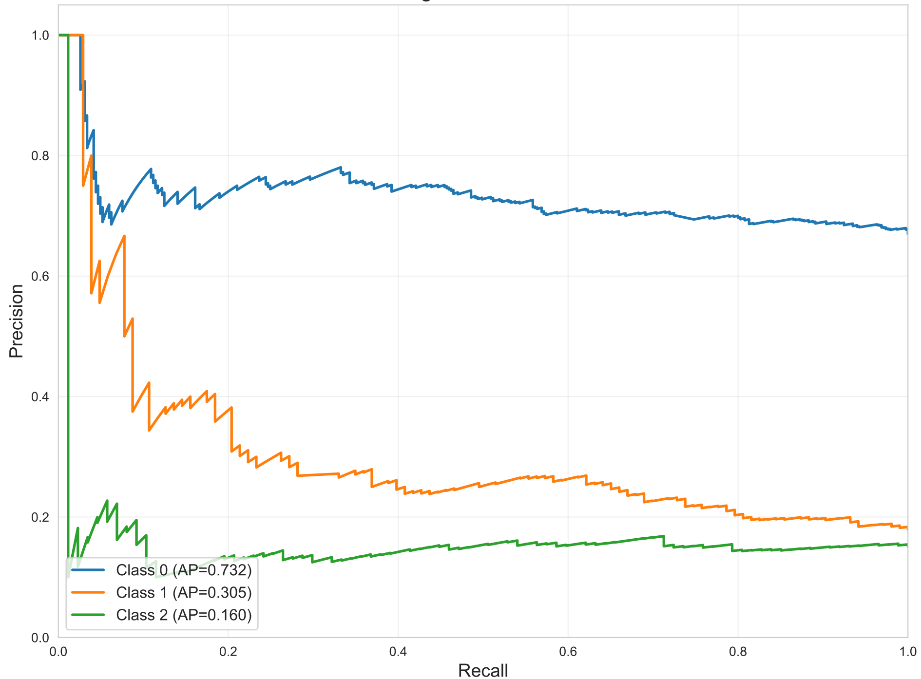
PR Curves per Class - Multi Layer Perceptron Weighted AP = 0.569
