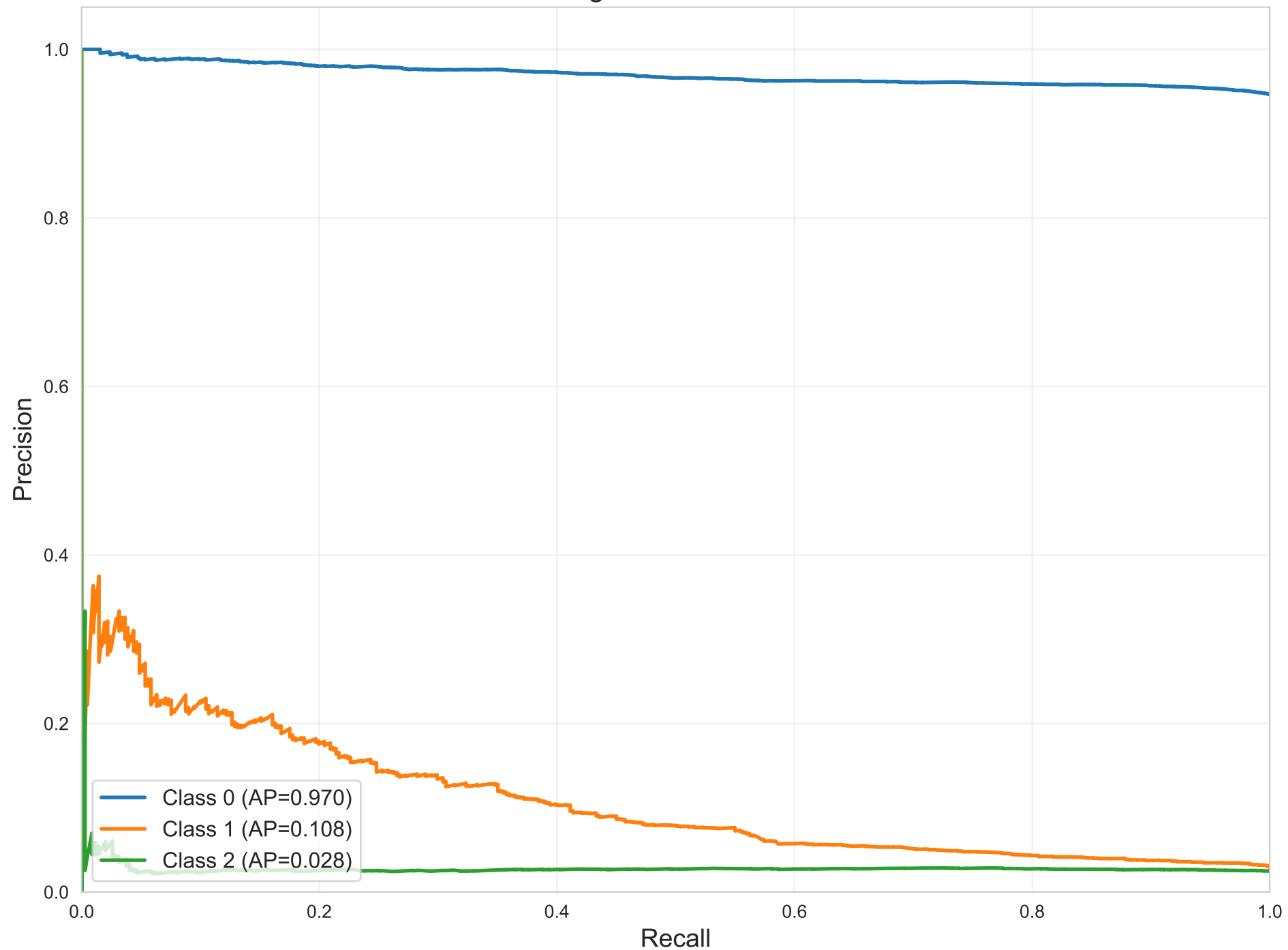
PR Curves per Class - Random Forest Weighted AP = 0.922
