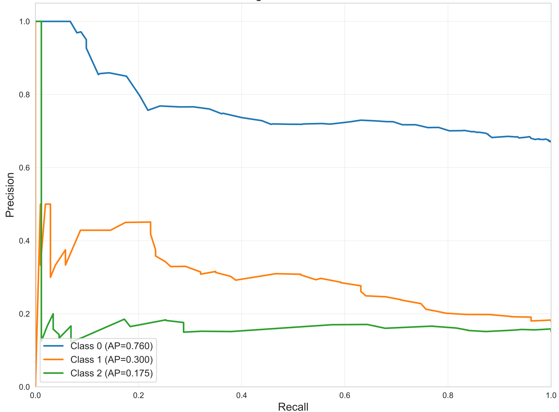
PR Curves per Class - Random Forest Weighted AP = 0.589
