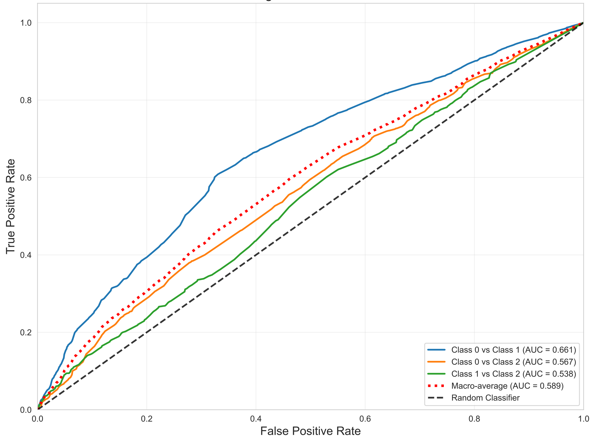
One-vs-One ROC - Decision Tree Weighted AUC = 0.612
