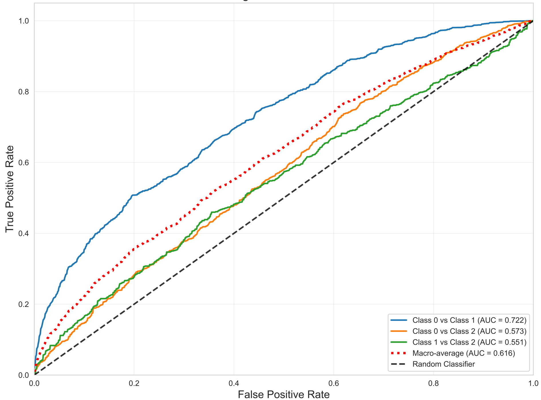
One-vs-One ROC - Random Forest Weighted AUC = 0.645
