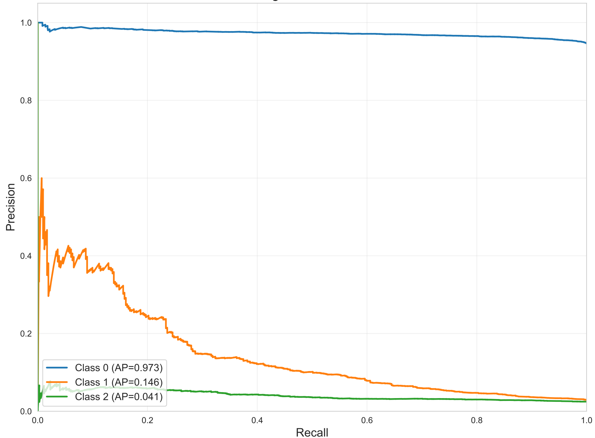
PR Curves per Class - Gradient Boosting Weighted AP = 0.926
