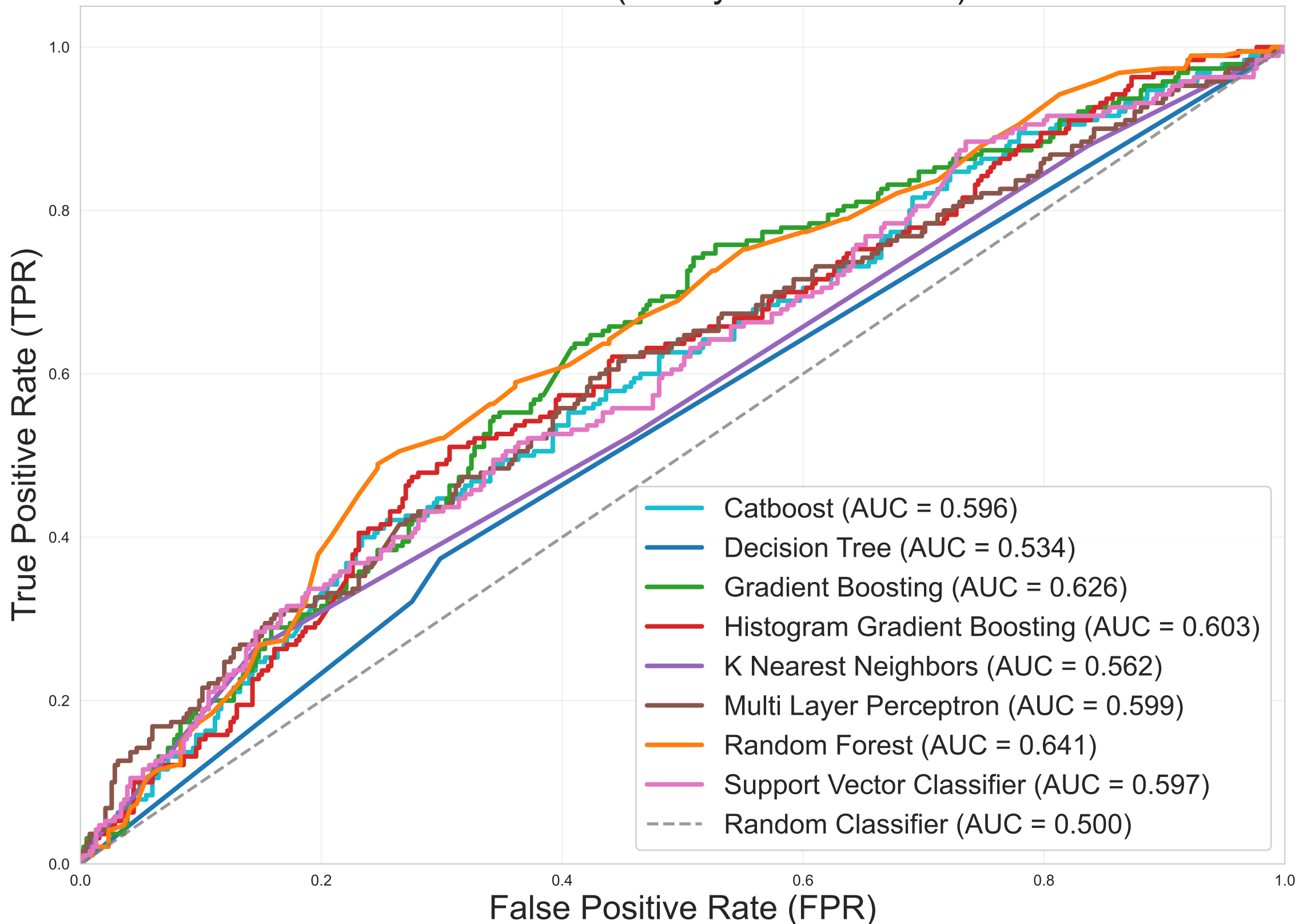
ROC Curves (Binary Classification)
