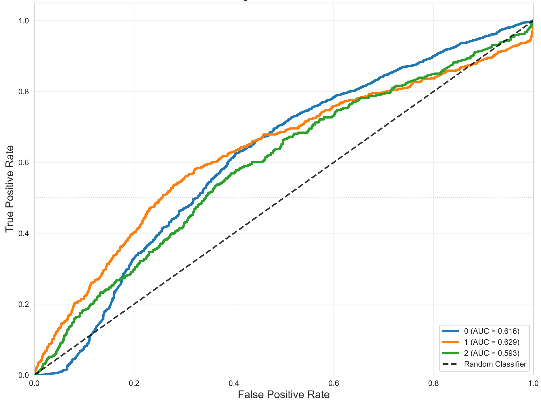
One-vs-Rest ROC - Support Vector Classifier Weighted AUC = 0.616
