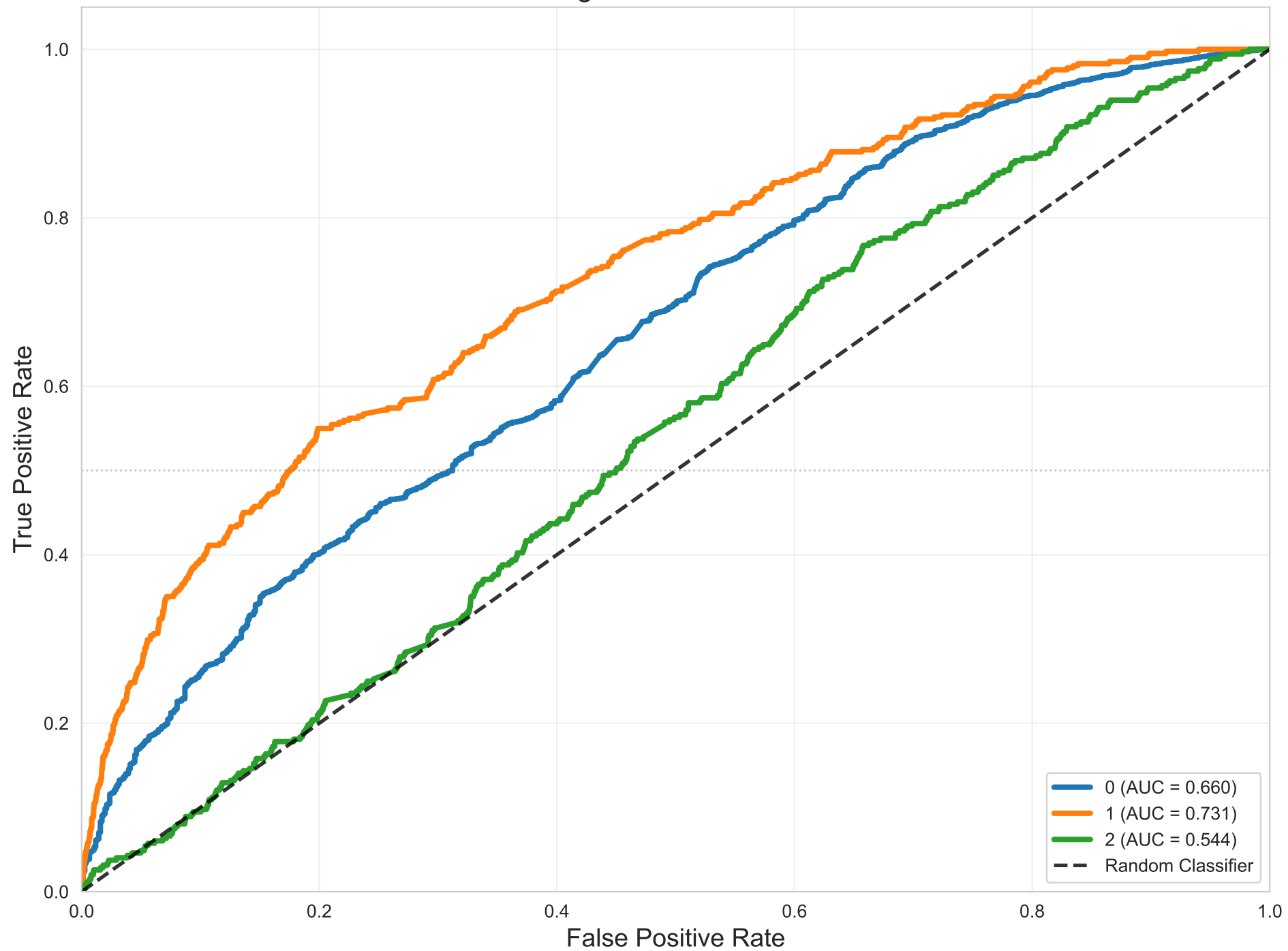
One-vs-Rest ROC - Random Forest Weighted AUC = 0.659
