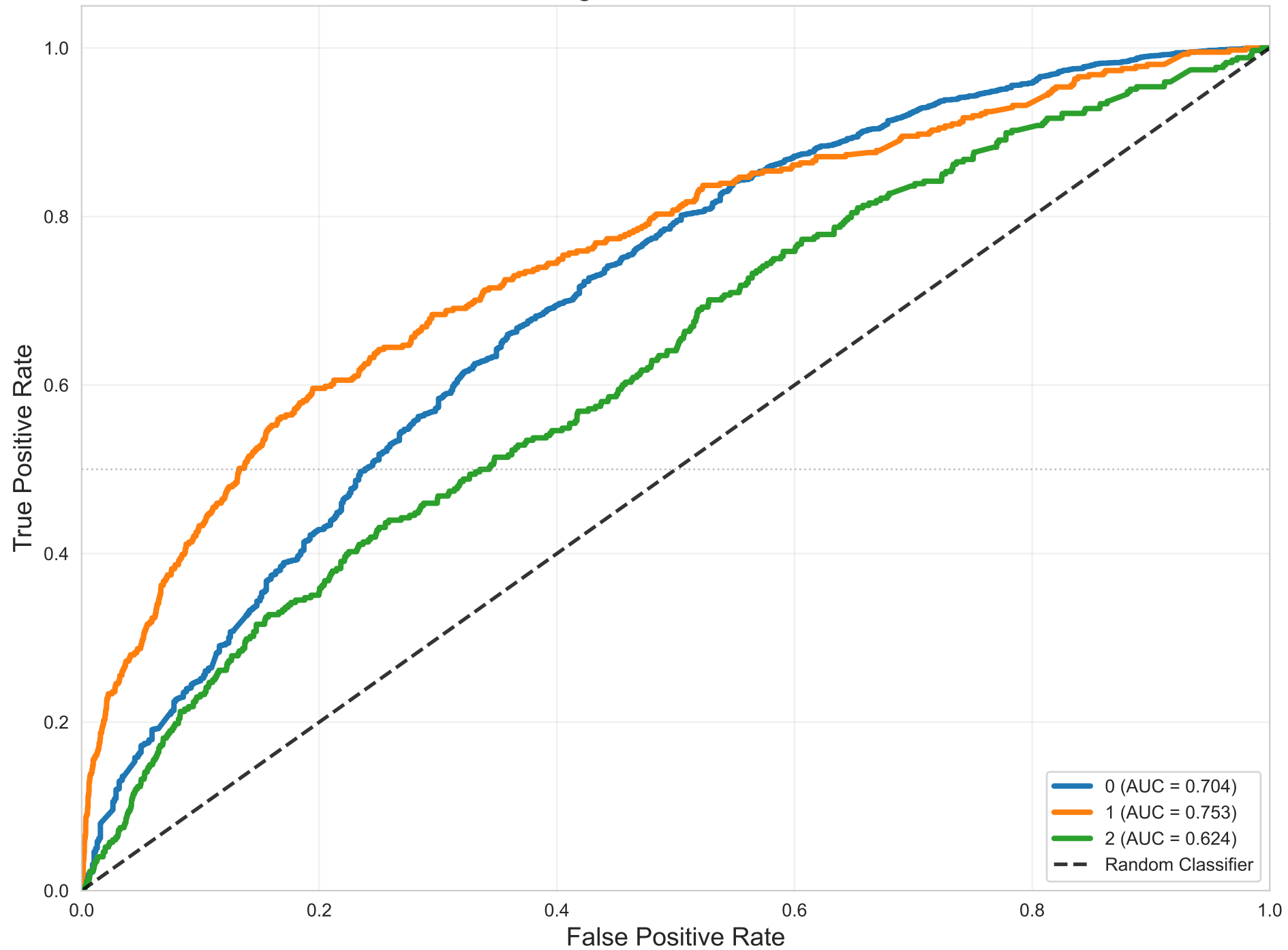
One-vs-Rest ROC - Gradient Boosting Weighted AUC = 0.704
