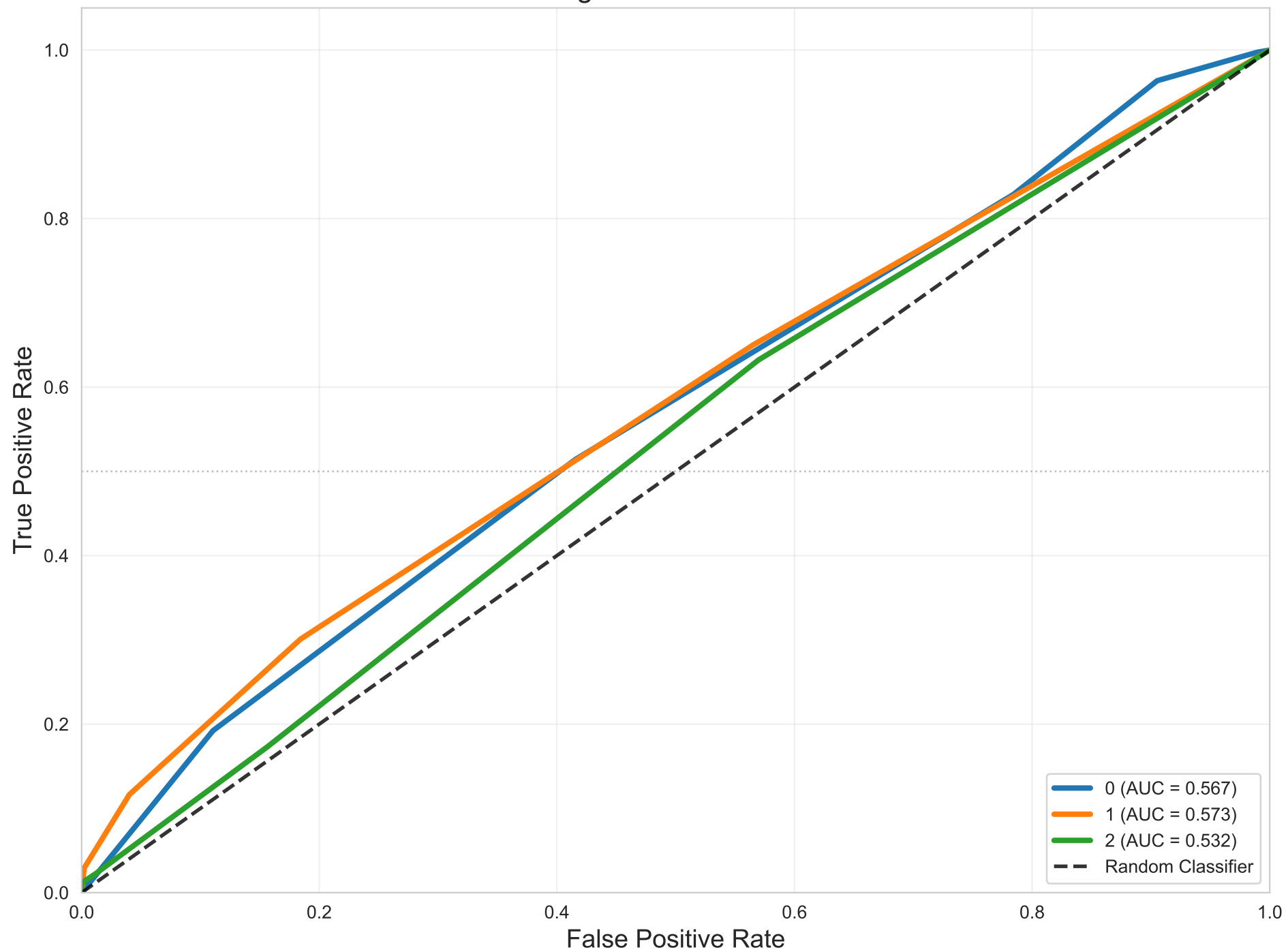
One-vs-Rest ROC - K Nearest Neighbors Weighted AUC = 0.563
