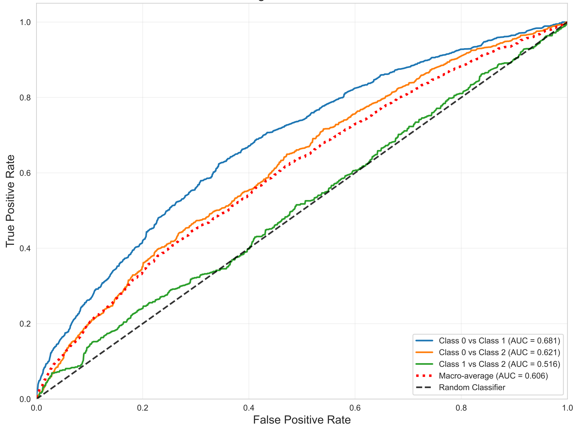
One-vs-One ROC - Multi Layer Perceptron Weighted AUC = 0.648
