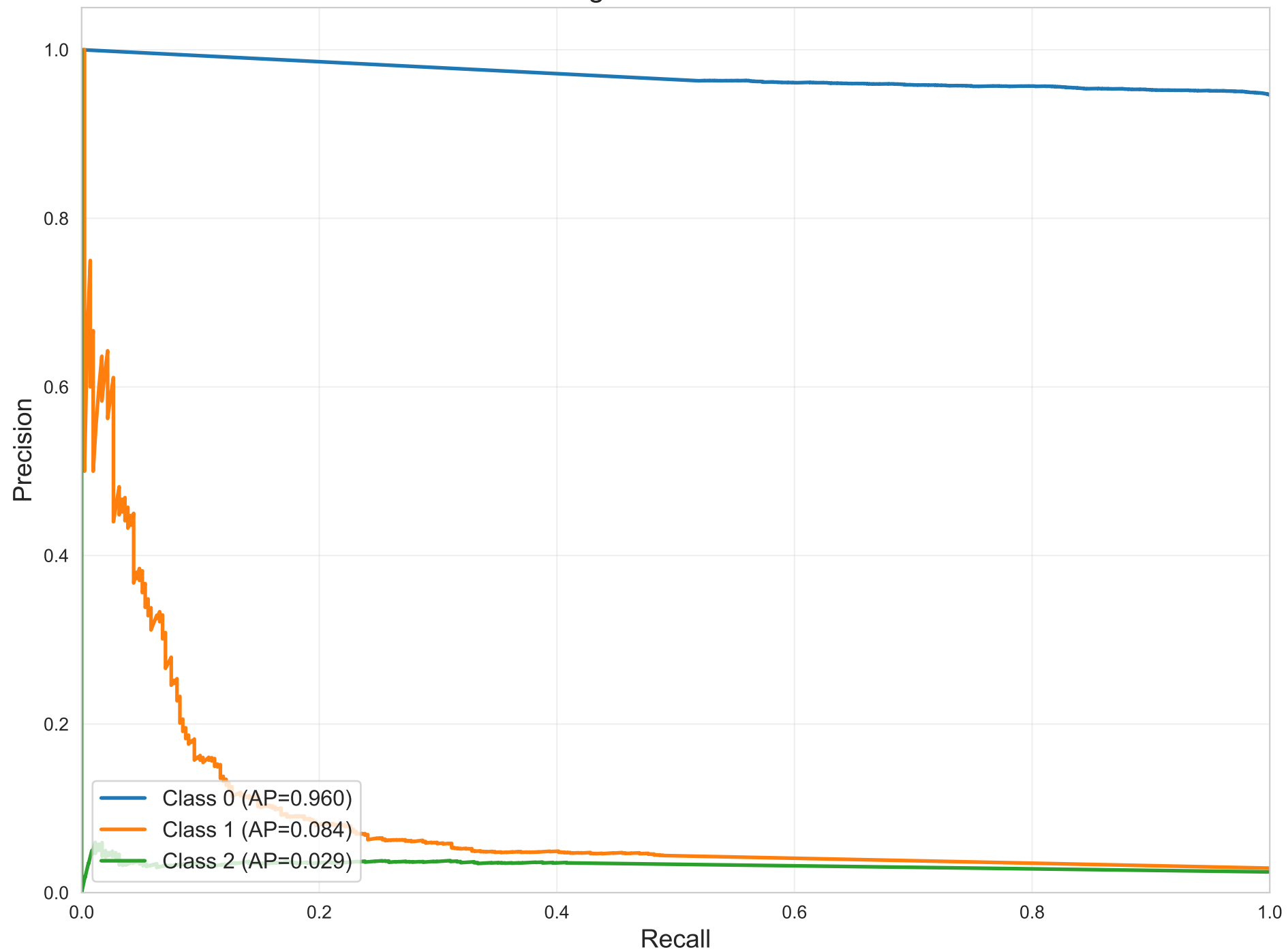
PR Curves per Class - K Nearest Neighbors Weighted AP = 0.912
