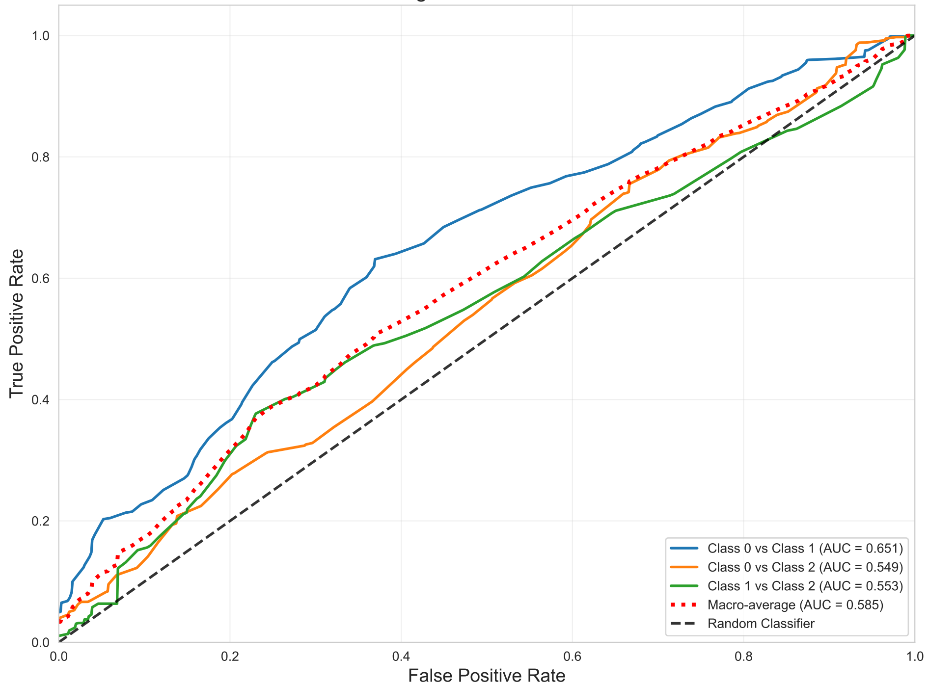
One-vs-One ROC - Random Forest Weighted AUC = 0.593
