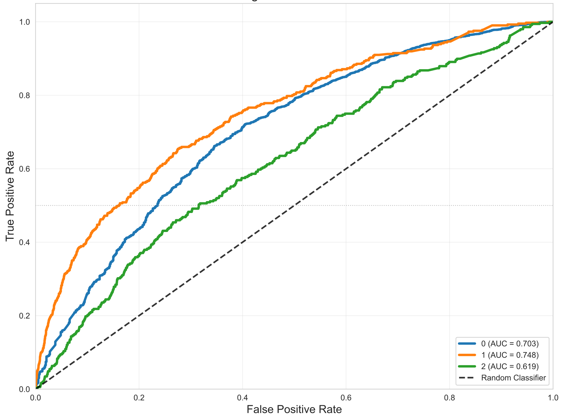
One-vs-Rest ROC - Histogram Gradient Boosting Weighted AUC = 0.702
