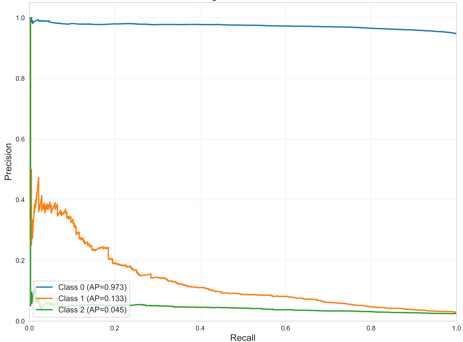
PR Curves per Class - Catboost Weighted AP = 0.926
