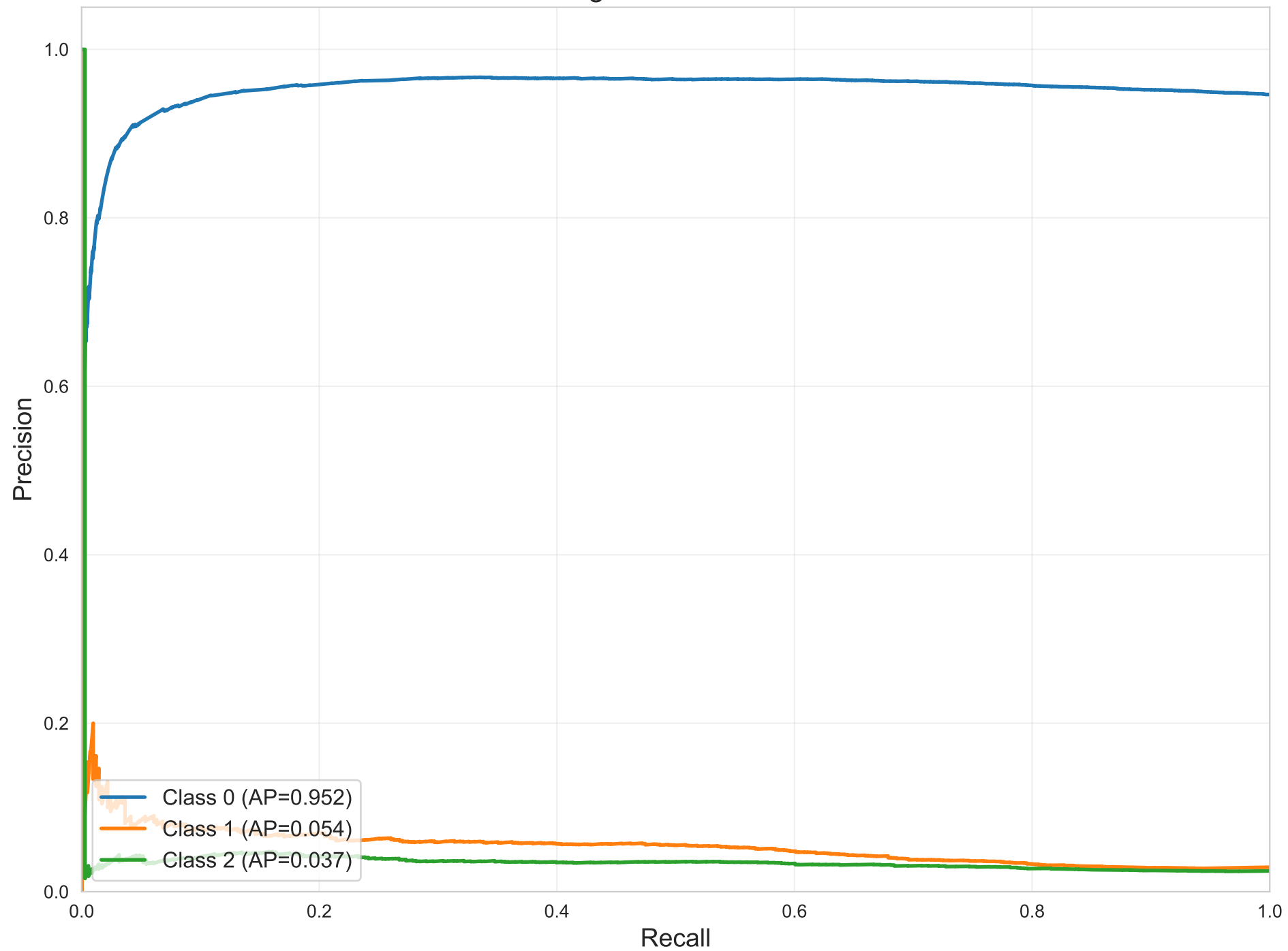
PR Curves per Class - Support Vector Classifier Weighted AP = 0.903
