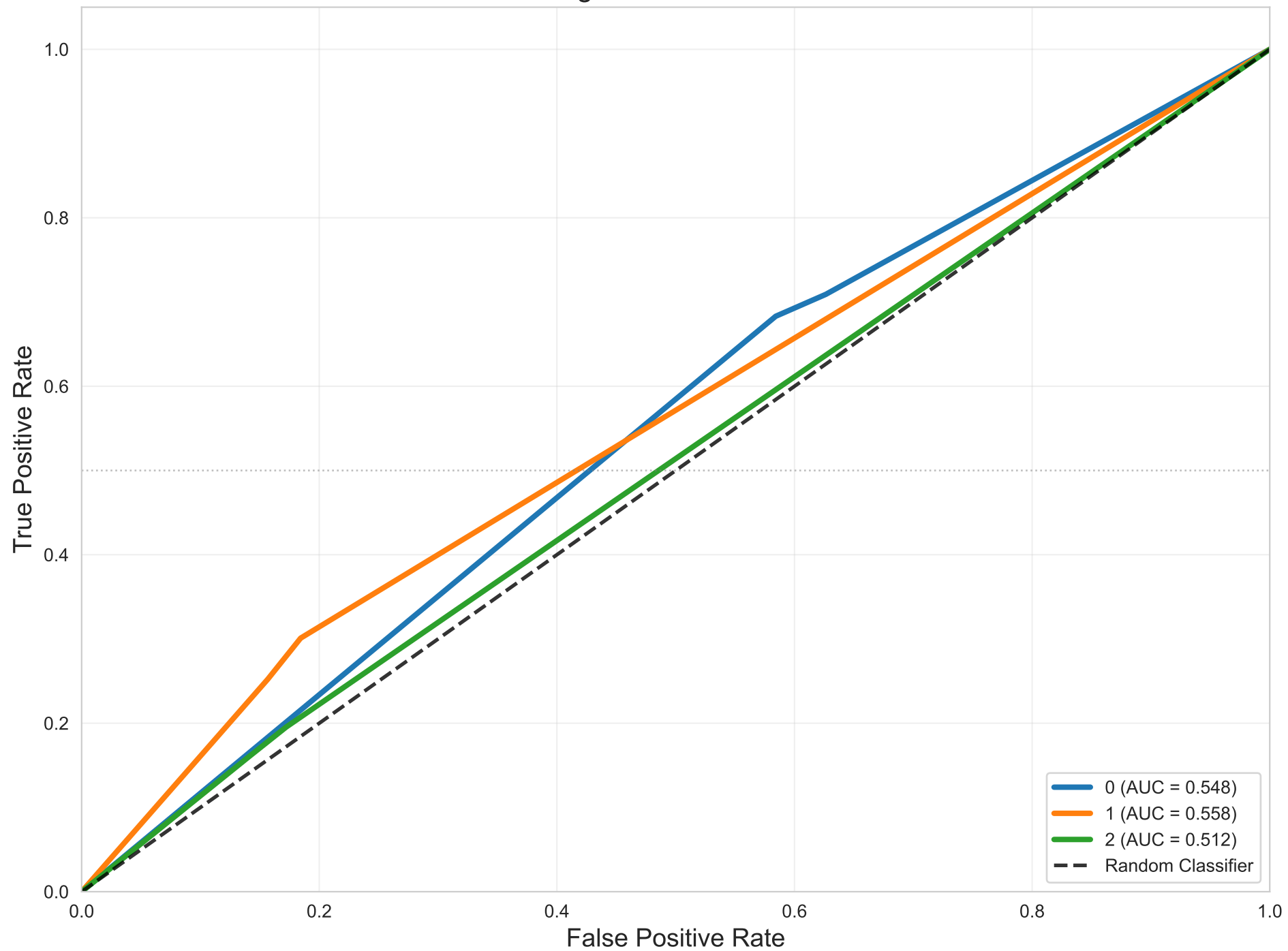
One-vs-Rest ROC - Decision Tree Weighted AUC = 0.544
