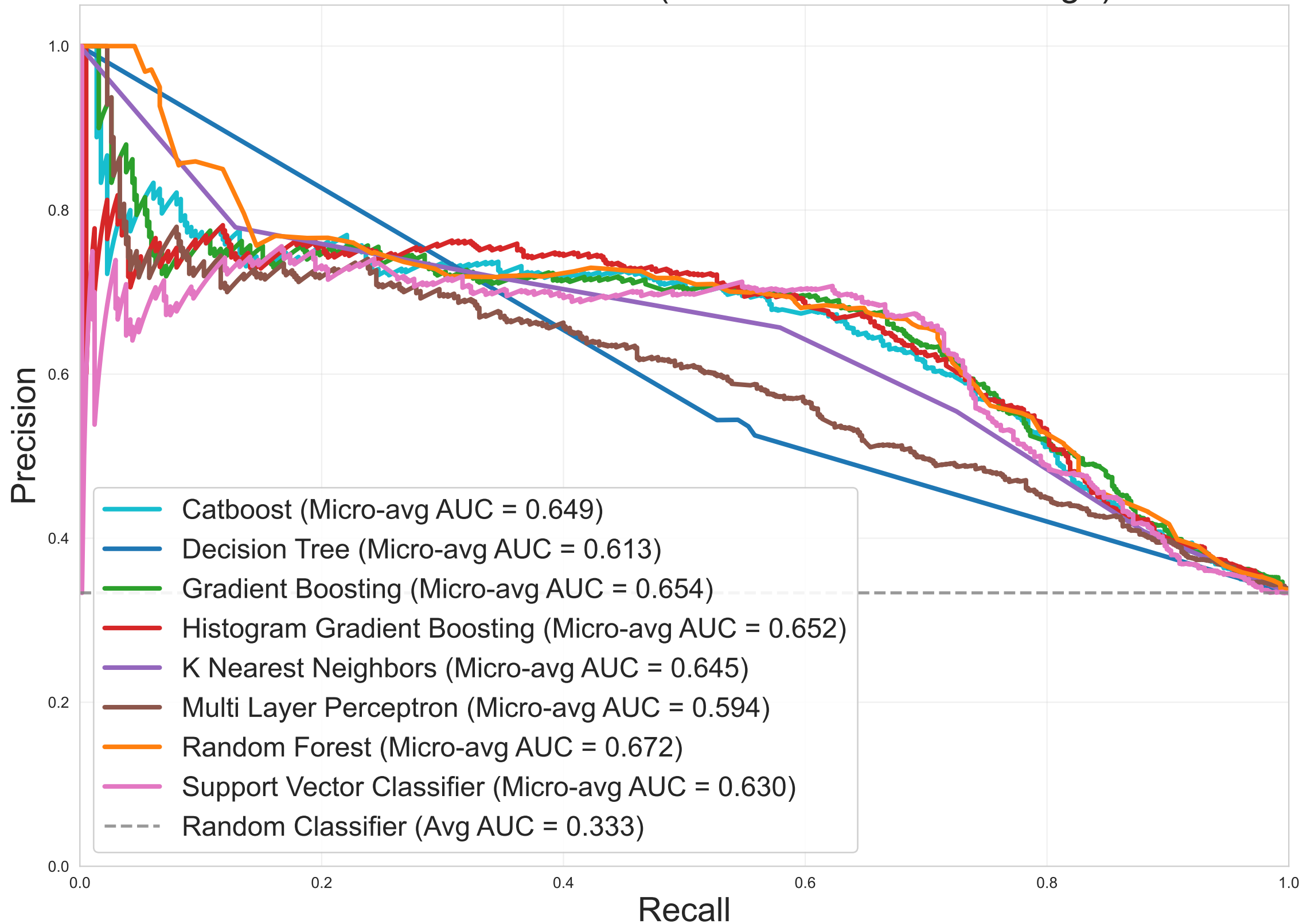
Precision-Recall Curves (Multiclass - Micro-Average)
