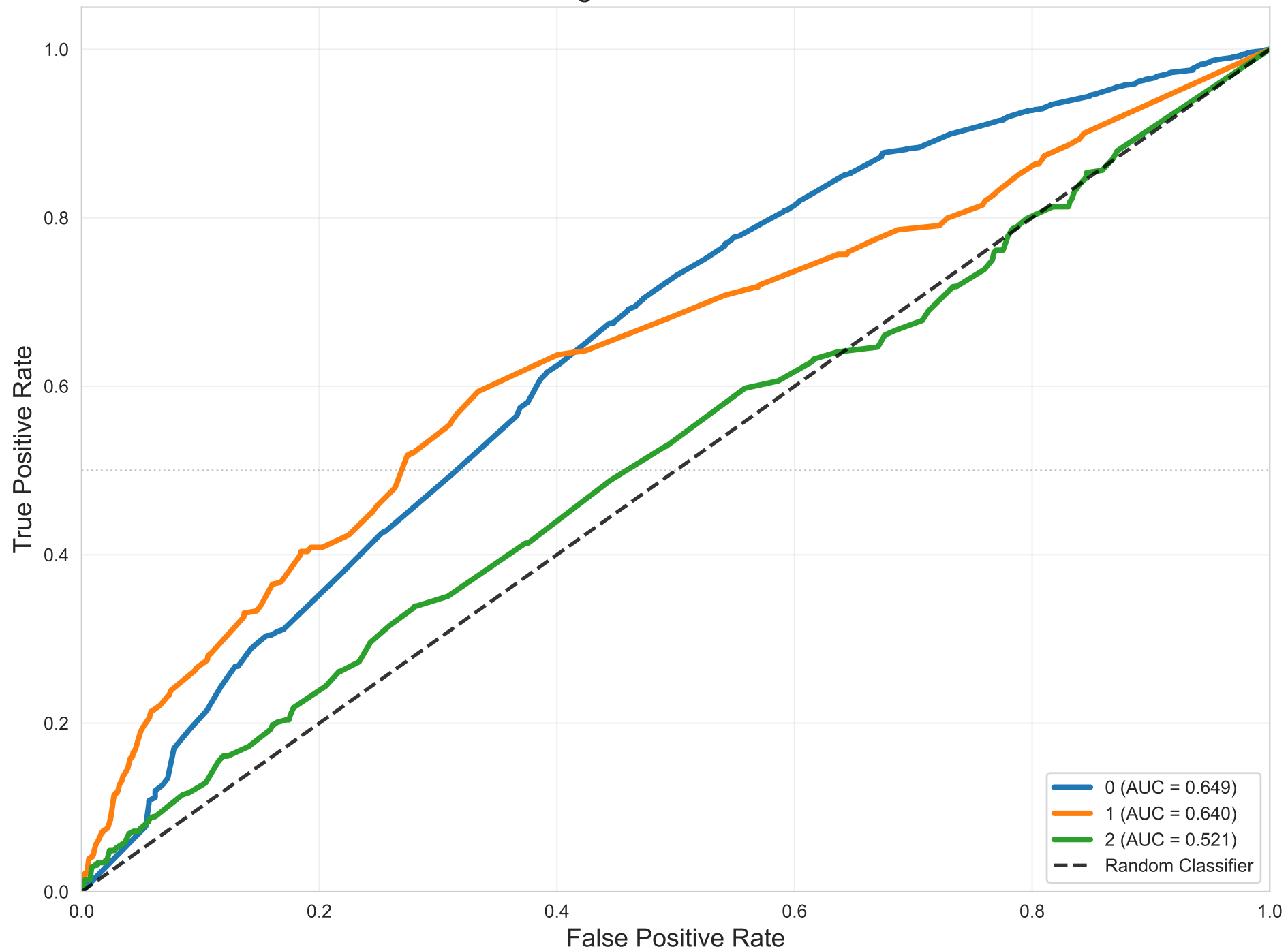
One-vs-Rest ROC - Decision Tree Weighted AUC = 0.646
