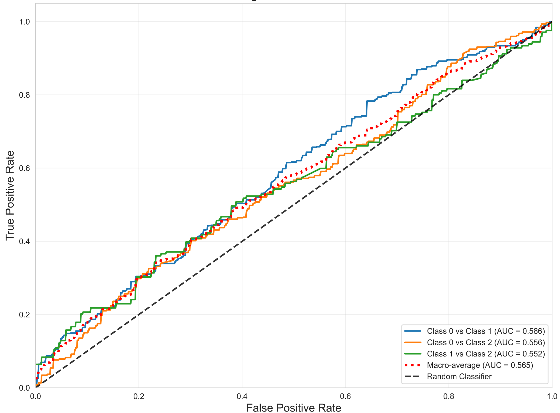
One-vs-One ROC - Support Vector Classifier Weighted AUC = 0.568
