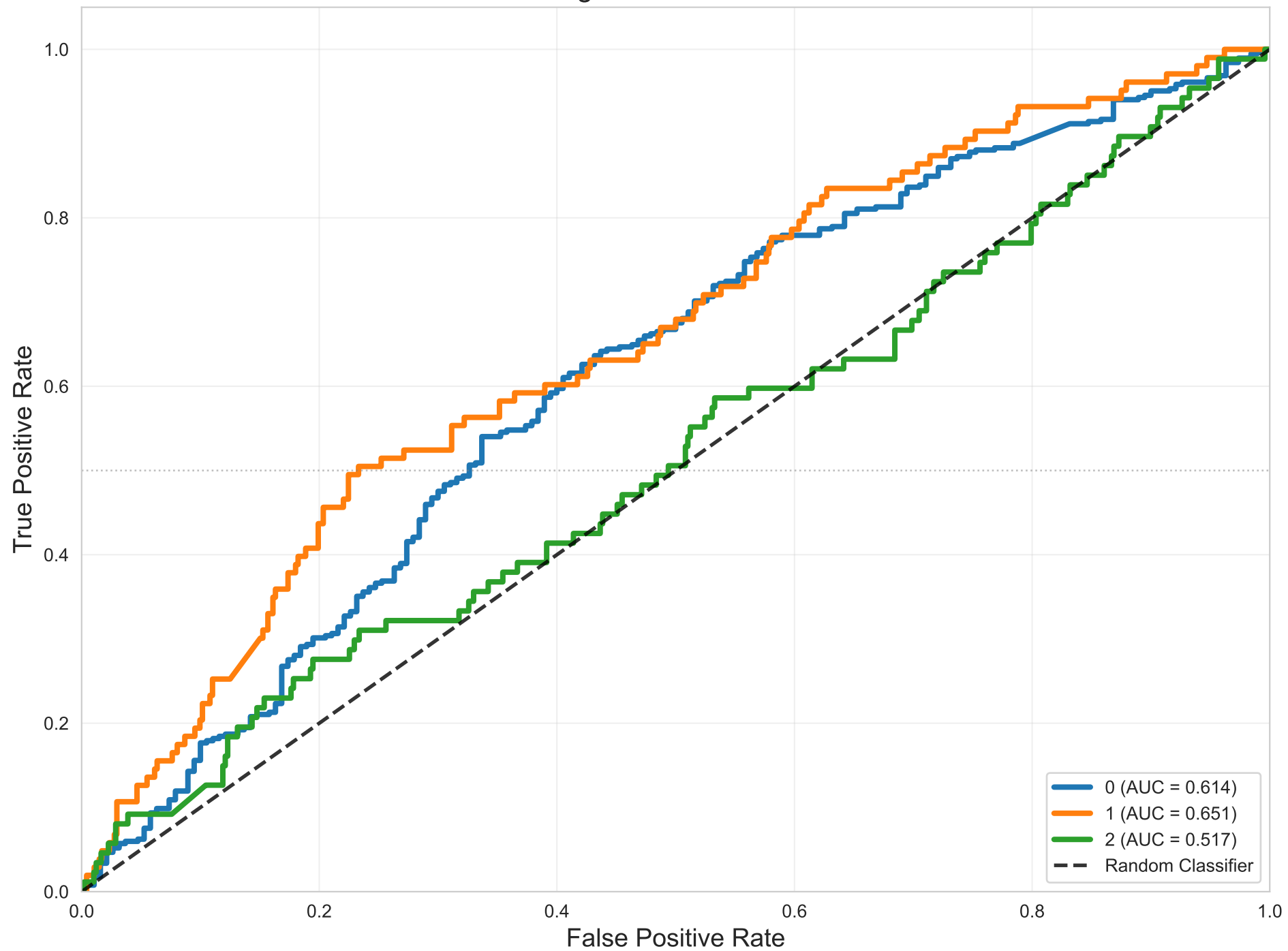
One-vs-Rest ROC - Histogram Gradient Boosting Weighted AUC = 0.606
