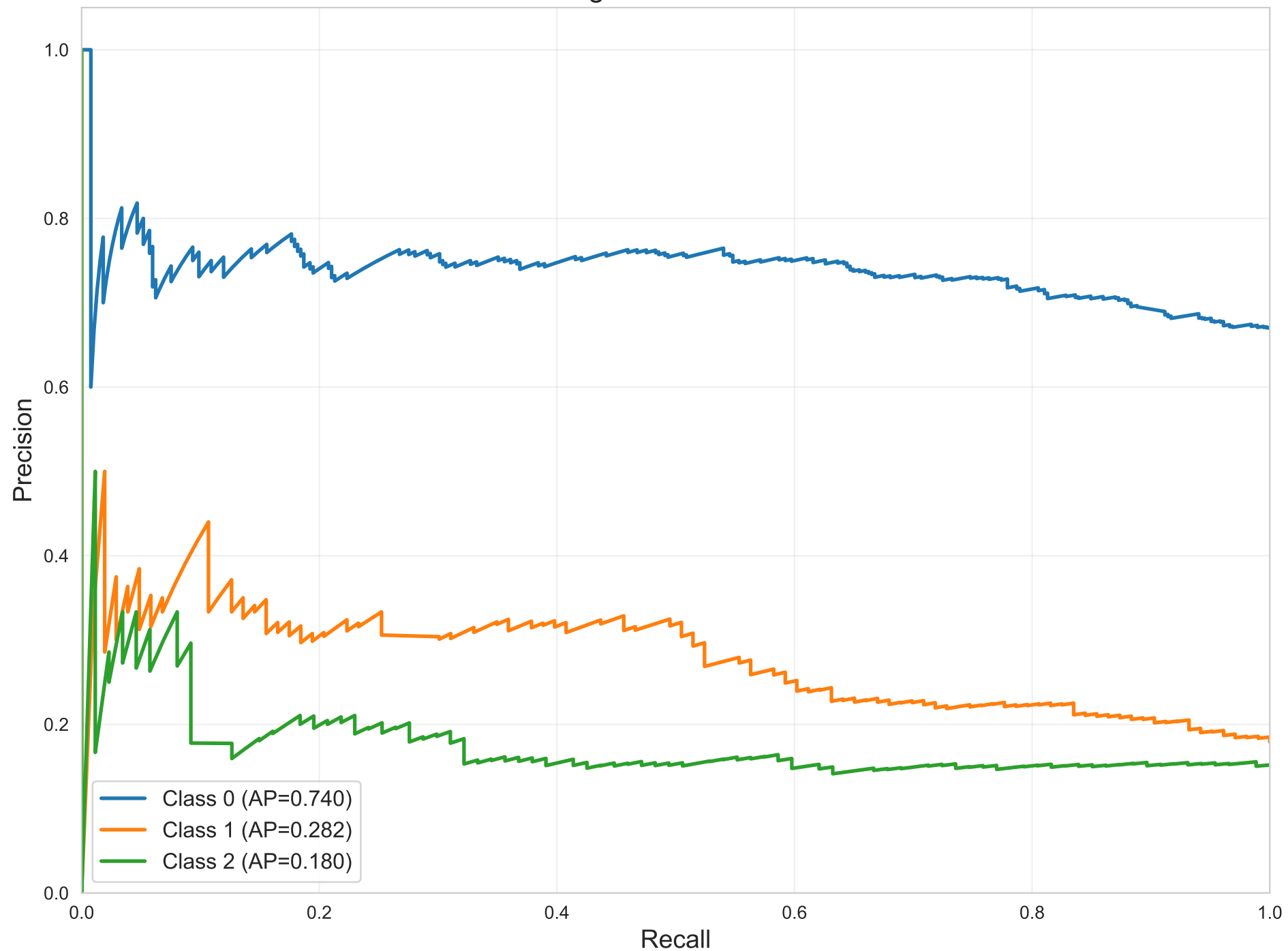
PR Curves per Class - Histogram Gradient Boosting Weighted AP = 0.573
