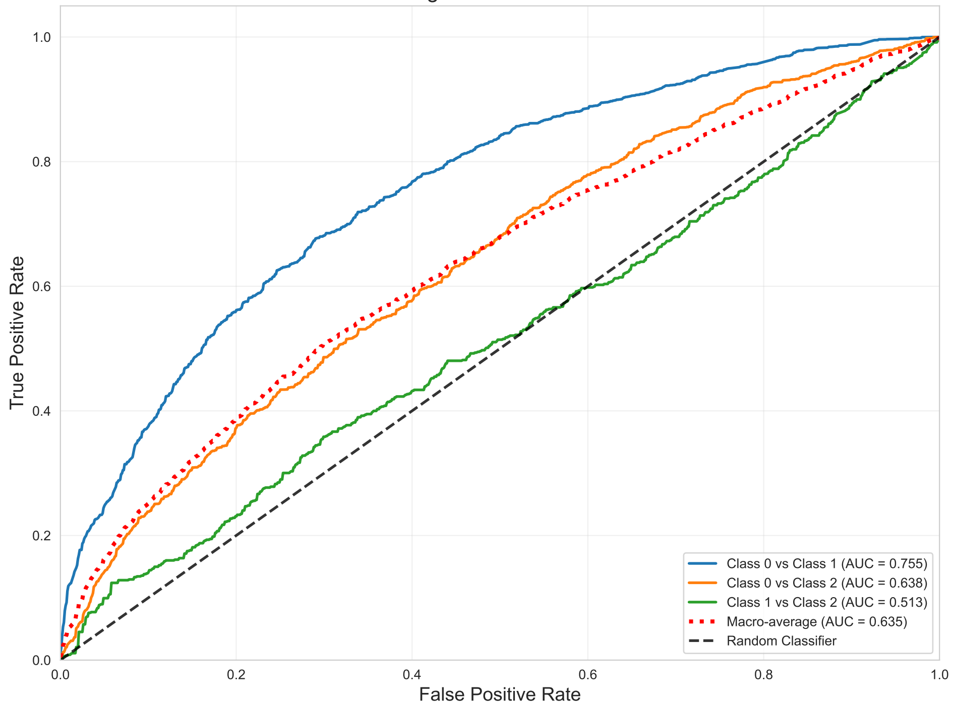
One-vs-One ROC - Gradient Boosting Weighted AUC = 0.692
