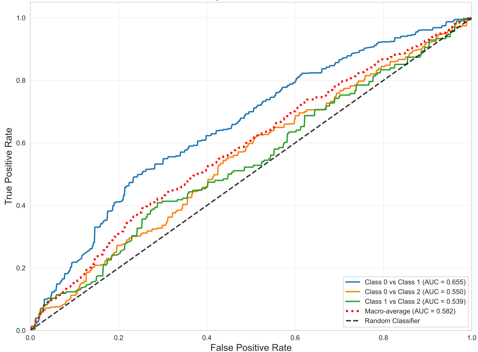
One-vs-One ROC - Histogram Gradient Boosting Weighted AUC = 0.593
