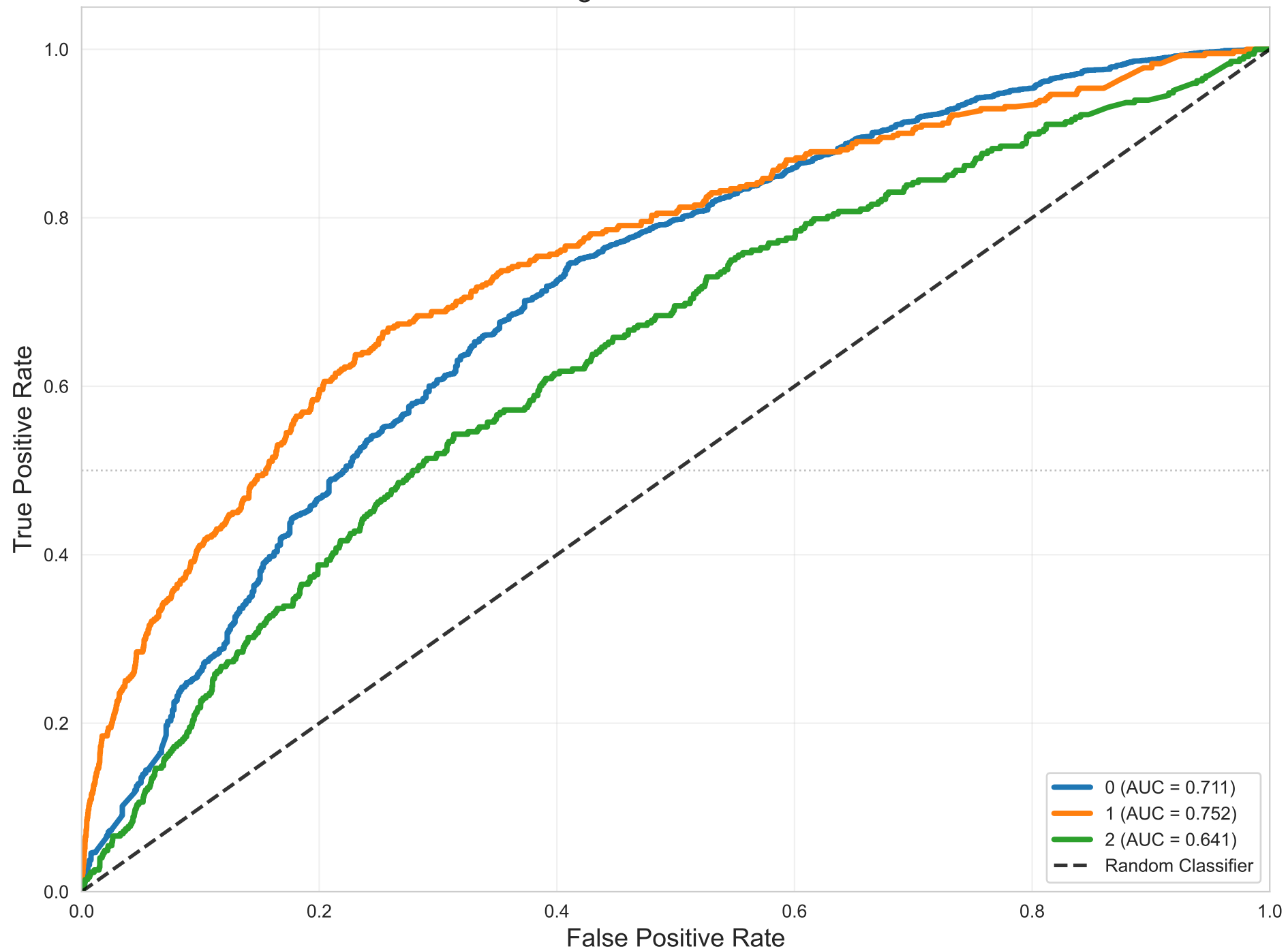
One-vs-Rest ROC - Catboost Weighted AUC = 0.710
