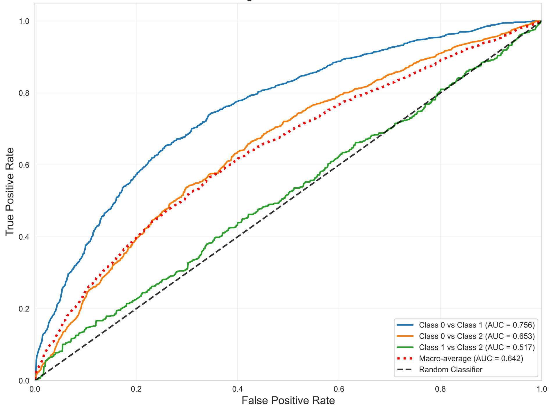
One-vs-One ROC - Catboost Weighted AUC = 0.699
