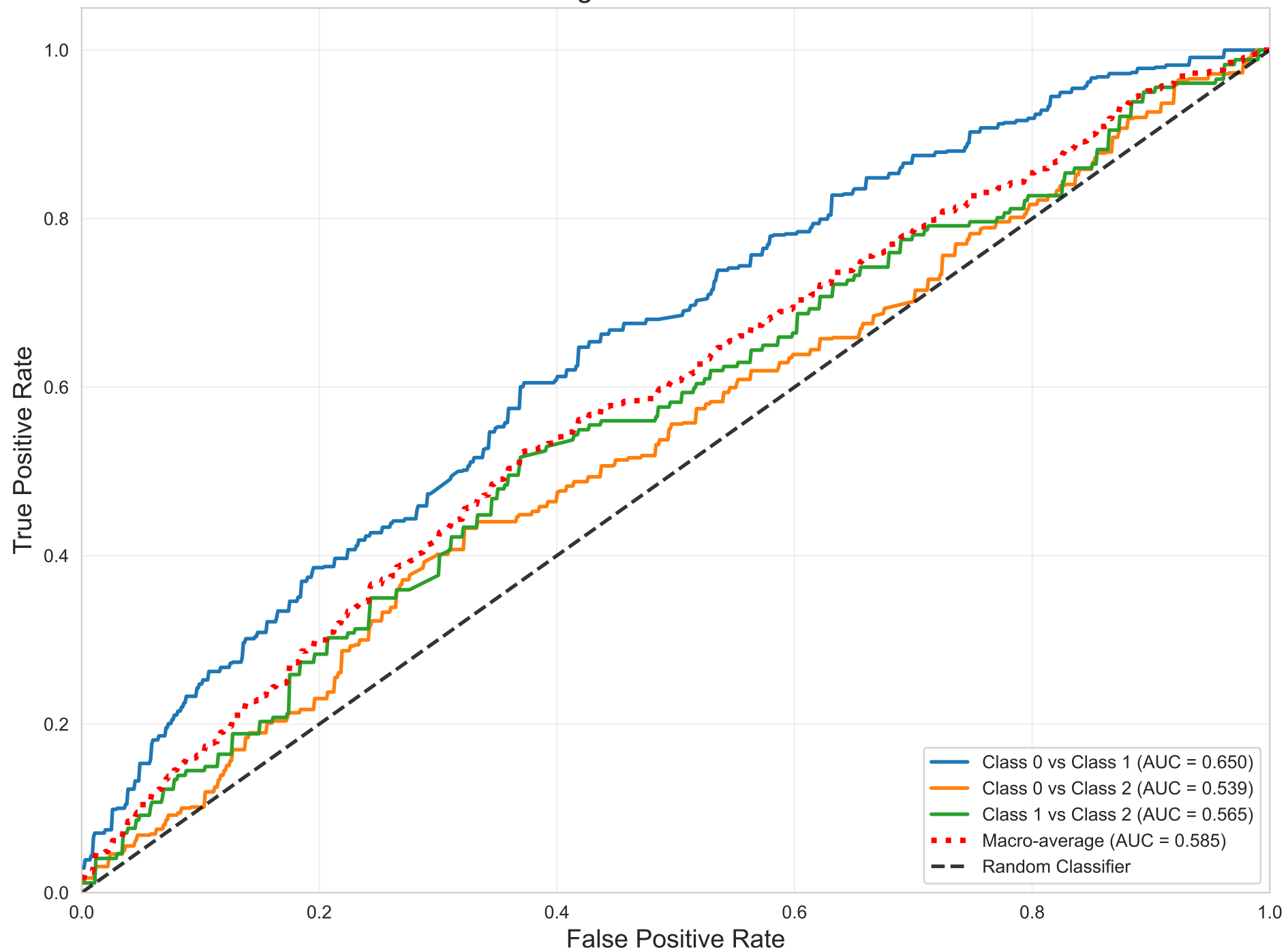
One-vs-One ROC - Gradient Boosting Weighted AUC = 0.590
