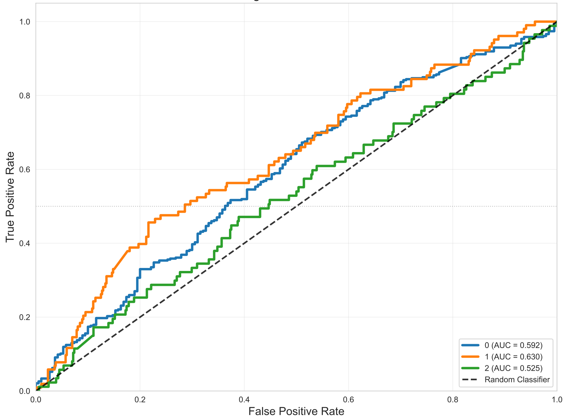
One-vs-Rest ROC - Catboost Weighted AUC = 0.589
