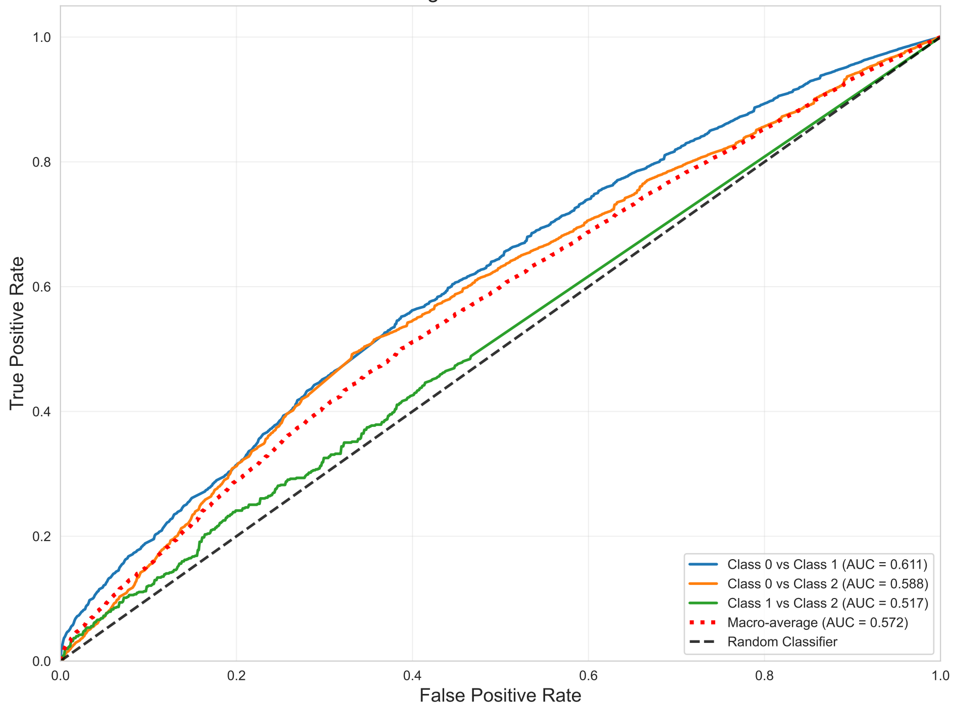
One-vs-One ROC - K Nearest Neighbors Weighted AUC = 0.597
