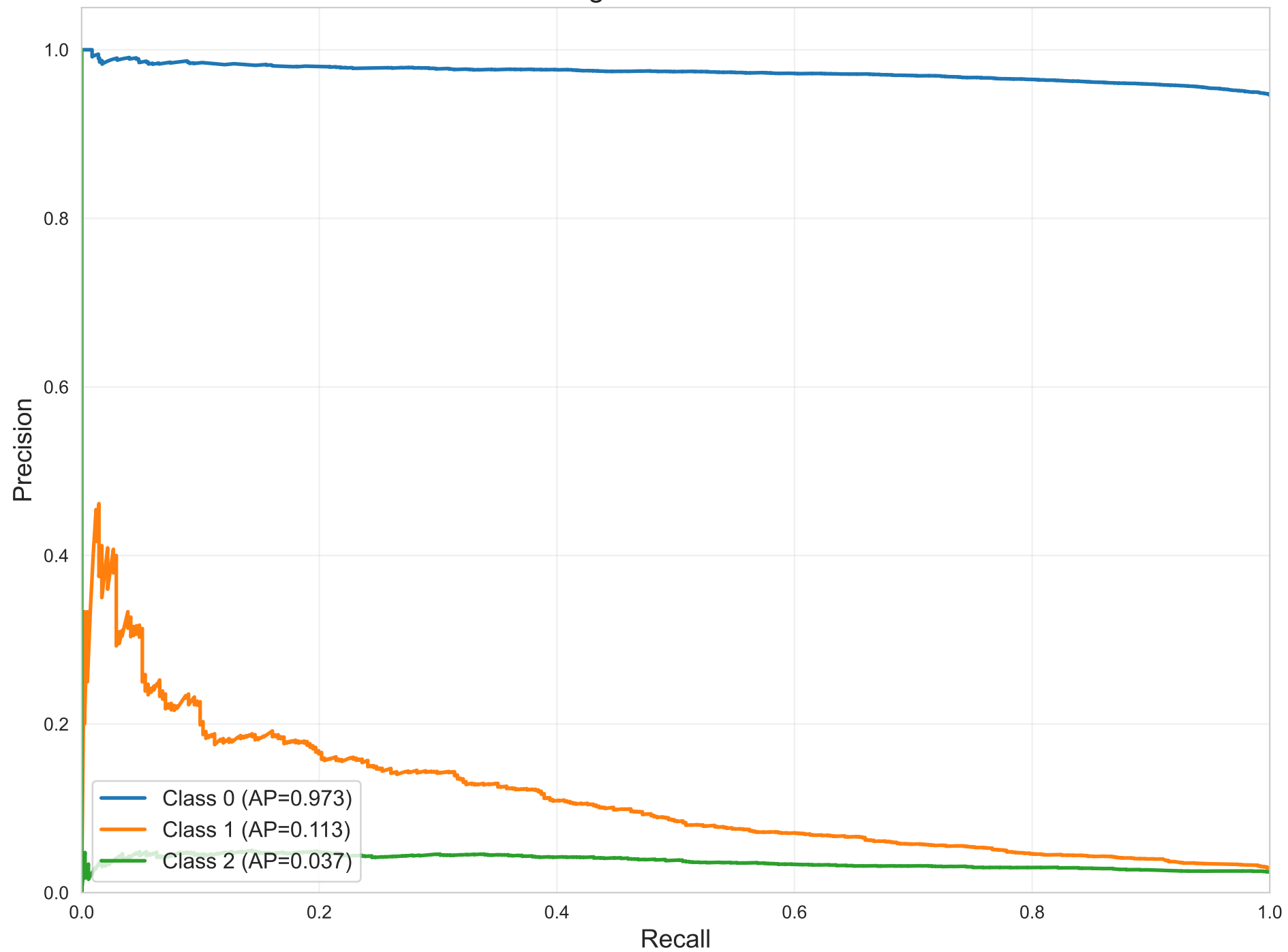
PR Curves per Class - Histogram Gradient Boosting Weighted AP = 0.925
