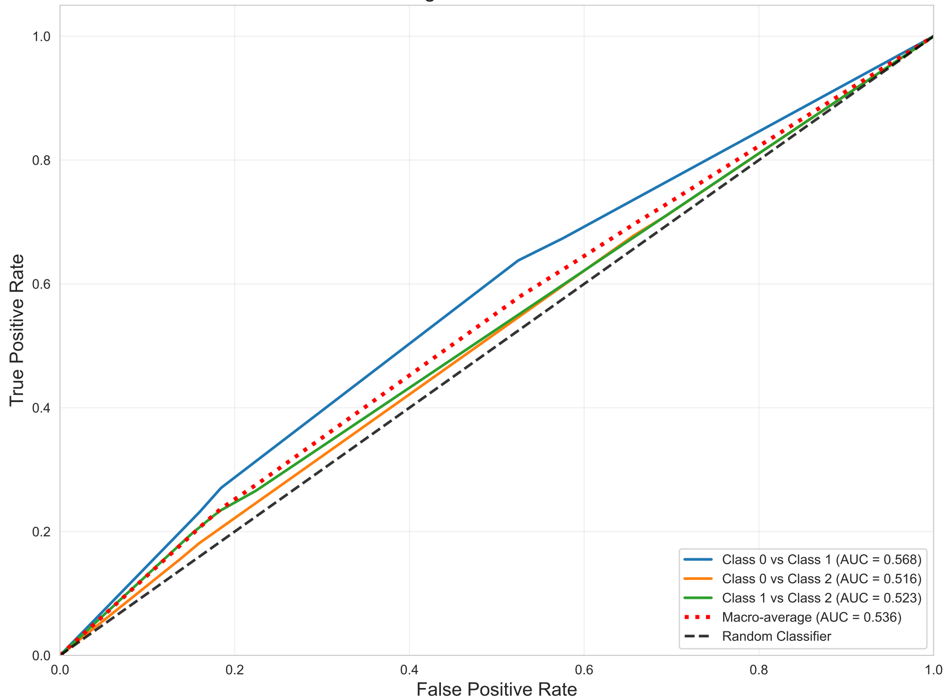
One-vs-One ROC - Decision Tree Weighted AUC = 0.539
