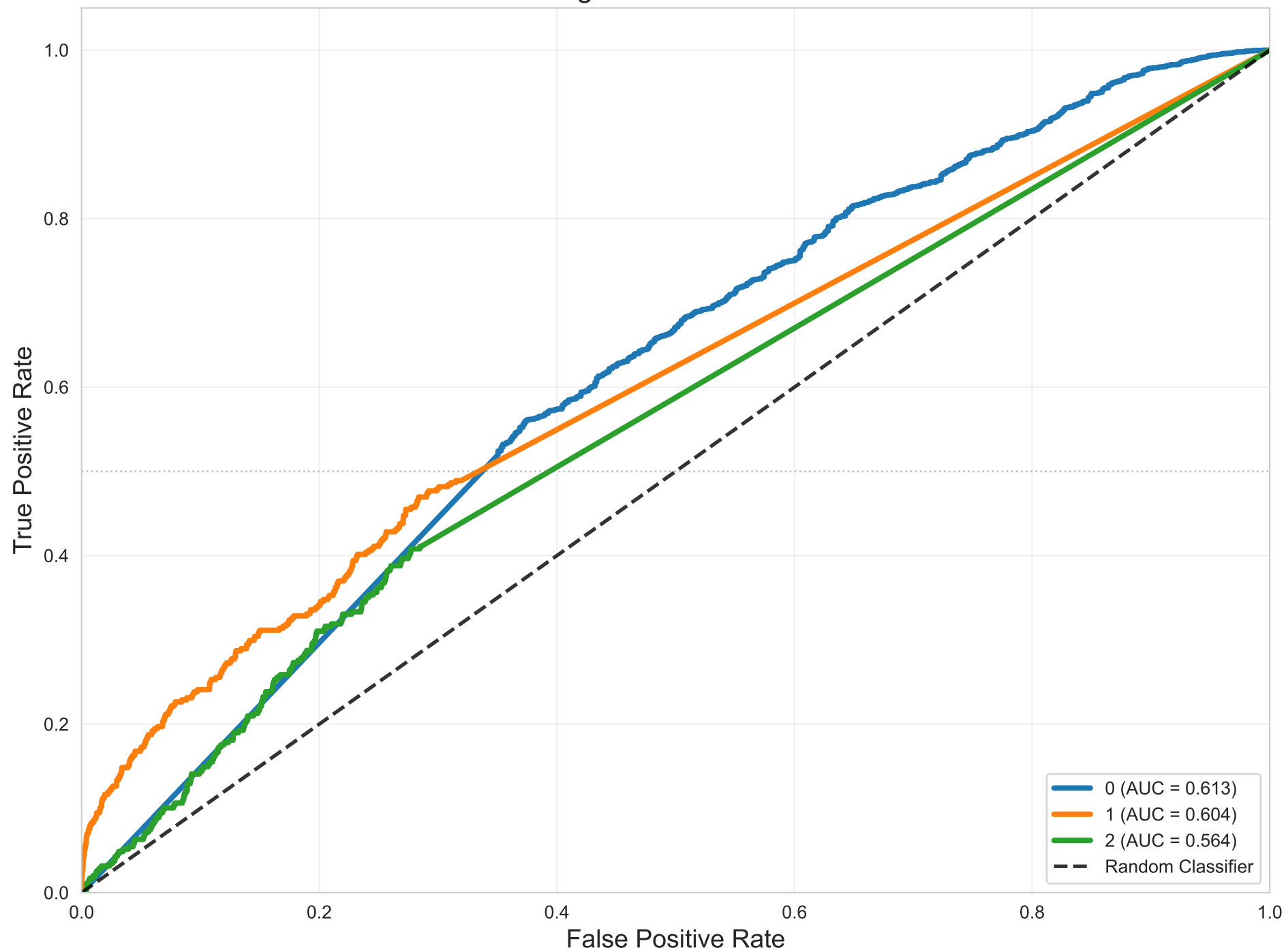
One-vs-Rest ROC - K Nearest Neighbors Weighted AUC = 0.612
