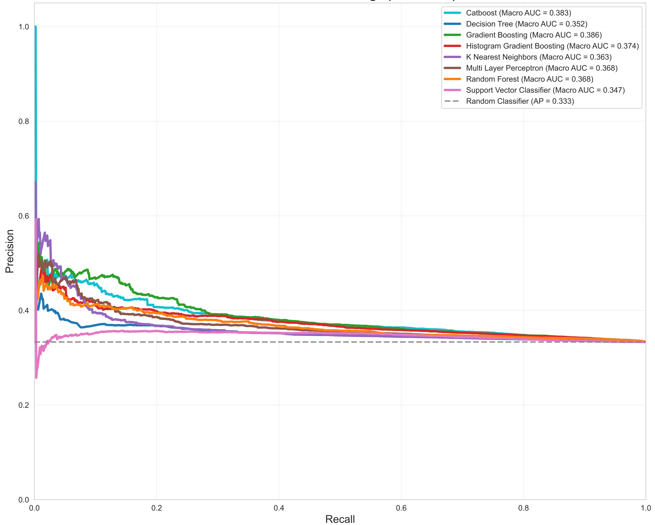
PR Curves - Macro Average (All Models)
