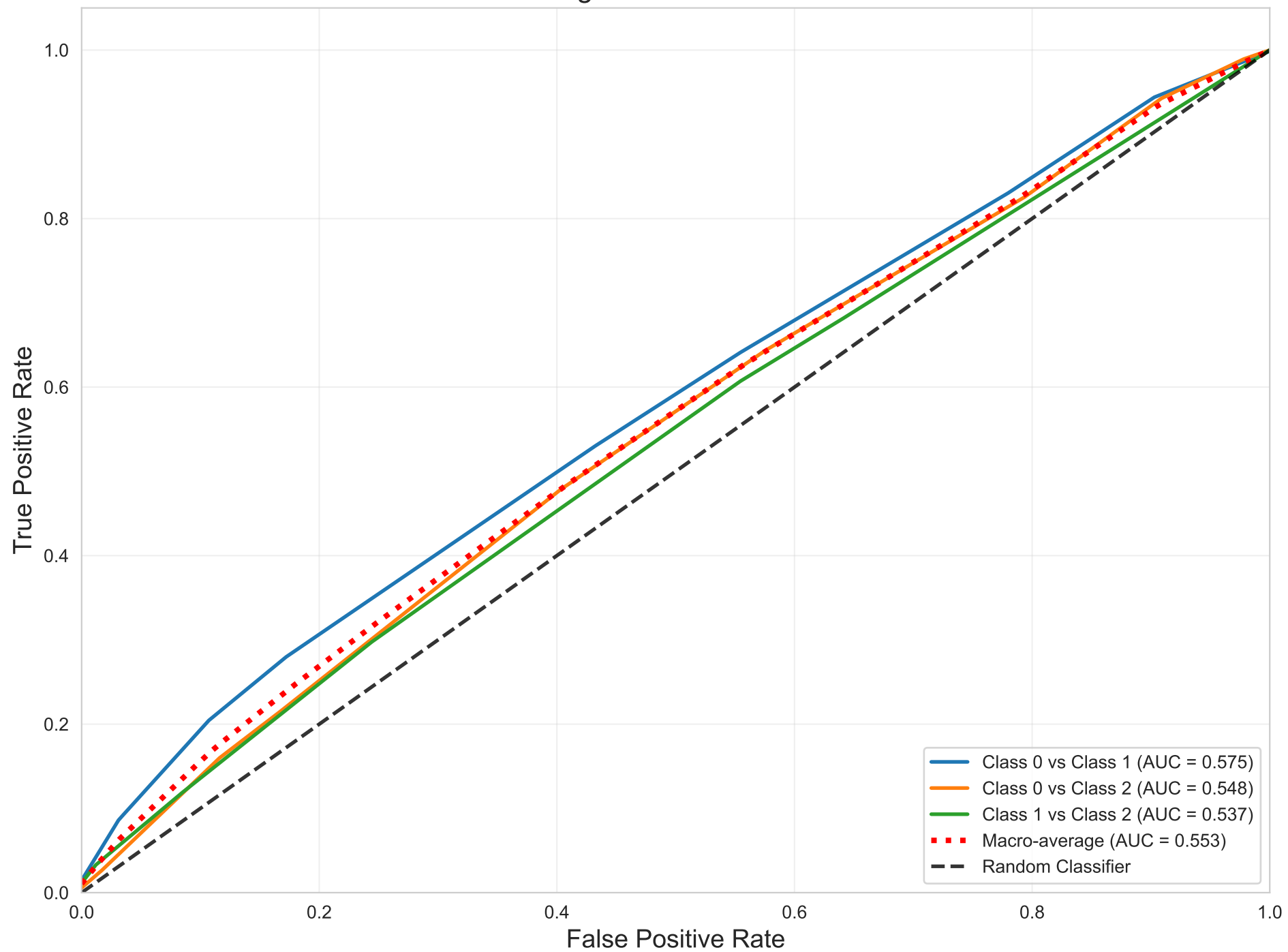
One-vs-One ROC - K Nearest Neighbors Weighted AUC = 0.558
