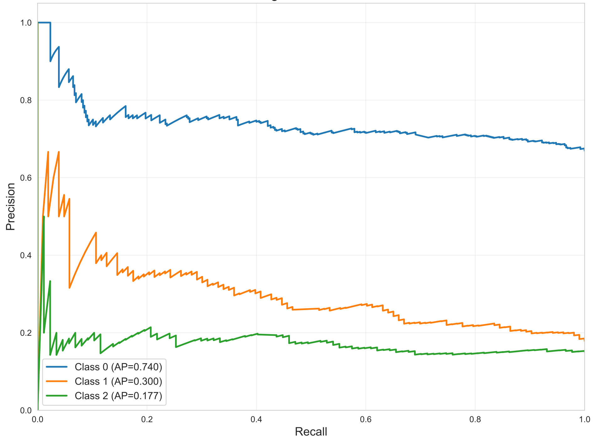
PR Curves per Class - Gradient Boosting Weighted AP = 0.576
