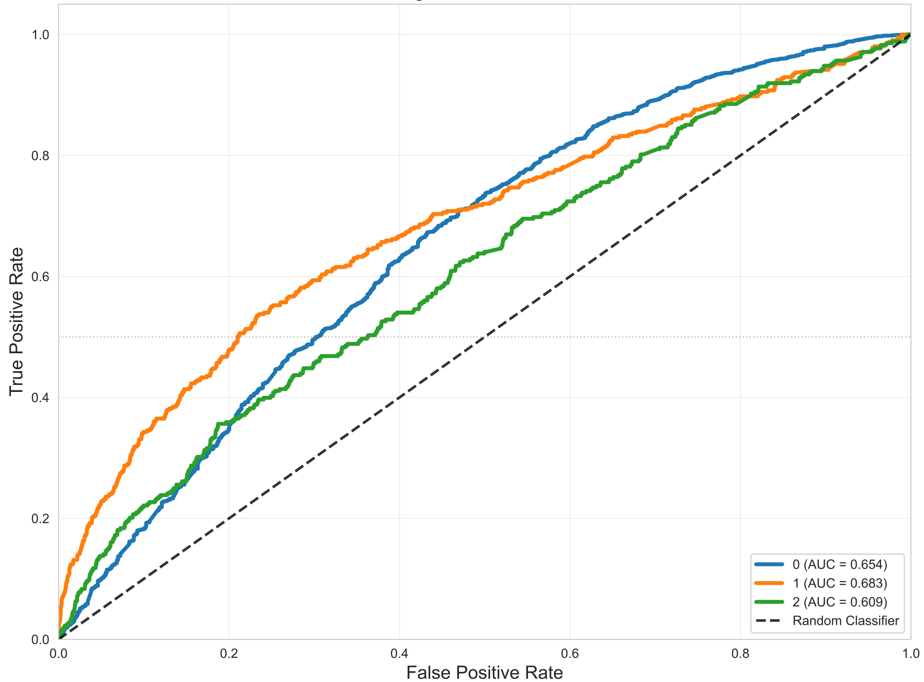
One-vs-Rest ROC - Multi Layer Perceptron Weighted AUC = 0.654
