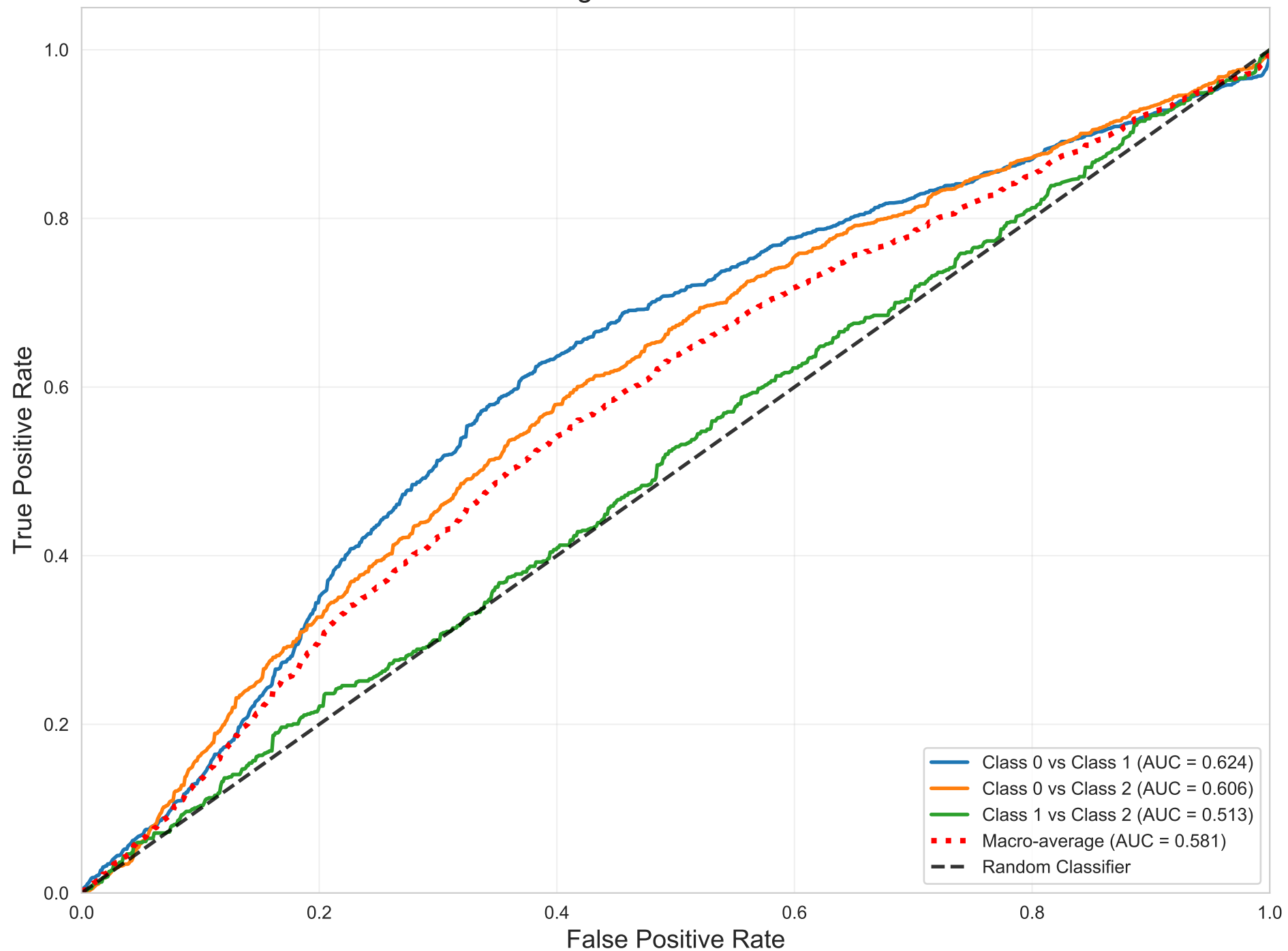
One-vs-One ROC - Support Vector Classifier Weighted AUC = 0.612
