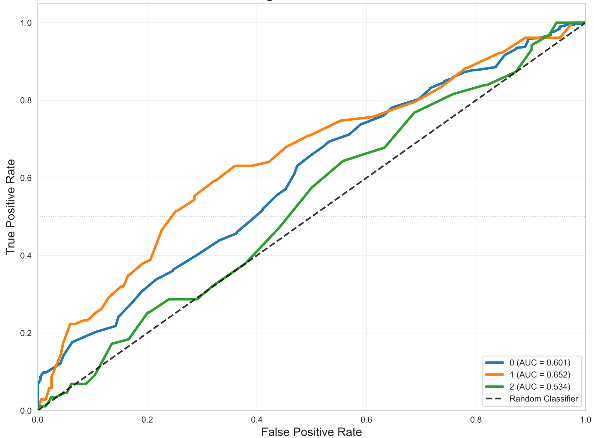
One-vs-Rest ROC - Random Forest Weighted AUC = 0.600
