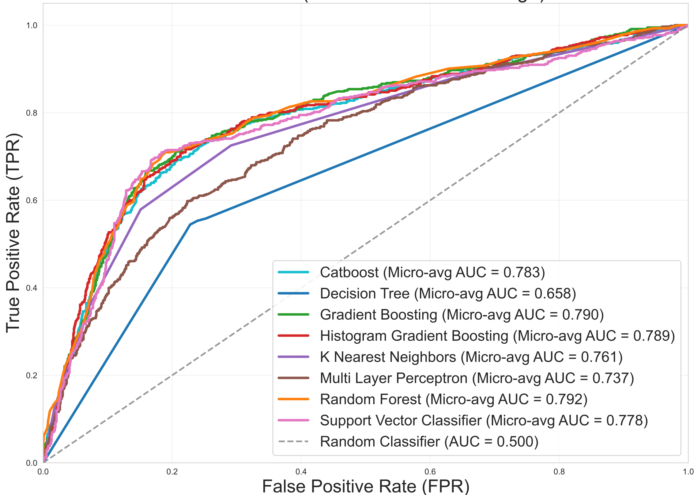
ROC Curves (Multiclass - Micro-Average)
