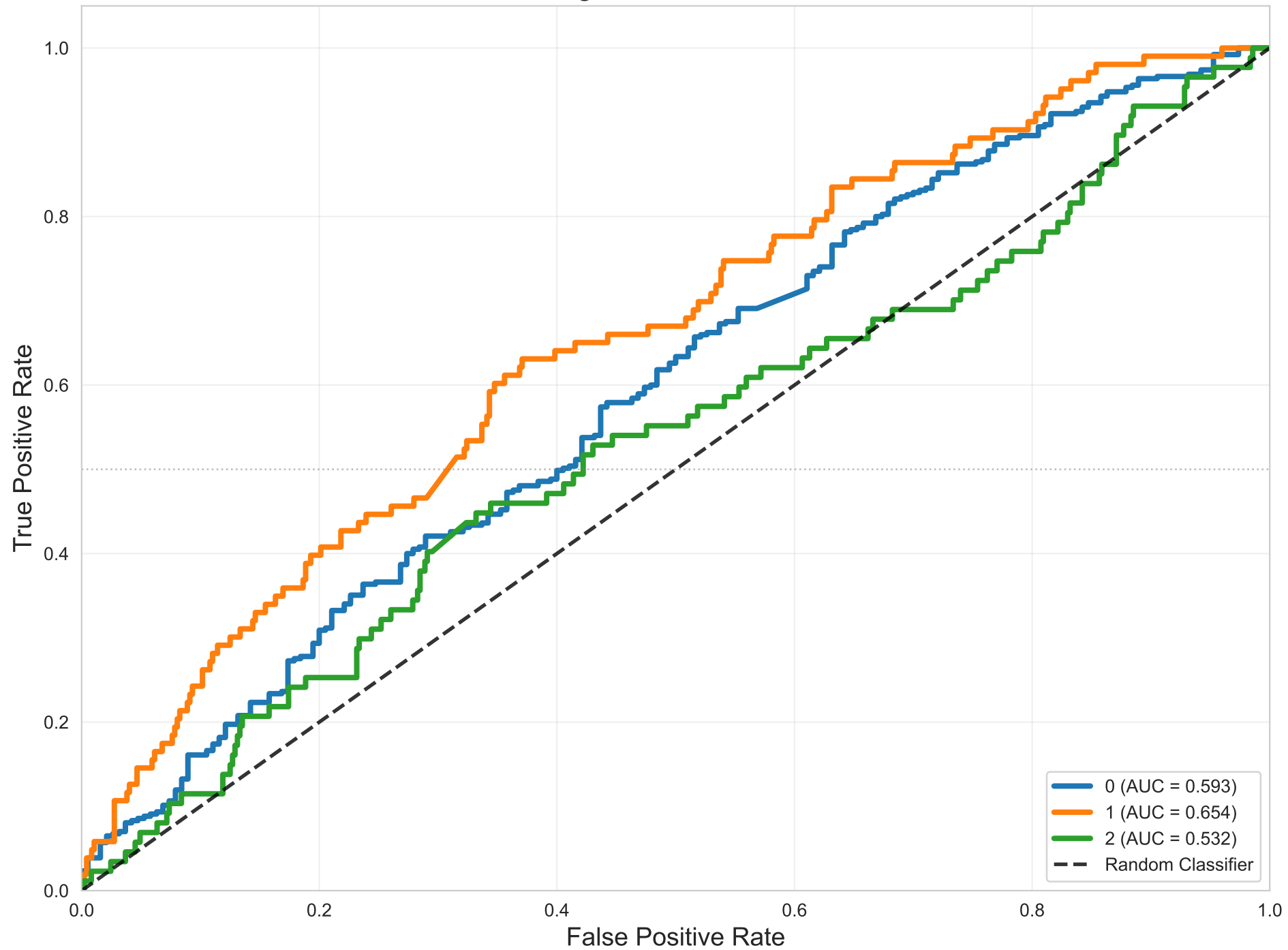
One-vs-Rest ROC - Gradient Boosting Weighted AUC = 0.595
