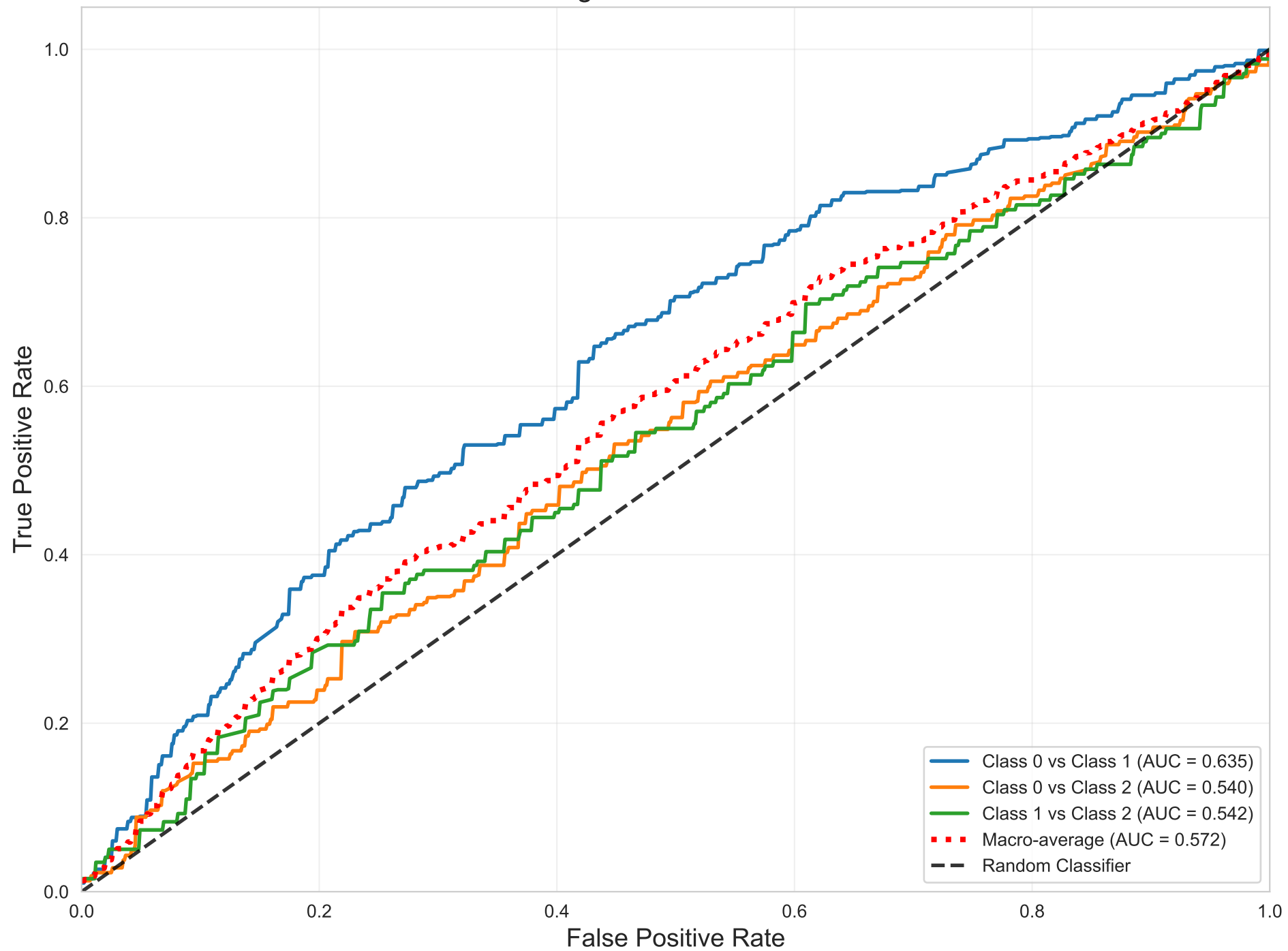
One-vs-One ROC - Catboost Weighted AUC = 0.580
