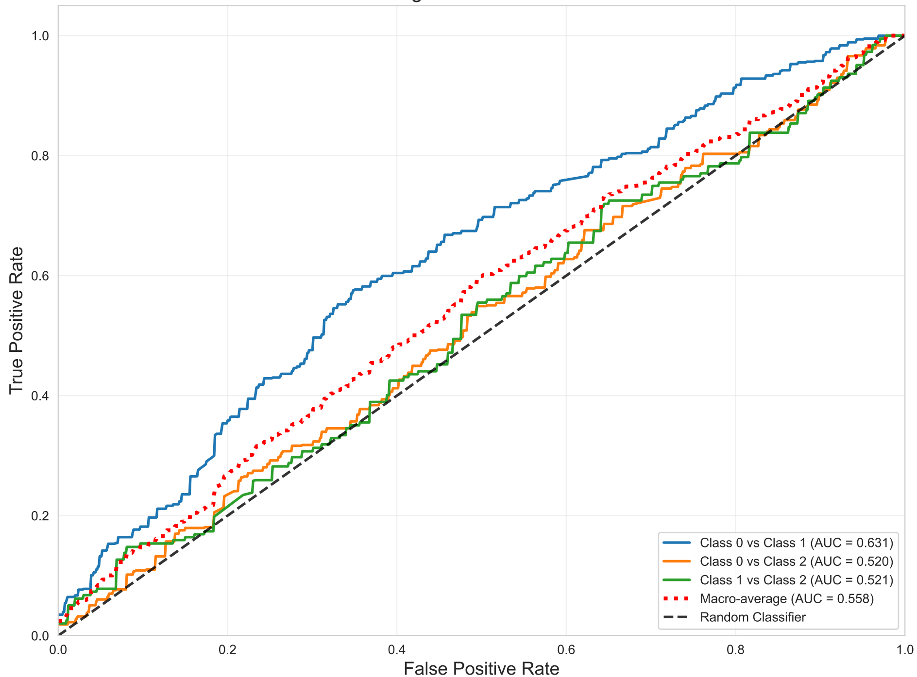
One-vs-One ROC - Multi Layer Perceptron Weighted AUC = 0.567
