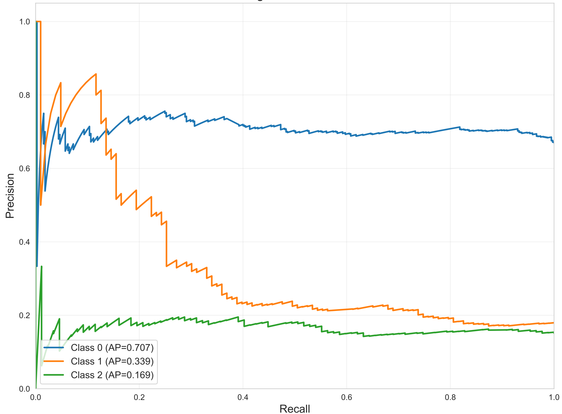
PR Curves per Class - Support Vector Classifier Weighted AP = 0.560
