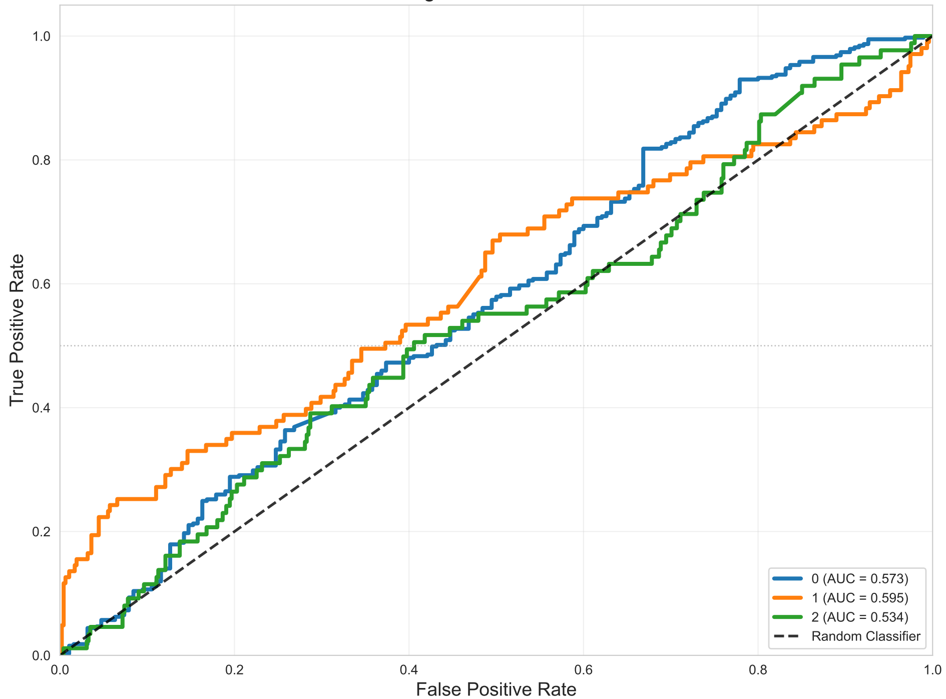
One-vs-Rest ROC - Support Vector Classifier Weighted AUC = 0.571
